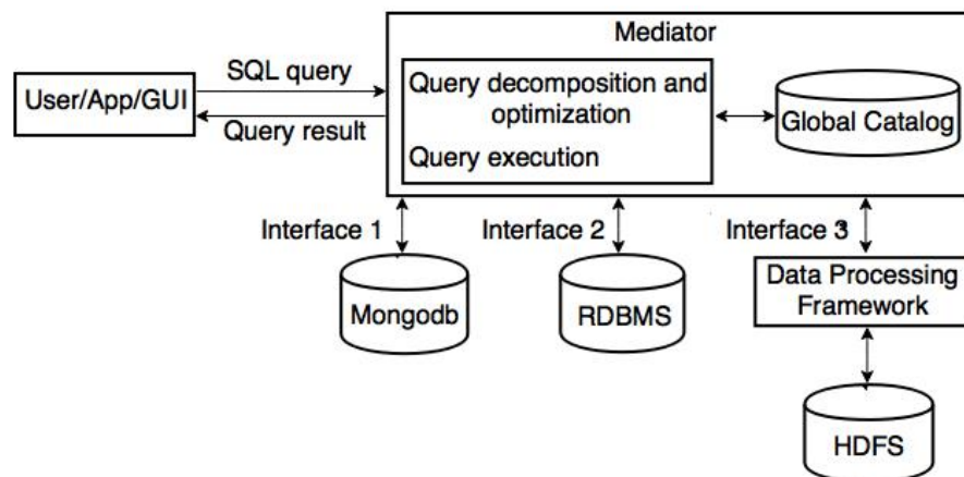
Figure 2.9 – Tightly-coupled multistore systems
