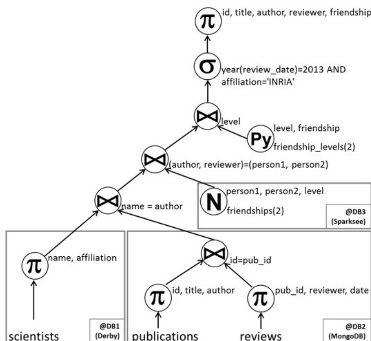
Figure 3.3 – Preliminary execution plan
