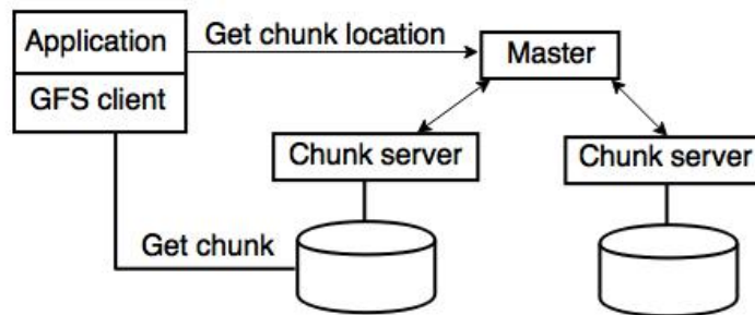
Figure 2.2 – GFS architecture
