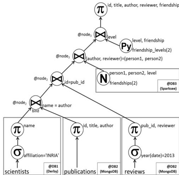
Figure 3.4 – Optimized execution plan
