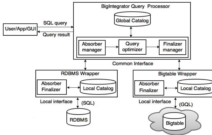
Figure 2.8 – BigIntegrator
