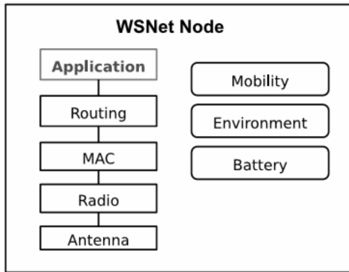
Fig. 5.4 Modular Architecture of a WSN Node.
