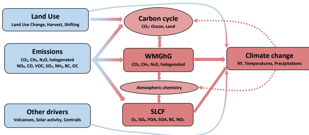
Figure 1.1: Schematic description of the reduced-form Earth system model OSCAR v2.2. The full description of the model can be found in Gasser et al. (2017a).
