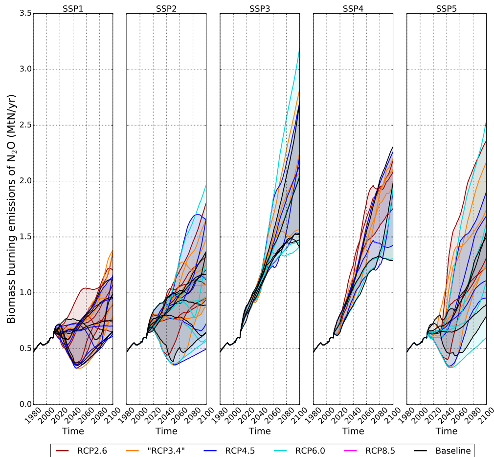
Figure 6.28: Change in N_2O emissions from biomass burning since the preindustrial equilibrium from 1980 to 2100 (section 3.3.1.4). The transition from the historic period and the scenario happens in 2010. Each subfigure details the results for a given SSP. The scenarios are also classified depending on the climate target. Each line represents an IAM that has run this SSP and this climate target, and in plain color is their ensemble. For the sake of clarity, uncertainties are not represented here.
