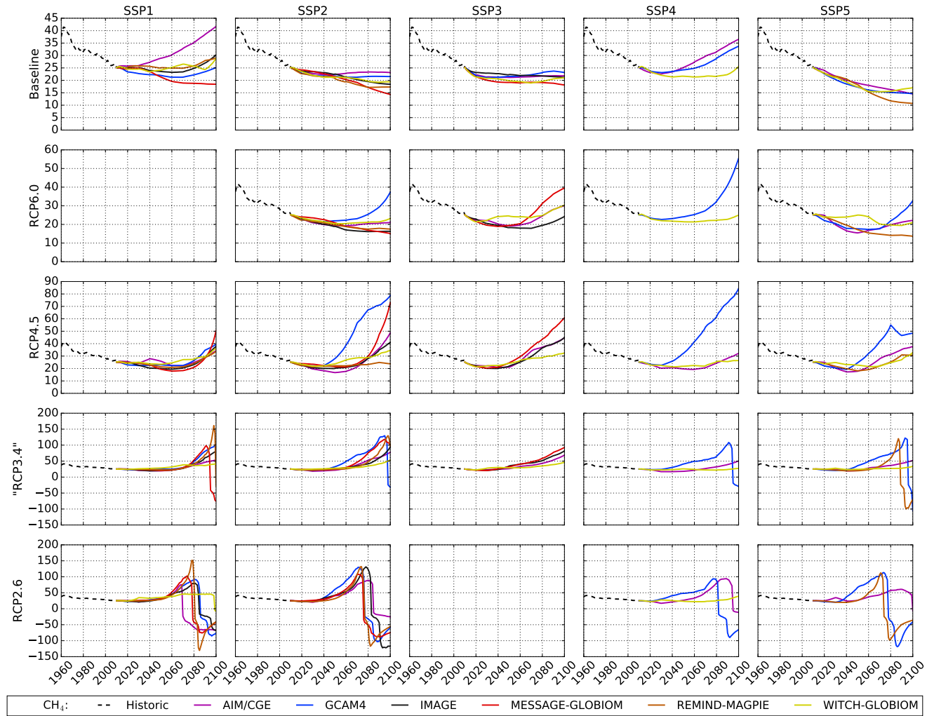
Figure 6.33: Co-emissions ratios for CH_4 (TgC/GtC), for extension of the Kaya decomposition in section 3.3.7. For the sake of clarity, uncertainties are not represented for the ratios.
