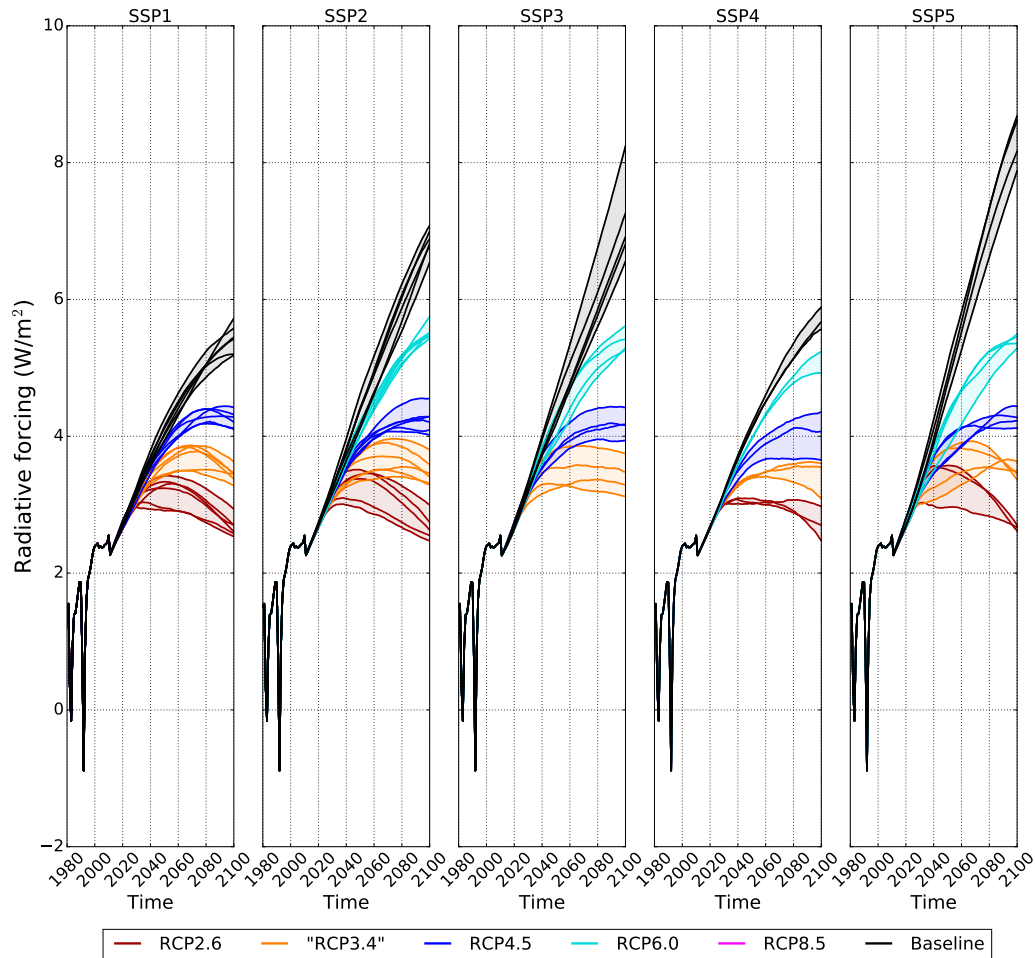
Figure 3.18: Radiative forcing ( \text{W}/\text{m}^2 ). Each subfigure details the results for a given SSP. The scenarios are also classified depending on the forcing target. Each plain line represents an IAM that has run this SSP and this forcing target. For comparison, the radiative forcing of 2011 with reference to 1750 is estimated at 2.3 \text{ W}/\text{m}^2 (Myhre et al., 2013). For the sake of clarity, uncertainties on SSP climate projections are not represented here.
