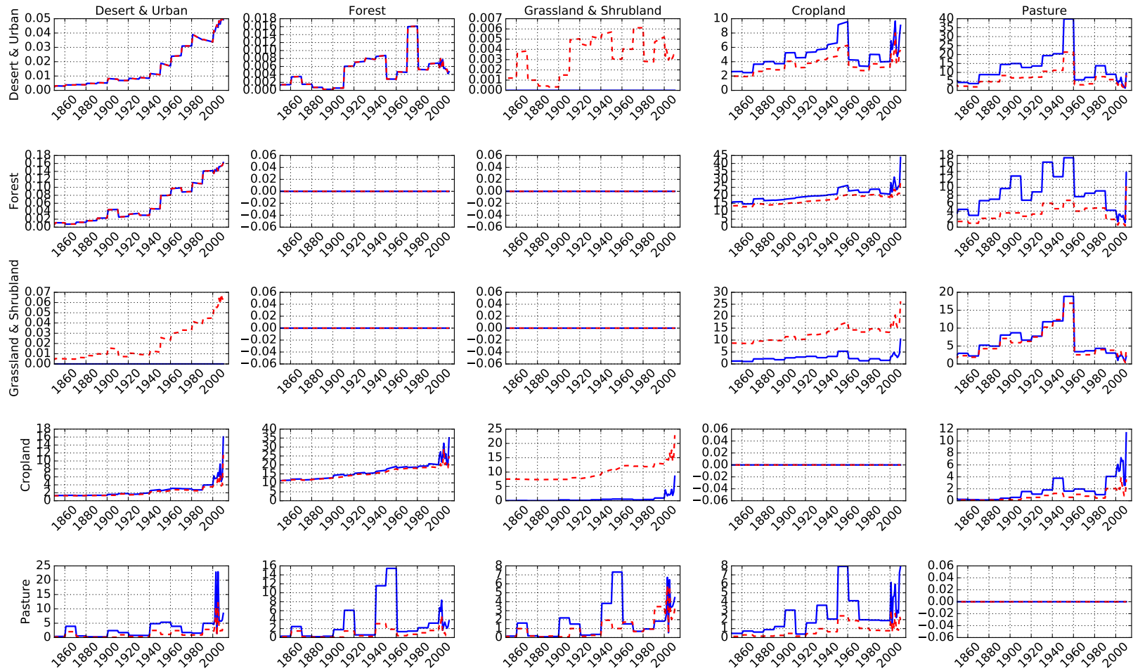
Figure 4.6: Global evolution of LUC (Mha/yr) over 1850-2015. The evolution from LUH1 is in plain blue line, whereas the evolution from LUH2 is in dashed red line.
