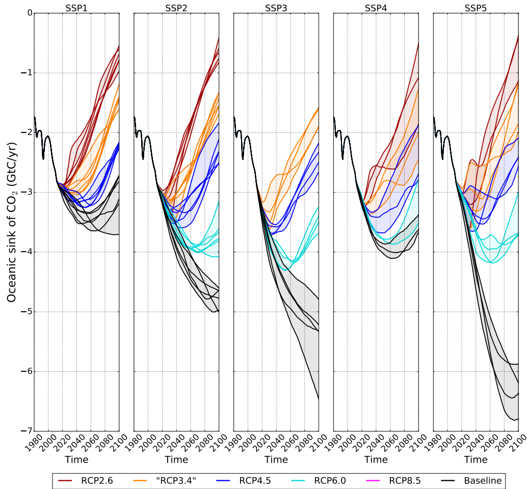
Figure 3.23: Ocean sink of \text{CO}_2 . Each subfigure details the results for a given SSP. The scenarios are also classified depending on the forcing target. Each plain line represents an IAM that has run this SSP and this forcing target. For the sake of clarity, uncertainties on SSP climate projections are not represented here.
