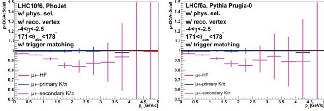
Figure 7.45: Ratio between the p_t distributions with p \times \text{DCA} cut in 5 \cdot \sigma(p \times \text{DCA}) and without this cut for different muon track sources from simulation from LHC10f6 (left) and LHC10f6a (right). The muon selection cuts are implemented.
