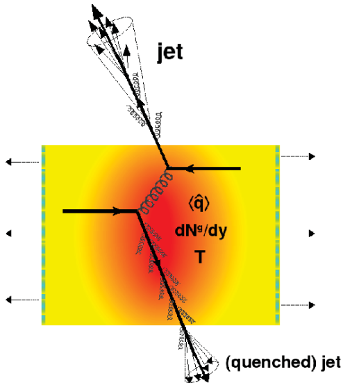
Figure 1.14: Jet Quenching
