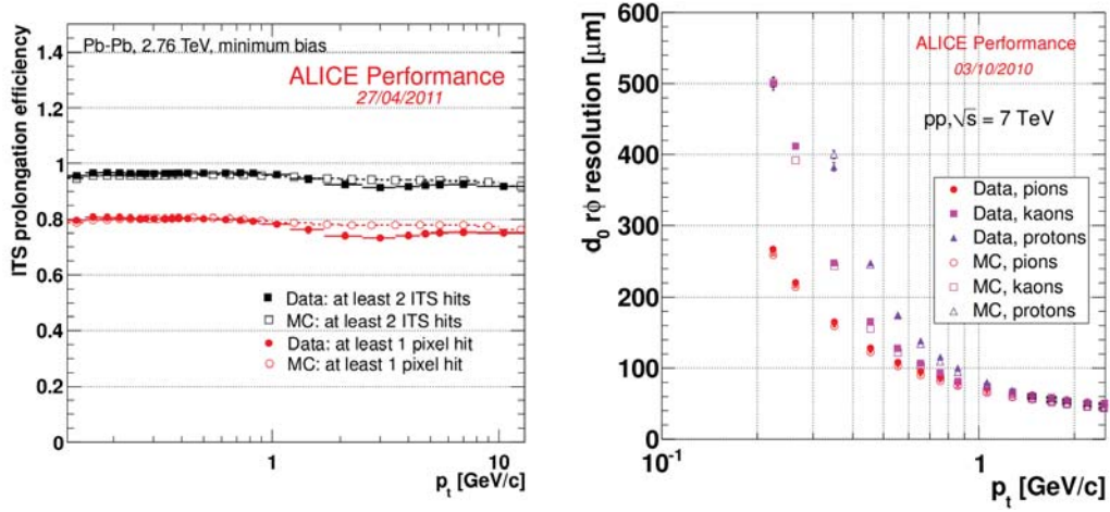
Figure 3.3: Left: track prolongation efficiency in ITS for TPC tracks, for the request of ITS-refit only (black) and ITS-refit with at least a point in SPD (red); data from Pb-Pb collisions at \sqrt{s_{NN}} = 2.76 TeV in 2010, MC results based on HIJING simulations. Right: transverse impact parameter resolution estimate as a function of p_t for pions, kaons, protons; data from pp collisions at \sqrt{s} = 7 TeV in 2010, MC corresponds to PYTHIA simulations with Perugia-0 configuration.
