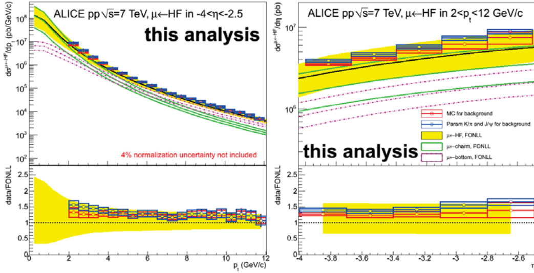
Figure 7.52: Similar as Fig. 7.48, but the production cross section of muons from heavy flavour decays based on the background estimate via the parameterized K/\pi and J/\Psi distributions are added at here.
