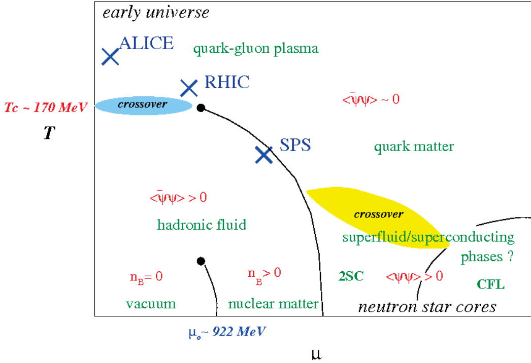
Figure 1.5: Schematic view of the QCD Phase Diagram
