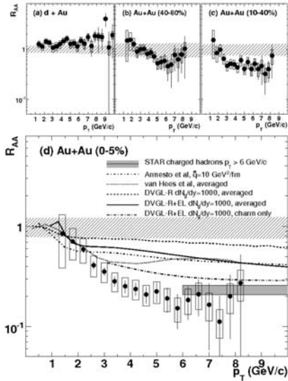
Figure 2.17: Nuclear modification factor R_{AA} of non-photonic electron measured in d–Au and Au–Au collisions at \sqrt{s_{NN}} = 200 \text{ GeV} with the STAR detector. Extracted from Ref. [201].
