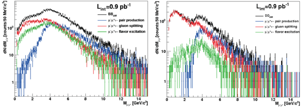
Figure 5.4: Reconstructed invariant mass distributions of correlated unlike-sign dimuons from BB_{\text{diff}} channel (left) and DD_{\text{diff}} channel (right) decay in pp collisions at \sqrt{s} = 14 TeV. The sources corresponding to different pQCD NLO processes of heavy flavour production are shown.
