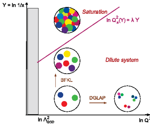
Figure 1.10: CGC Evolution
