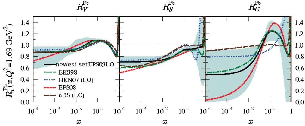
Figure 2.13: Comparison of the average valence quark, sea quark, and gluon modifications at Q^2 = 1.69 \text{ GeV}^2 ( \sim m_c^2 ) for a Pb nucleus, from LO global DGLAP analyses: EKS98, nDS [187], HKN07, EPS08 and EPS09LO.
