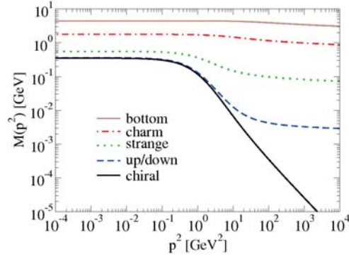
Figure 1.3: Constituent quark masses with various current masses of different flavours [32].
