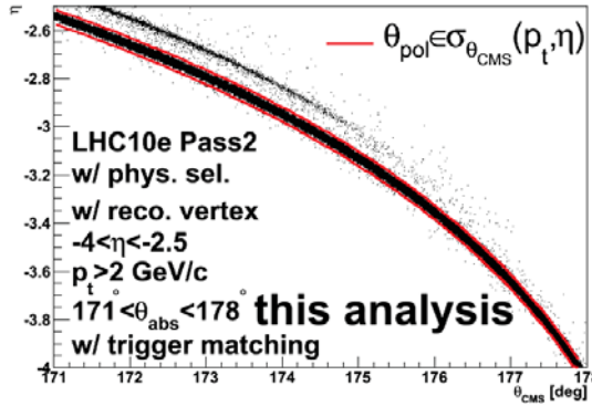
Figure 7.39: Same as the left panel of Fig. 7.35, but with the correlation between \eta and \theta_{\text{CMS}} as defined in Eq. (7.35), see text for more details.
