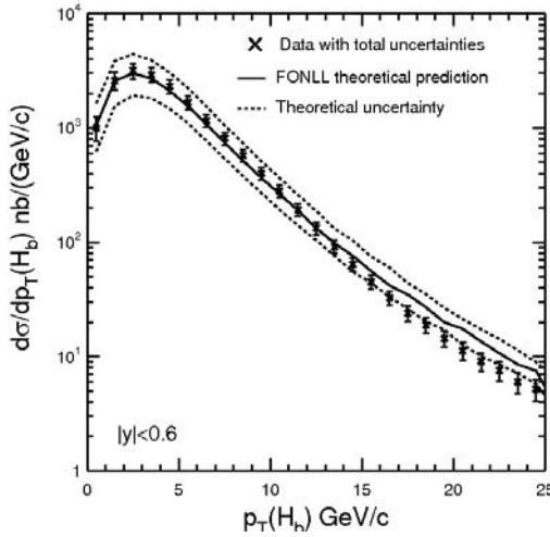
Figure 2.6: p_t -differential cross section of open b-hadron production [161] measured by CDF run II at Tevatron. Results are compared with FONLL predictions [162].
