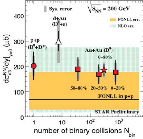
Figure 2.10: Charm production cross section per nucleon-nucleon collision at mid-rapidity as a function of N_{\text{bin}} (or N_{\text{coll}} ) measured at RHIC in Au-Au collisions at \sqrt{s_{\text{NN}}} = 200 GeV [177].
