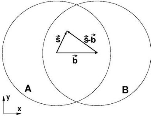
Figure 2.9: Collision geometry in the transverse plane.
