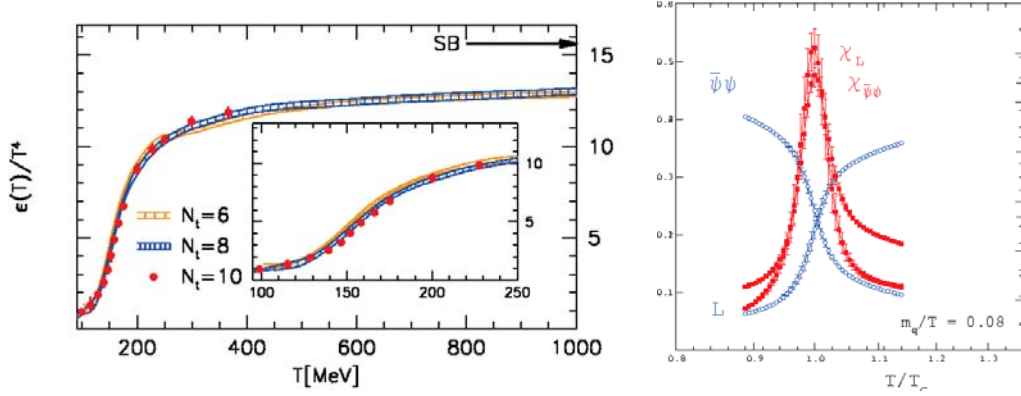
Figure 1.4: Left: energy density, \epsilon/T^4 , versus temperature, T , with 2 light and 1 heavier (strange) quarks [39]. Right: chiral condensation, \langle \bar{\Psi}\Psi \rangle (Eq. (1.11)), and quark free energy function, L(f_q) , (Eq. (1.13)) with their associated susceptibilities, \chi_{\bar{\Psi}\Psi} and \chi_L , as a function of temperature, T/T_c [34]. All the results are obtained with \mu_B = 0 .
