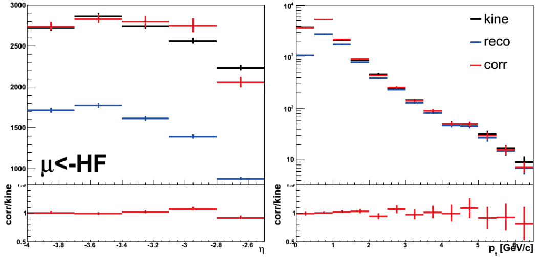
Figure 7.23: Same conditions as in Fig. 7.21, except that total muon signals from both open charm and beauty hadrons are used as input.
