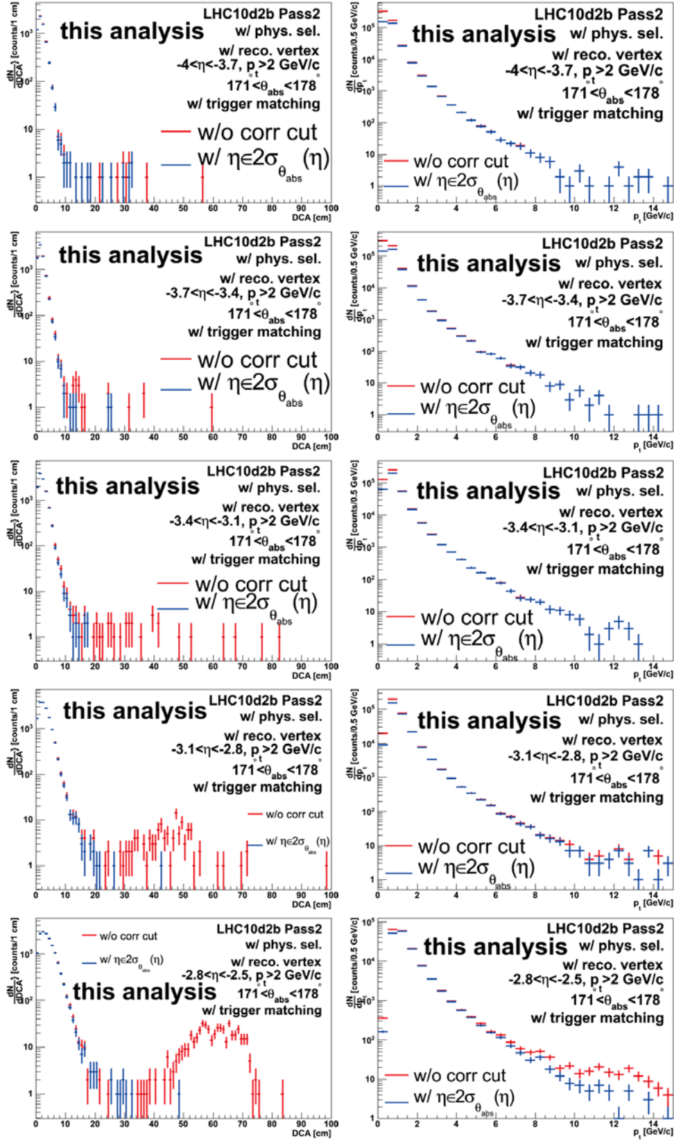
Figure 7.36: DCA (in p_t > 2 GeV/c, left column) and p_t (right column) distributions without (red lines) and with (blue lines) the combination cut defined in Eq. (7.34) in five pseudo-rapidity bins. The results are from the muon triggered data in LHC10d2b with the muon selection cuts.
