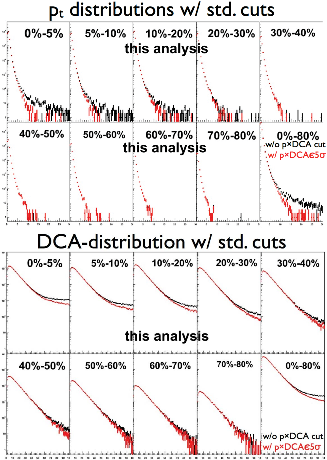
Figure 8.17: The p_t (upper) and DCA (lower) distributions of muon tracks with the standard selection cuts in different centrality classes. The results are obtained from LHC10h pass 2 data which is used for our final analysis. The distributions without the p \times \text{DCA} cut and those with p \times \text{DCA} cut are compared.
