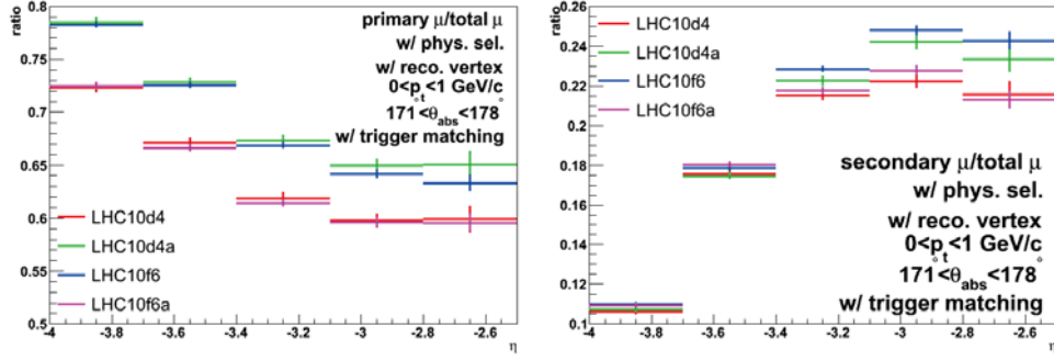
Figure 7.19: The ratios of primary muons (left) and secondary muons (right) to the total muons in 0 < p_t < 1 GeV/c (the region we used to calculate the R_{MC} ) in different simulations.
