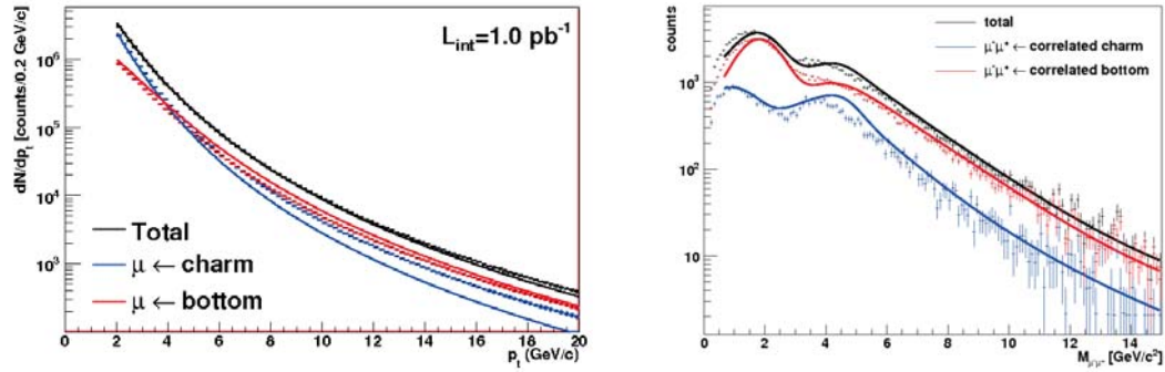
Figure 5.7: Example of combined fits obtained with biased f_{c/b}^{\mu^\pm} shapes for single muon p_t distribution (left) and with biased f_{c/b}^{\mu^-\mu^+} shapes for unlike-sign dimuon invariant mass distribution (right). The vertical error bars (smaller than the points for single muon channel) are the statistical ones.
