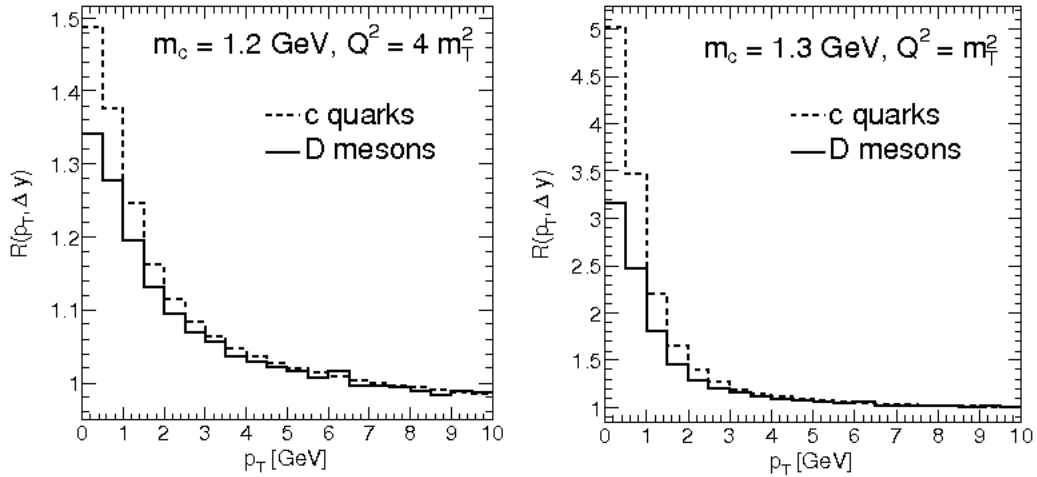
Figure 2.4: Enhancement factor R(p_t, \Delta y) for charm quarks (dashed lines) and D ( D^0 , D^+ ) mesons (solid lines), with m_c = 1.2 GeV/ c^2 , Q^2 = 4m_T^2 (left panel) and m_c = 1.3 GeV/ c^2 , Q^2 = m_T^2 (right panel) [132].
