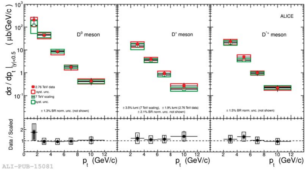
Figure 2.29: Upper: p_T -differential cross section for prompt D^0 , D^+ , and D^{*+} mesons in pp collisions at \sqrt{s} = 2.76 \text{ TeV} [224] compared with the scaling of the ALICE measurement at \sqrt{s} = 7 \text{ TeV} [225]. Bottom: ratio of the \sqrt{s} = 2.76 \text{ TeV} cross section and the \sqrt{s} = 7 \text{ TeV} measurement scaling. Results are obtained with ALICE.
