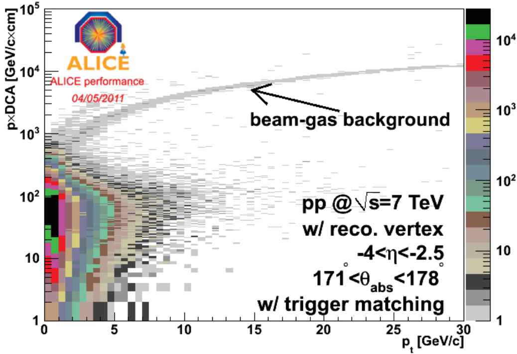
Figure 7.42: p \times DCA ( pDCA_{calib} as defined in Eq. (7.47)) versus p_t for muon trigger data in LHC10e. The muon selection cuts are applied.
