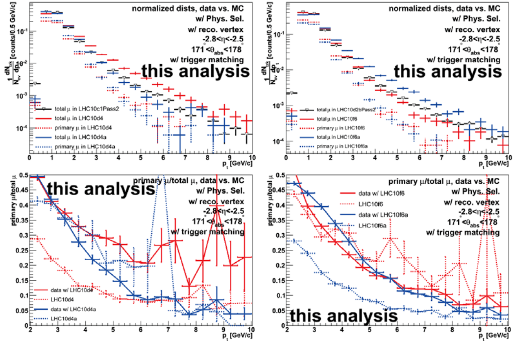
Figure 7.15: The same as Fig. 7.11, in -2.8 < \eta < -2.5 .
