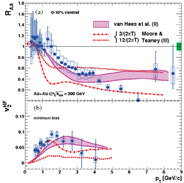
Figure 2.18: Nuclear modification factor and elliptic flow of non-photonic electrons measured in Au–Au collisions at \sqrt{s_{NN}} = 200 \text{ GeV} with the PHENIX detector. The data are compared to predictions from different Langevin based models (see text). Extracted from [202].
