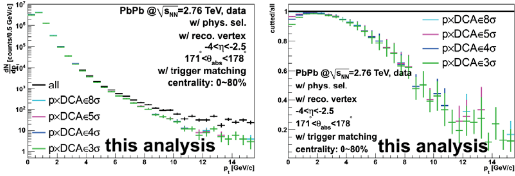
Figure 8.14: The left and right plots are similar to the upper and lower plots in the right plot of Fig. 7.43. The results are here obtained from LHC10h pass 2 data.
