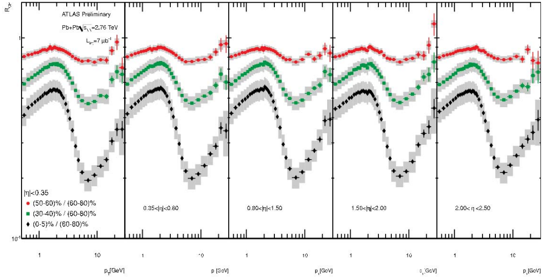
Figure 8.34: R_{CP} extracted from the inclusive charged particle distributions in different \eta ranges, and three centrality classes 0 – 5%, 30 – 40% and 50 – 60% with respect to a common peripheral sample (60 – 80%). Statistical errors are shown with vertical lines and the overall systematic uncertainty is shown with gray boxes [330].
