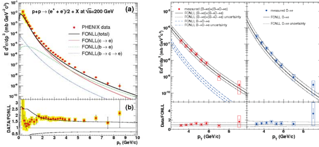
Figure 2.8: Left: (a) invariant differential cross sections of electrons from heavy flavour decays measured by PHENIX in pp collisions at \sqrt{s} = 200 GeV [166]. The curves are FONLL calculations [167]; (b) ratio of data and FONLL calculations, upper (lower) curve shows the theoretical upper (lower) limit of the FONLL calculations. Right: invariant cross section of (e^+ + e^-)/2 from beauty (upper-left) and charm meson (upper-right) decays measured by the STAR collaboration in pp collisions at \sqrt{s} = 200 GeV, together with the ratio of the corresponding measurements to FONLL predictions for beauty (lower-left) and charm electrons (lower-right) [168].
