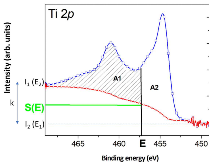
Figure 2.13. Shirley background of a Ti 2p spectrum.
