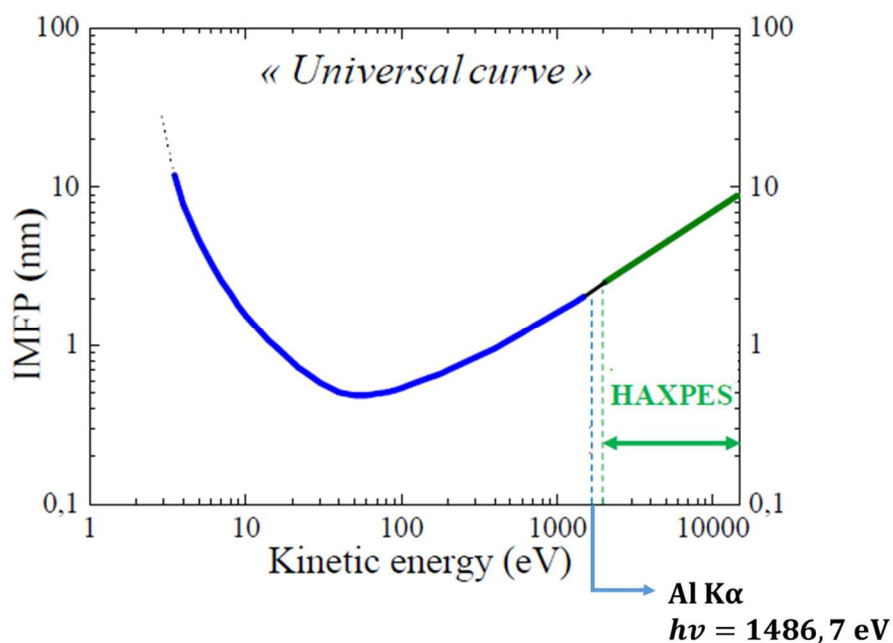
Figure 2.19. Universal curve representing the IMFP as a function of the kinetic energy of the photoelectrons. Adapted from Seah et al. [92].
