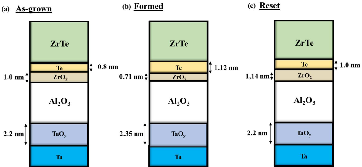
Figure 4.24 Evolution of the thicknesses of the Te, \text{ZrO}_2 and \text{TaO}_y layers during reverse forming and reset in the TiN/ZrTe/ \text{Al}_2\text{O}_3 /Ta memory stack.
