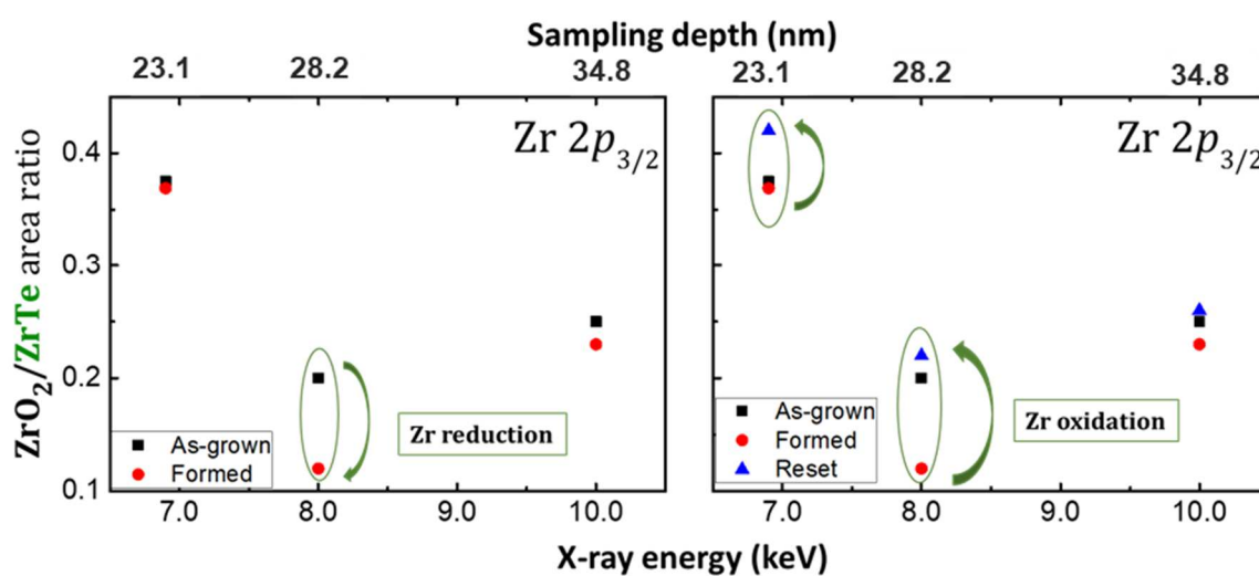
Figure 4.26. \text{ZrO}_2/\text{ZrTe} area ratios extracted from Zr 2p_{3/2} measured at 6.9, 8 and 10 keV for (a) as-grown, formed and (b) reset samples.
