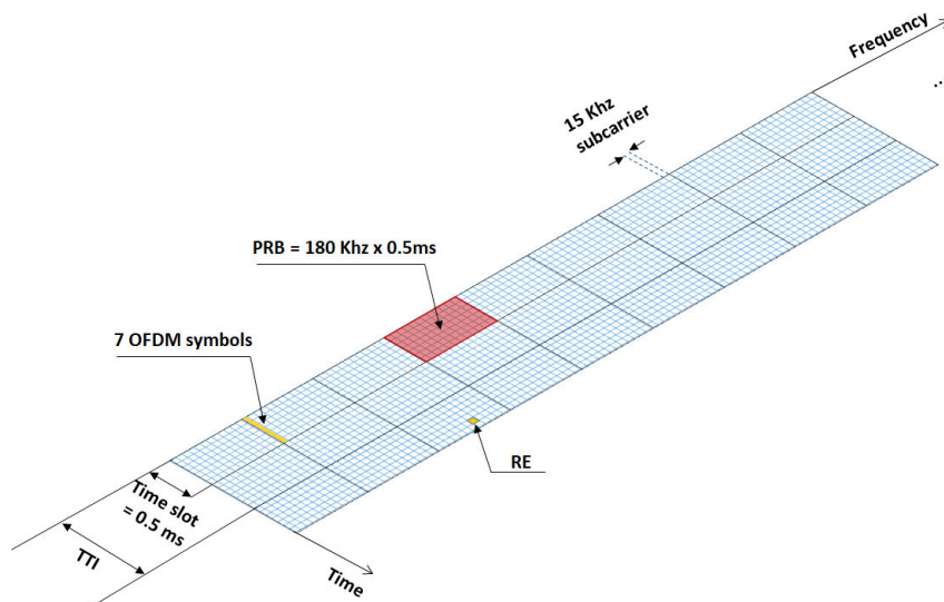
Figure 2.2: LTE resources.
