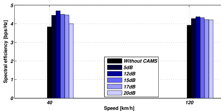
Figure 3.6: Spectral efficiency.
