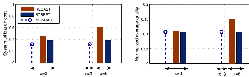
Figure 5.22: STREET vs. RECAST and NEWCAST: System utilization cost and normalized average quality in function of \pi for SD_{err} = 10^{-3} Mbits and a short horizon length of 10s.
