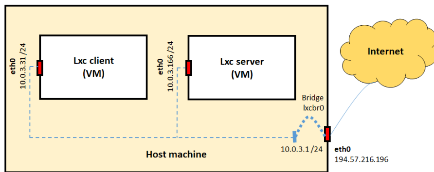
Figure 6.6: General IP configuration of the system used for experiments.
