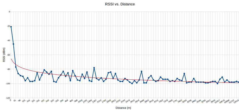
Figure 4.12 – Obtained RSSI values for experiment in the Roc’h Trevezel. The complex terrains in this area strongly impact on quality of radio links.
