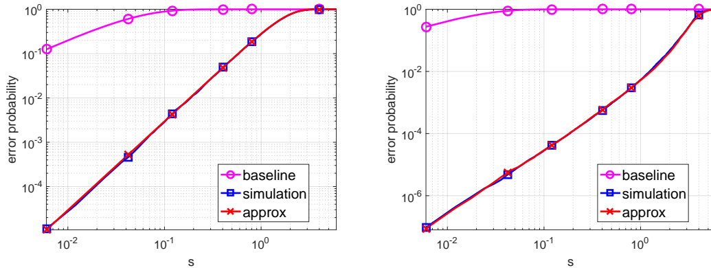
Figure 3.5: Multicast outage rate, probability of error 1 - P_+(s) vs s for n = 10^2 UEs. Scenario (1) (left), Scenario (2) (right).
