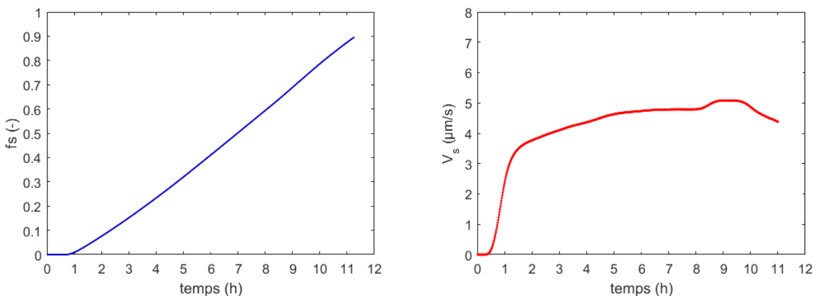
A - fraction solide.
