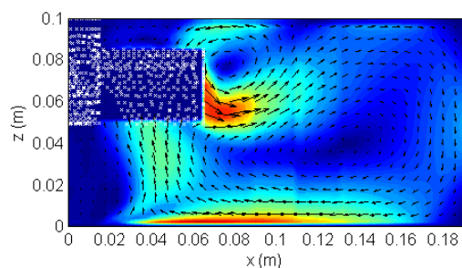
C1 - Simulation H = 10 cm ; N = 20 rpm
