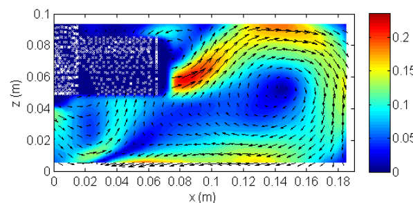
C2 - Mesure H = 10 cm ; N = 70 rpm
