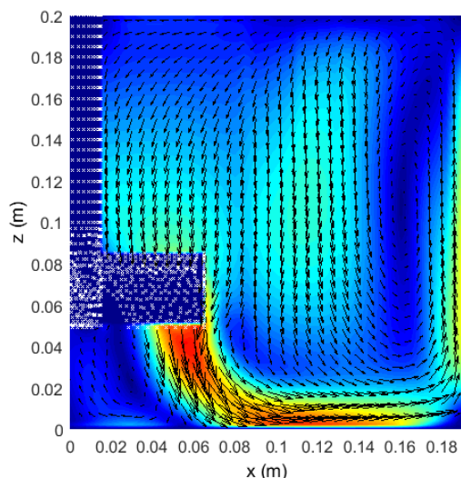
A1 - Simulation H = 20 cm ; N = 20 rpm
