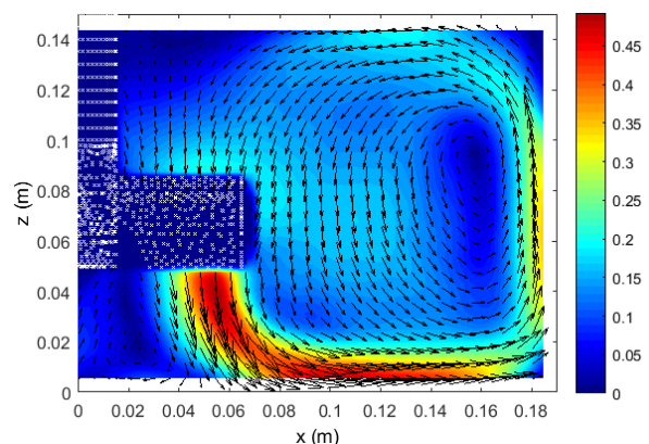
B2 - Mesure H = 15 cm ; N = 70 rpm
