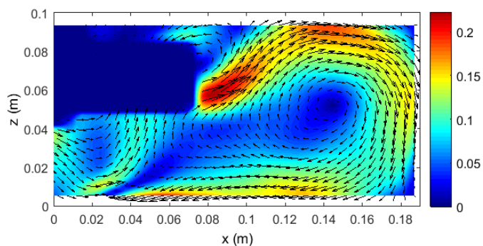
C - configuration 8 - H = 10 cm
