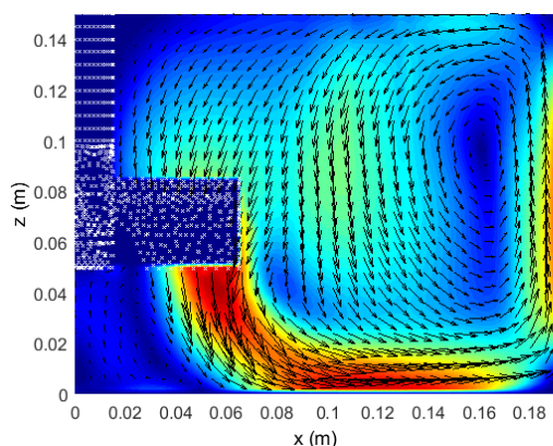
B1 - Simulation H = 15 cm ; N = 20 rpm
