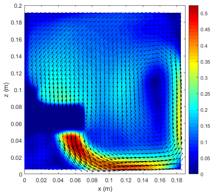
A - configuration 5 - H = 20 cm
