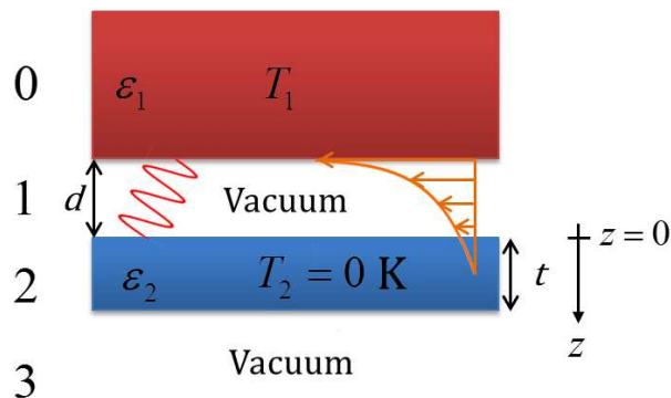
Figure IV.1: Case of a semi-infinite emitter separated by a vacuum gap of size d from a film of thickness t . The film is considered as non-emitting.
