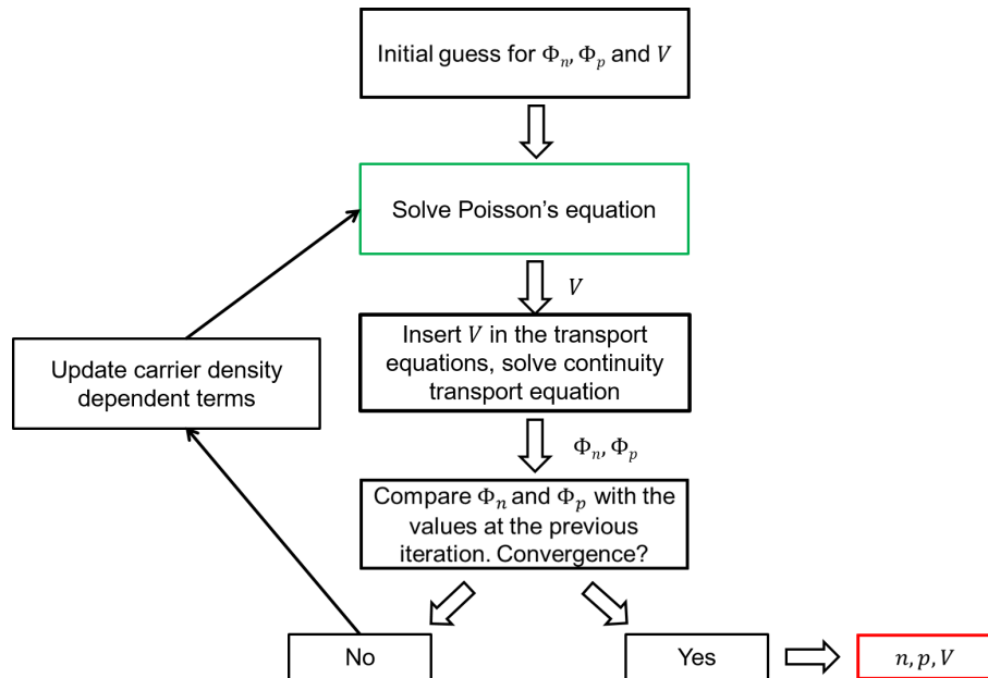
Figure V.3: Algorithm used to solve the Drift-Diffusion equations with Gummel's iteration method. The green frame represents the algorithm to solve Poisson's equation.
