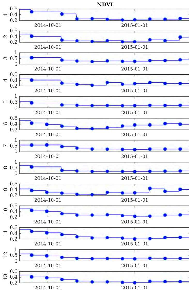
Figure D.3 – NDVI time series observed at each of the station locations (the station ID is indicated in the axis labels at the left). The values are extracted from the NDVI raster, input to the disaggregation algorithm in the C4DIS processor (Molero et al., 2016).
