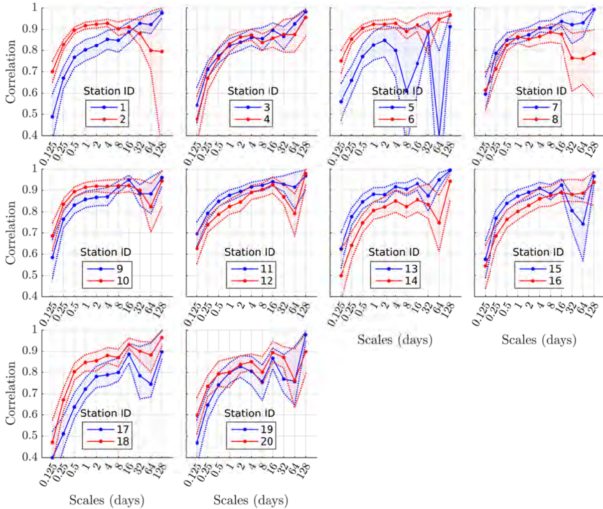
Figure C.1 – Correlation between the detail series of the point in situ series and the average in situ series of Little Washita, with the respective 95 % CIs calculated with the overlapping block bootstrap method
