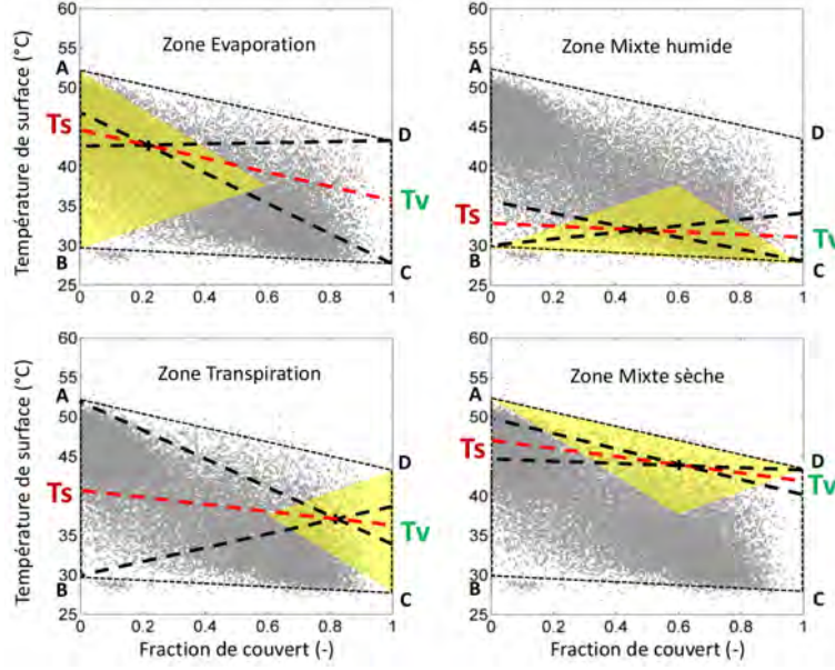
Figure A.1 – Example of the triangle method of Moran et al. (1994), which is based on the position of the pixel in the LST- f_v space, applied to the ASTER data acquired on the 17/08/2011 in Urgell, Spain. Source: Merlin (2016)
