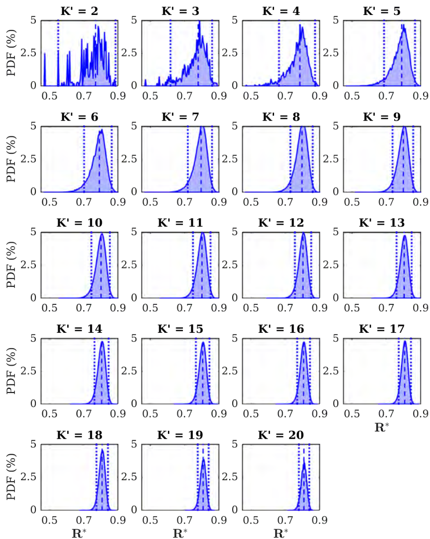
Figure F.1 – Bootstrap distribution of the correlation between SMOS and the in situ NAVg, as a function of the number of in situ time series taken to compute the NAVg. The dashed line correspond to the median and the dotted lines to the 5 % and 95 % confidence limits
