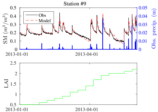
Figure 5.3 – Final model fit for station #9
