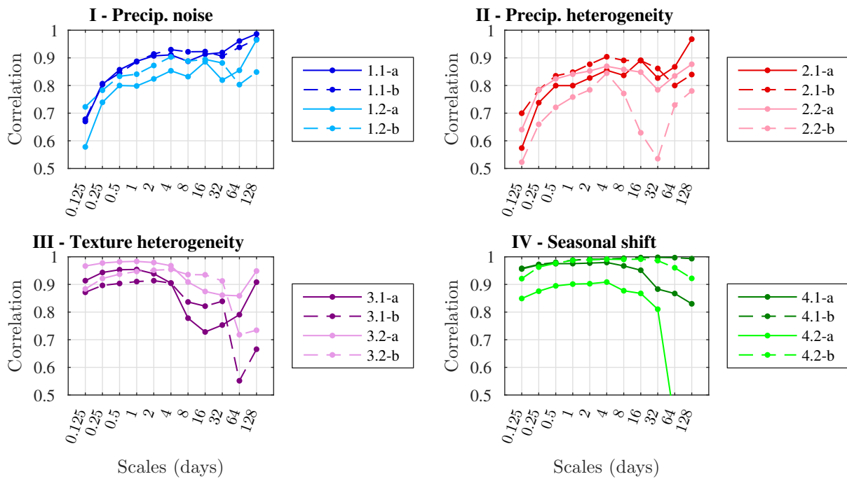
Figure 3.11 – Wavelet-based correlation between the modelled sample and reference series.
