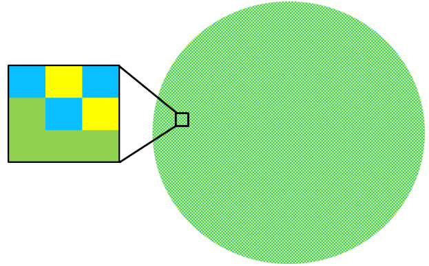
Figure 1.7 – Conceptual representation of the geophysical mismatch
