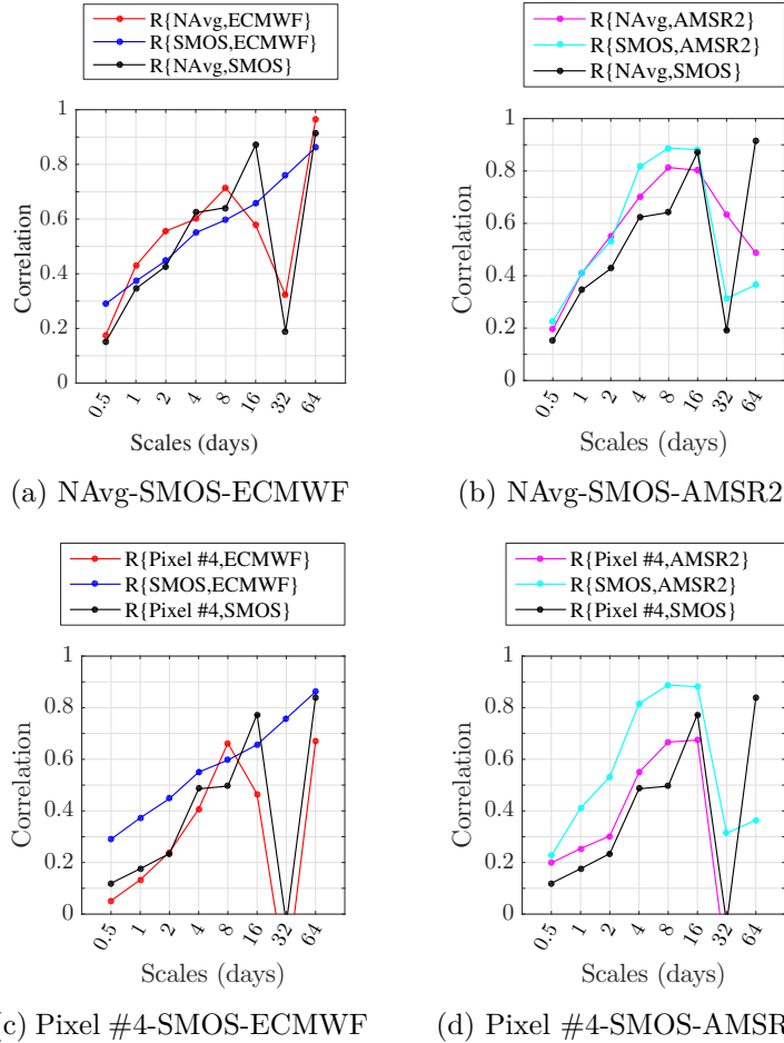
Figure 4.7 – Correlation between the detail series of the TC datasets. The left column represents the TC-ECMWF triplet and the right column, the TC-AMSR2 triplet. In the top row, the gridded SM dataset is the network average, in the bottom row, the gridded SM dataset is the pixel #4 time series
