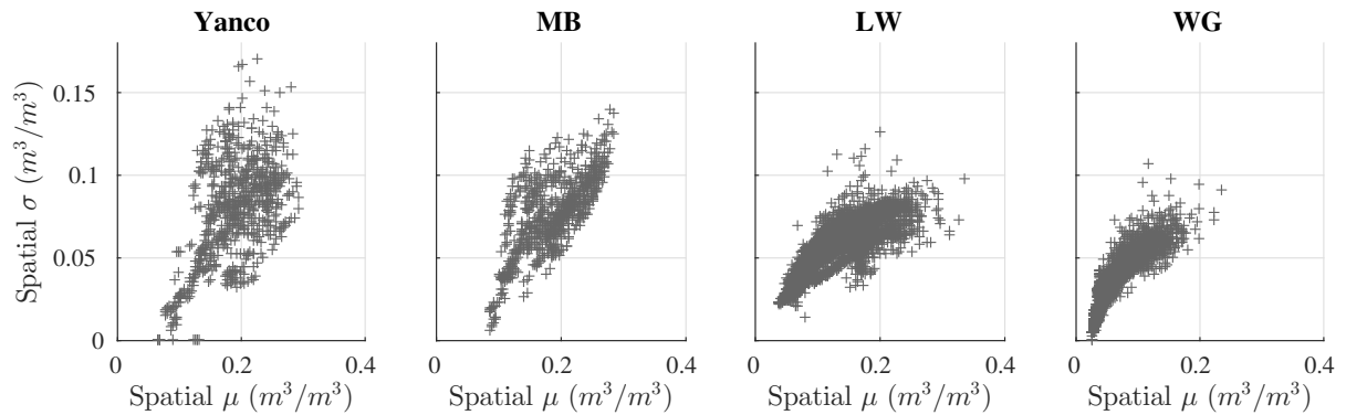
Figure 2.3 – The spatial standard deviation vs the spatial mean of the in situ samples of Yanco, MB, LW and WG, at the SMOS overpass times.
