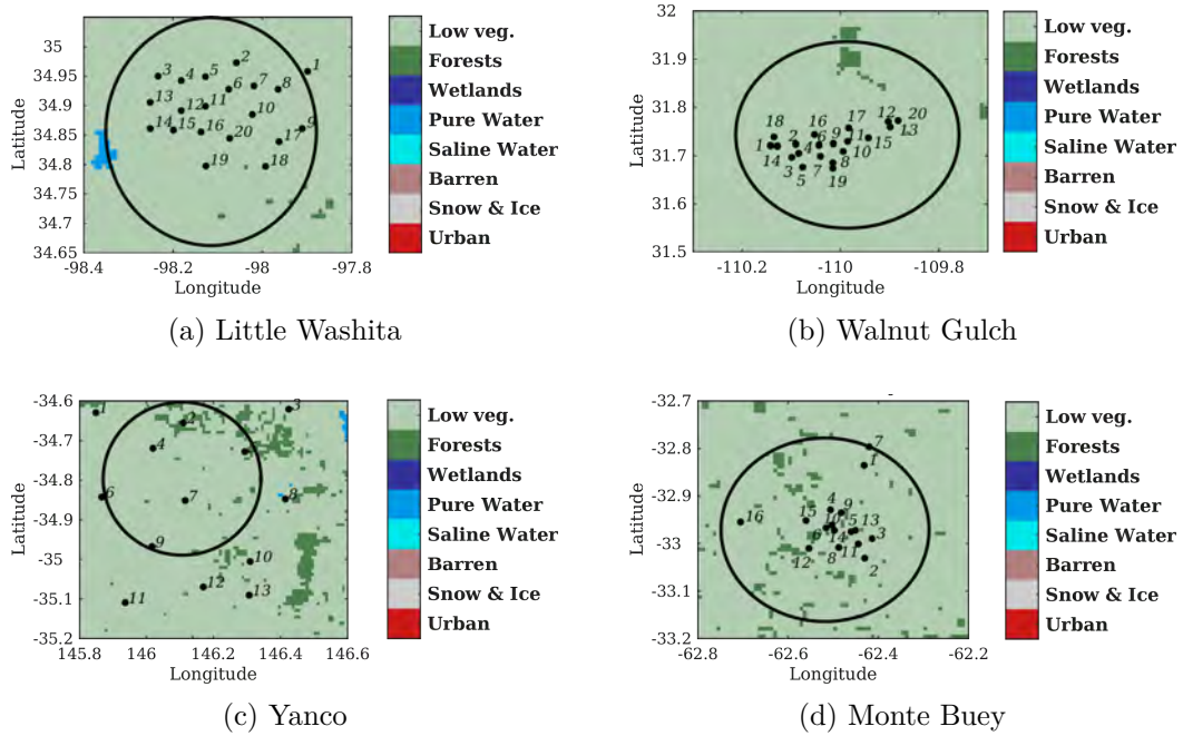
Figure D.2 – Aggregated Ecoclimap land cover maps for the four dense in situ networks used in this thesis. The aggregated classes are those considered in the SMOS retrieval algorithms. The circle represents a mean SMOS footprint size of 40 km.
