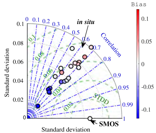
Figure 1.8 – Comparison of one SMOS soil moisture time series with 20 in situ time series corresponding to the same SMOS footprint
