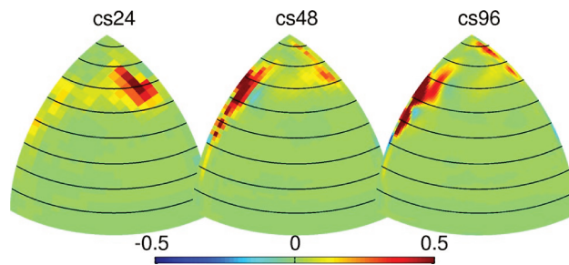
Fig. 11 Term -\overline{\mathbf{u}'T' \cdot \nabla\bar{T}} related to baroclinic instability eddy fluxes in the potential temperature variance budget averaged over the upper 1000 m ocean and over several MOC oscillation periods, in \text{K}^2 \text{ year}^{-1} . The thin black contours mark latitude circles every 10^\circ from 10^\circ to 80^\circ\text{N}
