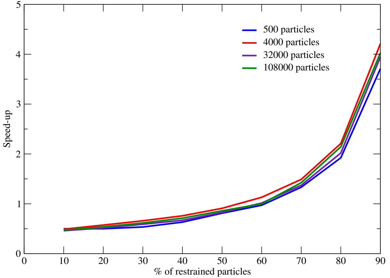
Fig. 3.2 Obtained speed-up in construction the ANL (compare to the HNL) as a function of percentage of restrained particles.
