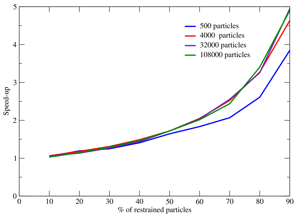
Fig. 3.3 case 1: Obtained speed up in performing integrations step.
