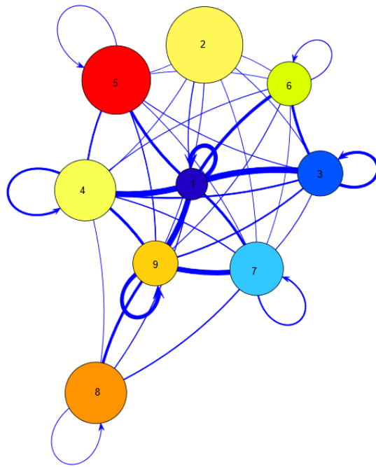
Figure 5.14: Summary of connection probabilities between groups.
