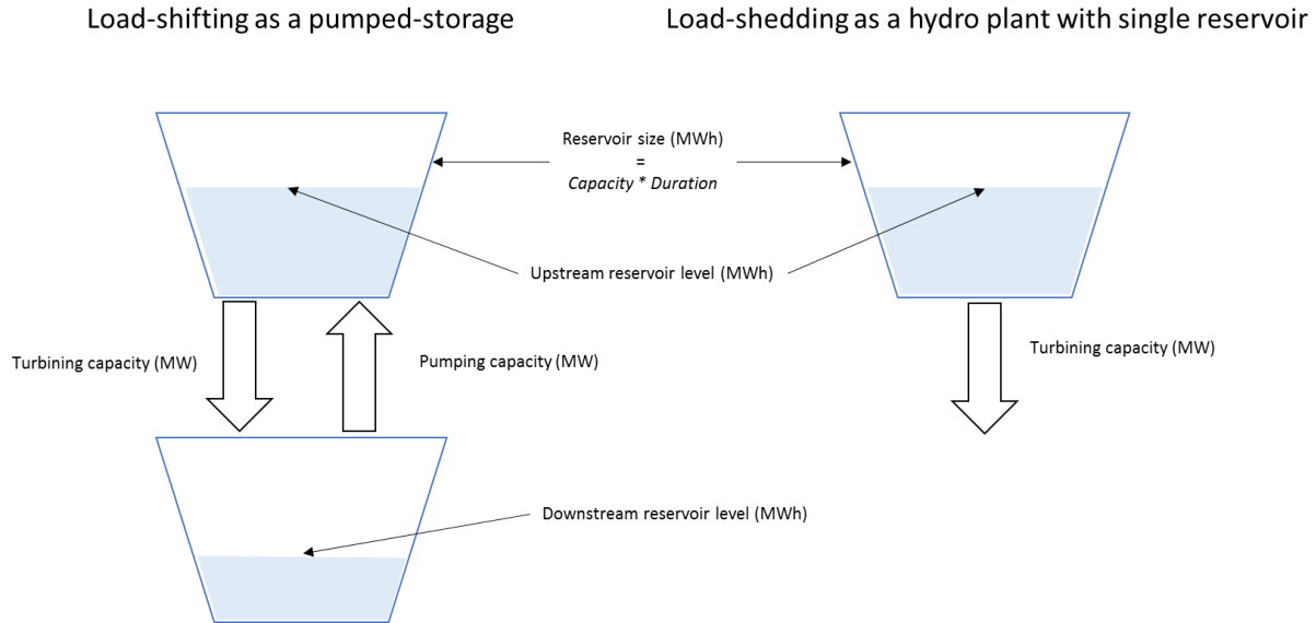
Figure 4.1 – Drawing of our Demand Response modelling approach
