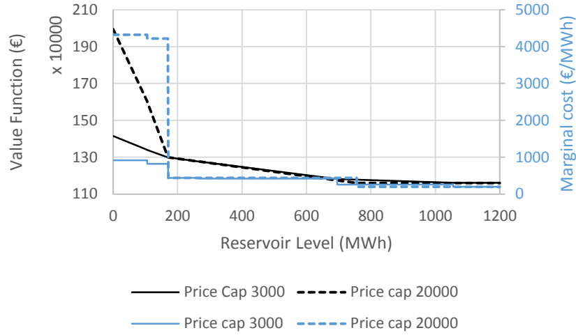
Figure 5.8 – Price cap impact on load-shedding_low marginal cost
