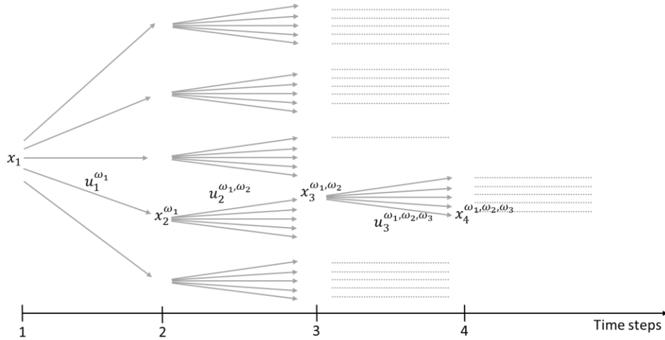
Figure 4.4 – Scenario tree
