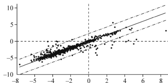
Fig. 3. Predicted rate constants of [4+2]π cycloaddition reactions in comparison with the experimental ones. Solid line corresponds to the ideal correlation between the predicted and experimental values. Dashed line corresponds to deviations of the predicted values from the observed ones on 3·RMSE.
