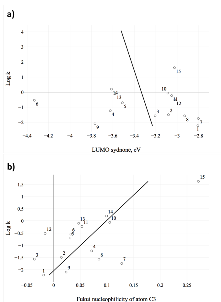
Figure 50. Dependency of rate constant on (a) LUMO energy of sydnone and (b) Fukui nucleophilicity on C3 atom. Reaction numbers corresponding to Table 7 is shown next to points.
