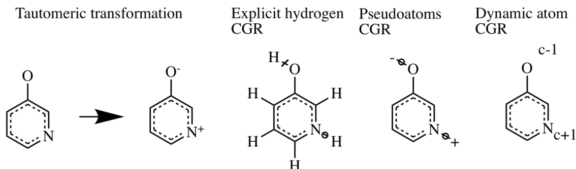
Figure 26. Dynamic atom representation in tautomeric equilibria. (ChemAxon Marvin Sketch representation [180]). Left side original tautomeric transformation, right side CGR representation with dynamic atoms.
