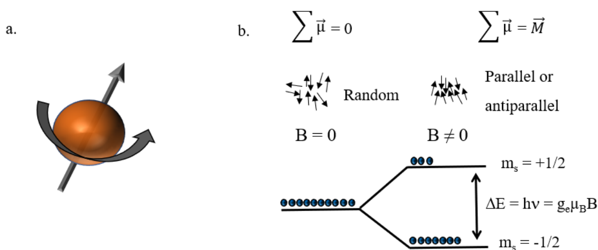
Figure 2.1 Schematic view of (a) an unpaired electron with a spin angular momentum (curved arrow) and magnetic moment (tilted arrow); (b) paramagnetic system in the presence of an external magnetic Field: the classical (up) and quantum approach (bottom) 8
