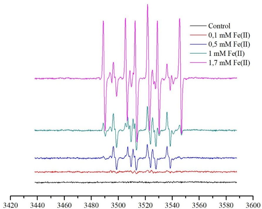
Figure A7.2: Spin-adducts and HEPES, Cum-OOH (0.54 mM) / DMPO (25 mM), Fe(II) varying concentrations
