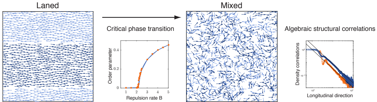
Figure 8 | Numerical simulations of active populations targetting opposite directions show two distinct phases, a laned phase and a mixed phase, separated by a critical phase transition. The mixed phase displays algebraic structural correlations.
