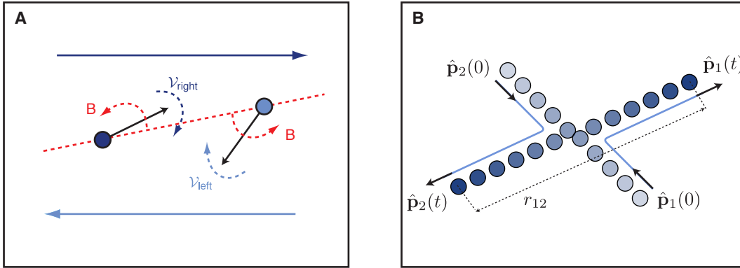
Figure 1.3 | Schematic description of the individual dynamics. (A) Illustration of the equations of motion Eqs. (1.2) and (1.3) for two particles of opposite species. Each particle travels at constant speed along its preferred direction (black arrow). Their respective orientations change via a repulsion torque B (red arrows) and the alignment on an external field \mathcal{V} (blue arrows). (B) Trajectories of two particles interacting solely via a repulsive torque as defined in Eq. (1.3). The post-collision orientations \hat{\mathbf{p}}_i(t) are along the center to center axis r_{ij} .
