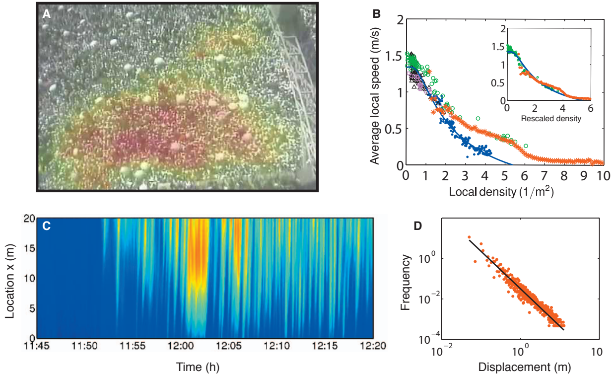
Figure 2 | Experimental data of the 2006 Hajj (all adapted from [43]). (A) Image from the video footage of the entrance of the Jamarat bridge, during the occurrence of the so-called crowd turbulence. Color codes for displacement intensity (B) Fundamental relation: local speed as a function of the local density. Red stars are from the Hajj measurements [43], black triangles [30], green circles [61] and purple squares [75] from street measurements and blue dots from a controlled experiment [82]. Solid blue line is a theoretical fit [99]. Inset: scaling the density by a factor of 0.7 for [43] and a factor of 0.6 for [61], the rescaled fundamental relations are compatible with the theoretical fit [99]. Same color codes. (C) Kymograph of the local density. After 11:50, density oscillations start to appear and propagate in the crowd. (D) Distribution of displacements in the “turbulent” phase.
