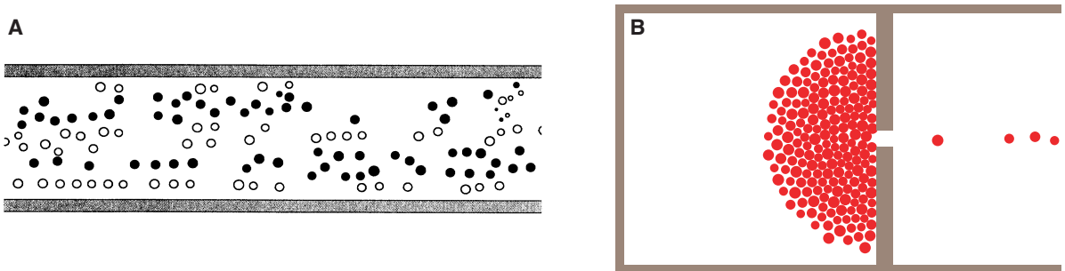
Figure 6 | The social force model qualitatively reproduces some large scale phenomena. (A) Lane formation in bidirectional flows (adapted from [45]). (B) Clogging at constrictions (adapted from [41]).
