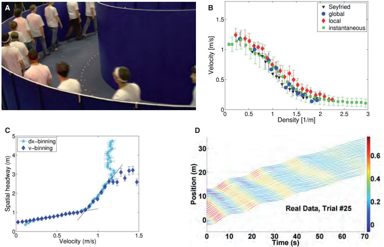
Figure 4 | Experimental results from unidimensional flows in a controlled setup . (A) Picture of the experimental setup. Participants are placed in a circular setup and instructed to follow one another without overtaking (adapted from [56]). (B) Fundamental relation between velocity and density. Blue dots are global measurements, red diamonds averaged over a segment of the setup and green squares are instantaneous measures. Black triangles are from averages over a segment of another setup [82] (adapted from [50]). (C) Instantaneous inter-pedestrian distance ( dx = 1/\rho ) as a function of velocity v . Light blue stars are for a binning over the distance and dark blue diamonds a binning over the velocity. (adapted from [50]). (D) Positions of pedestrians on the ring as a function of time as a velocity wave propagates and is damped. Color codes for the instantaneous velocity (adapted from [56]).
