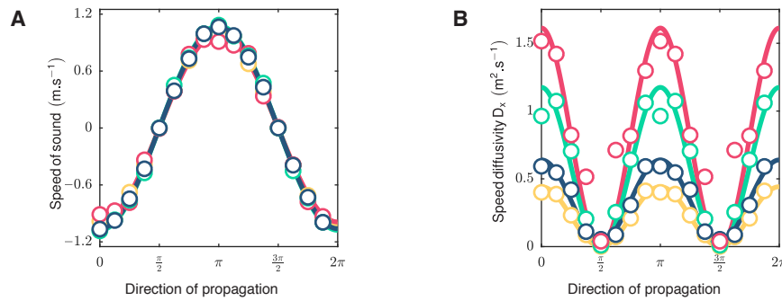
Figure 2.5 | Measurements of the hydrodynamic constants from spectral analysis (details are provided in Methods 4). (A) Variations of the speed of sound with the direction of the wave vector \theta for all experiments. Circles: experimental data. Solid line: cosine fit. The excellent fit shows that the dispersion relation is given by \omega = cq_x . (B) Variations of the speed diffusivity D_x with the direction of propagation. Circles: experimental data. Solid lines: squared cosine fits. Same color code as Fig 2.3c.
