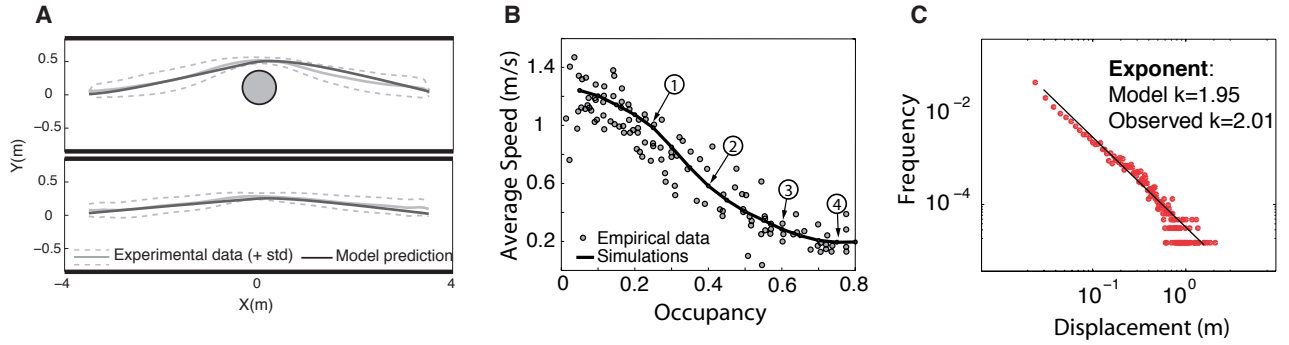
Figure 7 | Quantitative comparisons between the heuristic model and experiments (all adapted from [66]). (A) Trajectory comparison of obstacle (top) and pedestrian (bottom) avoidance in a narrow corridor. Light grey: experiments (from [64]). Dark grey: model. (B) Speed-density comparison between numerical simulations of 6 to 96 pedestrians in a unidirectional corridor and field measurements (from [70]). (C) Frequency-amplitude of displacement bursts comparison between numerical simulations of 360 pedestrians at a bottleneck and field measurements (from [43]).
