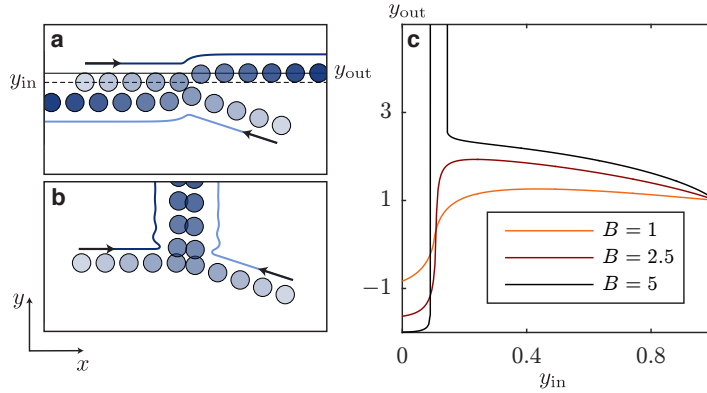
Figure 1.8 | Collision between left and right movers. (a) and (b) Trajectories of two colliding particles in the presence of an alignment field. The trajectories before contact are prolongations of the incoming orientations, both interactions and alignment field are only turned on at contact. (a) Scattering trajectory for B = 5 , and y_{in} = 0.75 . y_{in} (resp. y_{out} ) is the initial (resp. final) vertical position of the right mover with respect to the contact point. y_{in} (resp. y_{out} ) is represented by the dashed line (resp. plain line). (b) Example of collision resulting in a strong and persistent deviation along the transverse direction ( B = 5 , y_{in} = 0.125 ). (c) The transverse displacement y_{out} is plotted as a function of the impact parameter y_{in} as defined in (a), for different values of the repulsion strength B . Initial conditions: a right mover with an orientation \theta_r = 0 and a left mover with \theta_l = \pi - \pi/10 are vertically placed at +y_{in} and -y_{in} . Their x coordinate is chosen so that they start interacting at t = 0 .
