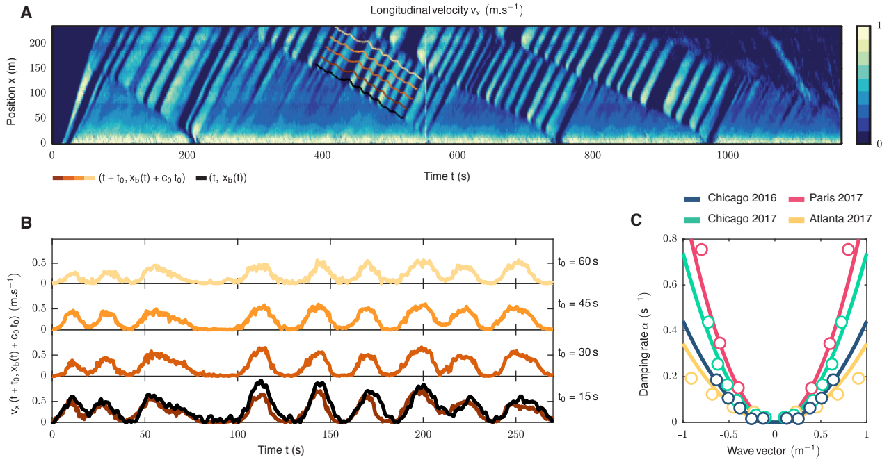
Figure 2.3 | Underdamped propagation of linear and non dispersive velocity waves. (A) Kymograph of the longitudinal velocity, averaged over the transverse direction (Chicago 2016). The position x indicates the distance from the starting line. A number of velocity waves are seen to propagate upstream at the same speed. (B) Black line: velocity of a chain of race-staff members \dot{x}_b(t) , measured by direct tracking. The corresponding positions x_b(t) are reported as a black line on the kymograph in (A). As illustrated with the same color code on the the kymograph (A), the colored curves correspond to the longitudinal velocity field measured along the curves defined by the race staff position x_b(t) after four different waiting times t_0 : v_x(t + t_0, x_b(t) + c_0 t_0) . Independently of the shape of the \dot{x}_b(t) signal, the velocity waves faithfully propagate the information of the boundary speed \dot{x}_b(t) over system spanning scales, at constant speed. (C) Damping rate of the speed waves plotted for all wave vectors along the direction of propagation \theta = \pi/4 . Circles: experimental data. Solid lines: best quadratic fits.
