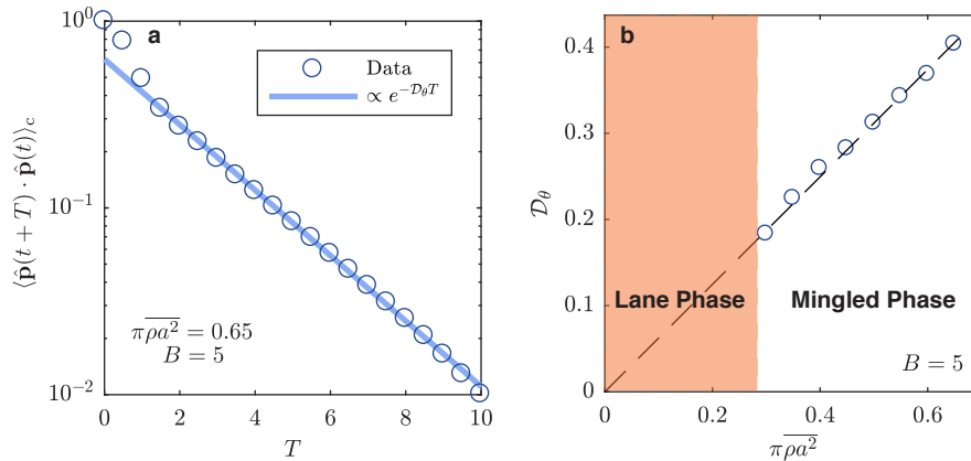
Figure 1.10 | Computation of the orientational diffusivity. (a) Log-linear plot of the orientational diffusivity. Dark blue circles: Numerical time autocorrelation function of the unit orientation vector \hat{\mathbf{p}} averaged over all the particles, in the mingled phase at repulsion magnitude B = 5 and density \overline{\pi\rho a^2} = 0.65 . Light blue line: best exponential fit. (b) Orientational diffusivity \mathcal{D}_\theta as a function of the particle area fraction \overline{\pi\rho a^2} , at constant repulsion magnitude B = 5 . It is very nicely approached by a linear fit starting from the origin. The orange area represents the location of the lane phase.
