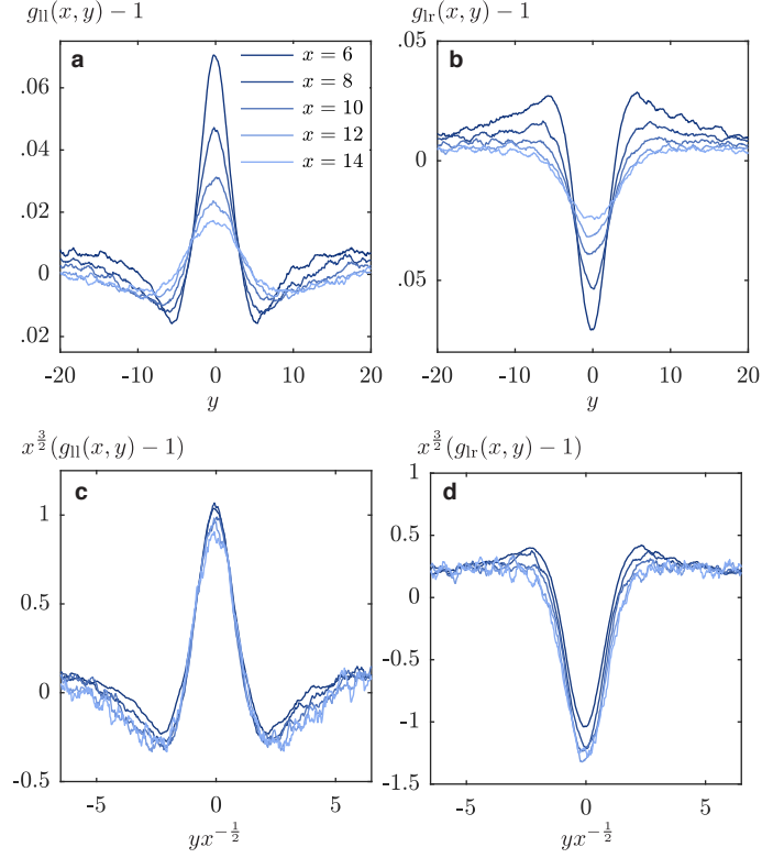
Figure 1.12 | Density correlation functions evaluated at a fixed values of x plotted versus the distance in the transverse direction y . Simulations performed deep in the homogeneous phase ( B = 5 and \pi\rho a^2 = 0.65 ). (a) Bare pair correlation functions for particles of the same population g_{||}(x, y) (left movers). (b) Bare pair correlation function for particles belonging to different populations g_r(x, y) . (c) and (d) Collapse of the pair correlations once rescaled by the universal x^{-3/2} power law and plotted as a function of the rescaled distance y/\sqrt{x} . The good collapse of the rescaled curves supports the validity of the scaling deduced from the linearized fluctuating hydrodynamics.
