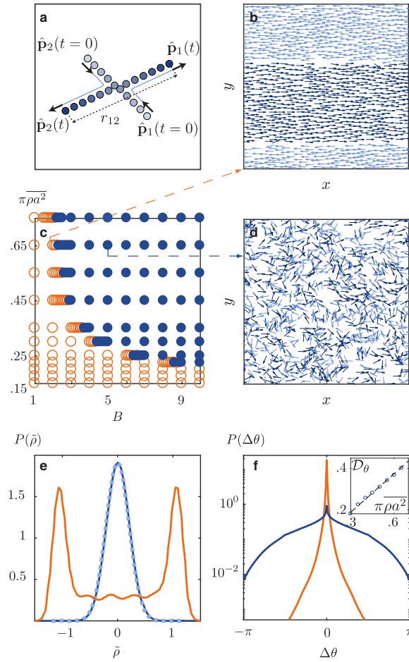
Figure 1.6 | Phase behavior. (a) Trajectories of two particles interacting solely via a repulsive torque as defined in Eq. (1.9) with B = 5 . The post-collision orientations \hat{\mathbf{p}}_i(t) are along the center to center axis r_{ij} . (b) and (d) Snapshots of a square window at the center of the simulation box ( L_x = 168 , N = 1973 , \pi\rho a^2 = 0.65 ), respectively in the lane ( B = 2 ) and the homogeneous ( B = 5 ) states. The arrows indicate the instantaneous position and orientation of the particles. Dark blue: right movers. Light blue: left movers. (c) Phase diagram. \pi\rho a^2 is the particle area fraction. Filled symbols: homogeneous state. Open symbols: lanes. (e) Probability distribution of the density difference \tilde{\rho} = \rho_r - \rho_l . Light orange line: B = 2 , \pi\rho a^2 = 0.65 . Dark blue line: B = 5 , \pi\rho a^2 = 0.65 . Dashed line: best Gaussian fit. (f) P.d.f. of the orientational fluctuations around the preferred orientation (lin-log plot). Same parameters and colors as in (e). Inset: orientational diffusivity \mathcal{D}_\theta in the homogeneous state at a fixed repulsion magnitude ( B = 5 ) and different particle area fractions \pi\rho a^2 . \mathcal{D}_\theta is defined as the decorrelation time of the particle orientation. In the mingled state, the velocity autocorrelation decays exponentially at short time, \mathcal{D}_\theta is therefore defined without ambiguity, see also Supplementary Note 1 for a full description of the numerical computation of \mathcal{D}_\theta . Dashed line: best linear fit.
