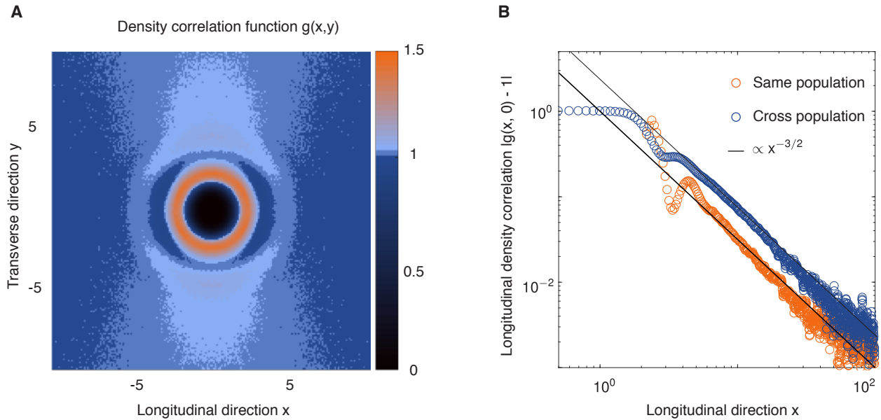
Figure 1.5 | Numerical evidence of long-range structural correlation. (A) Overall pair correlation function g(x, y) . (B) Plot of the longitudinal decay of the density auto- (light orange) and cross- (dark blue) correlation functions at y = 0 . Black lines: algebraic decay x^{-\frac{3}{2}} .
