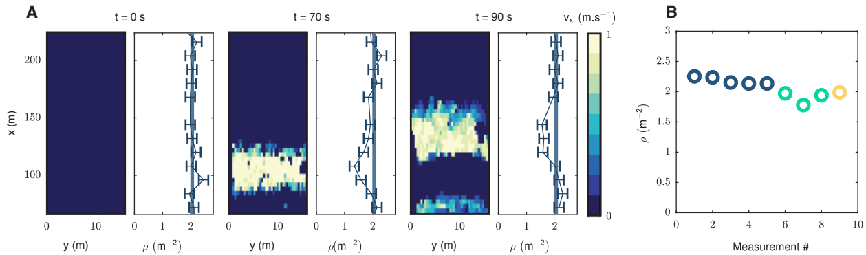
Figure 2.2 | Density measurements in queuing crowds. (A) Velocity and density fields at three successive times. At t = 0 s the crowd is static and has a uniform density \rho_0 \sim 2 \text{ m}^{-2} (blue lines). At t > 0 , as the staff members displaces the downstream boundary of the queuing crowd, a hybrid wave packet coupling velocity and density fluctuations propagates upstream. (B) For all events in which the density estimation was possible, the density in static crowds is roughly the same and equal to \rho_0 = 2.2 \pm 0.05 \text{ m}^{-2} . The color code for each race is provided in Fig. 2.3c
