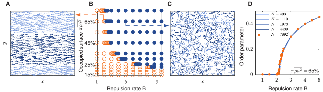
Figure 1.4 | A true phase transition. (A) and (C) Snapshots of the numerical simulations in (A) the laned phase and (C) the mingled phase. The arrows indicate the instantaneous position and orientation of the particles. Dark blue: right movers. Light blue: left movers. (B) Phase diagram. \overline{\pi \rho a^2} is the particle area fraction. Filled symbols: mingled phase. Open symbols: laned phase. (D) Order parameter at different repulsion rates B at a surface occupation of 65%. The bifurcation curves collapse for five system sizes.
