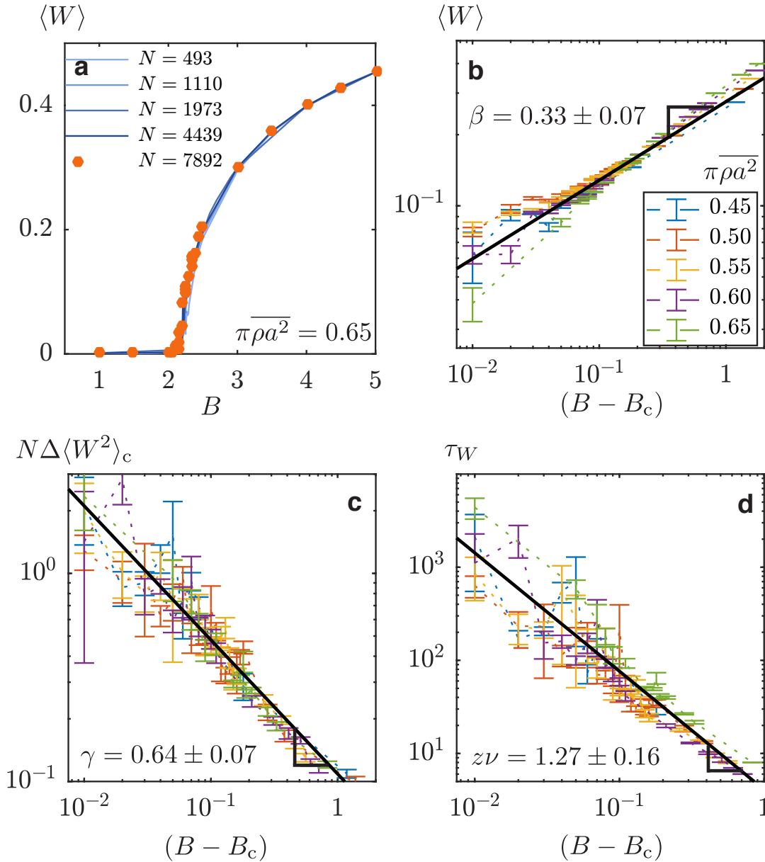
Figure 1.7 | Critical transition from laned to homogeneous liquid states. (a) and (b) Linear and log plots of the order parameter \langle W \rangle defined in Eq. (1.10). (a): \overline{\pi\rho a^2} = 0.65 , the bifurcation curves collapse for five system sizes. (b), (c) and (d) Log plots at five densities for a box of length L_x = 336 ( N ranges from 5462 to 7892). (c) Fluctuations of the order parameter plotted versus B - B_c for the same densities as in (b). The fluctuations are defined as \Delta\langle W^2 \rangle_c \equiv \langle W^2 \rangle_c(B) - \langle W^2 \rangle_c(B \rightarrow \infty) . (d) Correlation time \tau_W plotted against B - B_c . The correlation time is defined as \langle W(t + \tau_W)W(t) \rangle_c = \frac{1}{2}\langle W^2(t) \rangle_c . All error bars correspond to two standard deviations. The error on the estimate of the exponents correspond to one standard deviation after considering linear fits for each density.
