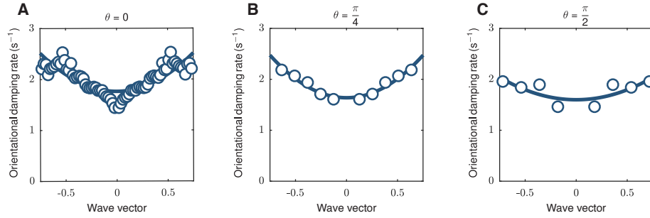
Figure 2.16 | (Chicago 2016) Orientational damping rate as a function of the wave vector, in directions of propagation (A) \theta = 0 , (B) \theta = \pi/4 , and (C) \theta = \pi/2 . In every propagation direction, the orientational damping grows quadratically with the wave vector.
