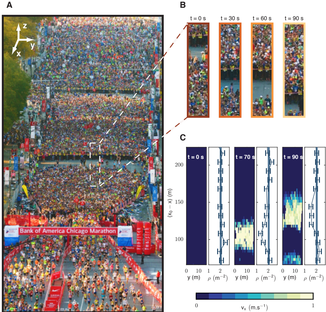
Figure 2.13 | Hybrid-wave propagation in queuing crowds. (A) Picture of the starting corrals of the Bank of America Chicago Marathon (2017) taken from an elevated observation point, see Methods 4. Thousands of runners progress towards the starting line under the guidance of race staff members. (B) The chain formed by the race staff advances with repeating sequences of walks and stops. (C) Velocity and density fields at three successive times. At t = 0 s the crowd is static and has a uniform density \rho_0 \sim 2 \text{ m}^{-2} (blue lines). At t > 0 , as the staff members displaces the downstream boundary of the queuing crowd, a hybrid wave packet coupling velocity and density fluctuations propagates upstream. x_0 - x indicates the distance from the starting line located at x_0 .
