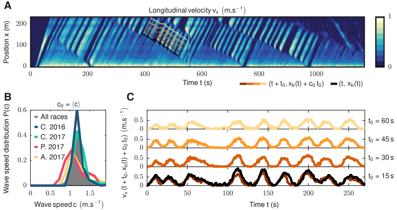
Figure 2.14 | Underdamped propagation of linear and non dispersive velocity waves. (A) Kymograph of the longitudinal velocity, averaged over the transverse direction (Chicago 2016). x_0 - x indicates the distance from the starting line. A number of velocity waves are seen to propagate upstream at the same speed. (B) Probability distribution function of wave speed, measured for all the studied events. The typical wave speed hardly differs from one event to the other. The overall speed distribution is narrowly peaked around, \langle c \rangle = c_0 = 1.2 \pm 0.3 m.s -1 . (C) Black line: velocity of a chain of race-staff members \dot{x}_b(t) , measured by direct tracking. The corresponding positions x_b(t) are reported as a black line on the kymograph in (A). As illustrated with the same color code on the the kymograph (A), the colored curves correspond to the longitudinal velocity field measured along the curves defined by the race staff position x_b(t) after four different waiting times t_0 : v_x(t + t_0, x_b(t) + c_0 t_0) . Independently of the shape of the \dot{x}_b(t) signal, the velocity waves faithfully propagate the information of the boundary speed \dot{x}_b(t) over system spanning scales, at constant speed.
