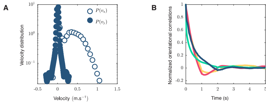
Figure 2.4 | (A) Probability distribution function of the longitudinal and transverse components of the velocity field (Chicago 2016). The longitudinal component dominates. (B) Normalized orientational correlations plotted versus time for all experiments ( \theta = \pi/4 , q = 0.5 \text{ m}^{-1} ). Same color code as Fig 2.3c.
