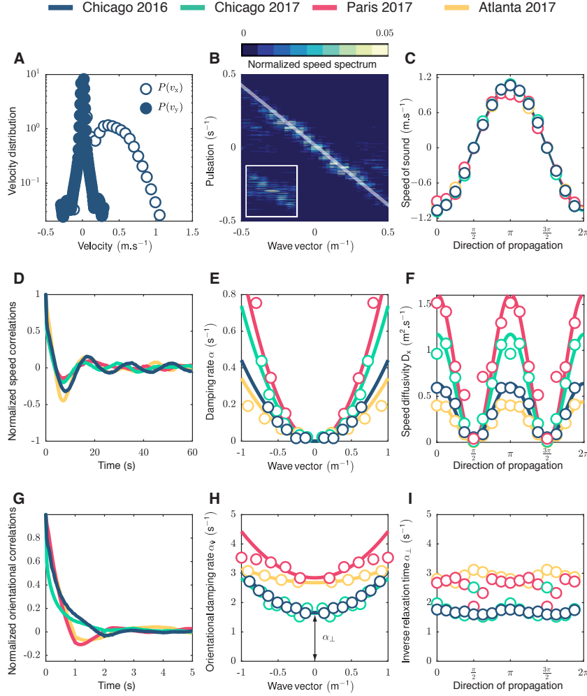
Figure 2.15 | Spectral properties of speed waves in queuing crowds. (A) Probability distribution function of the longitudinal and transverse components of the velocity field (Chicago 2016). The longitudinal component dominates. (B) Power spectrum of the flow speed, plotted for \theta = \pi/4 . The spectrum is normalized at every wave vector ( \int C_v(\omega, q, \theta) dq = 1 ). Inset: normalized speed spectrum for a crowd in free flow conditions. Data from the Chicago 2016 experiment. (C) Variations of the speed of sound with the direction of the wave vector \theta for all experiments. Circles: experimental data. Solid line: cosine fit. The excellent fit shows that the dispersion relation is given by \omega = cq_x . (D) Normalized speed correlations plotted versus time for all experiments ( \theta = \pi/4 , wave vector q = 0.5 \text{ m}^{-1} ). (E) Damping rate of the speed waves, \alpha , plotted for all wave vectors along \theta = \pi/4 . Circles: experimental data. Solid lines: best quadratic fits. (F) Variations of the speed diffusivity D_x with the direction of propagation. Circles: experimental data. Solid lines: squared cosine fits. (G) Normalized orientational correlations plotted versus time for all experiments ( \theta = \pi/4 , q = 0.5 \text{ m}^{-1} ). (H) Damping rate of the orientational fluctuations \alpha_{\hat{v}} plotted as a function of the wave vector ( \theta = \pi/4 ). Circles: experimental data. Solid lines: best quadratic fits \sim \alpha_{\perp} + D_{\hat{v}} q^2 , with D_{\hat{v}} = 1.2 \pm 0.5 \text{ m}^2 \text{ s}^{-1} . (I) Inverse relaxation time \alpha_{\perp} plotted as a function of the direction of the wave vector \theta . No significant angular variation is observed.
