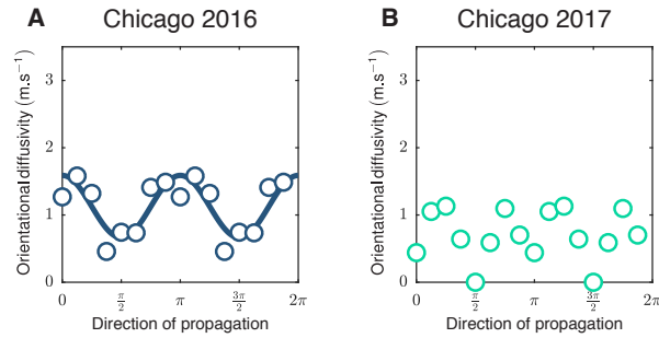
Figure 2.17 | Orientational diffusivity as a function of the direction of propagation. (A) Chicago 2016. (B) Chicago 2017.
