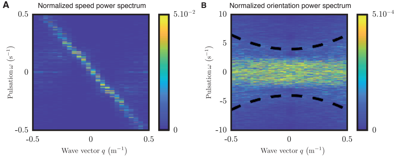
Figure 2.12 | Power spectra in the direction of the road normalized at every wave vector q . (A) Normalized speed power spectrum. (B) Normalized orientation power spectrum. Dashed-lines: visual guide for the spectral width increase as a quadratic function (main text Fig. 3h).
