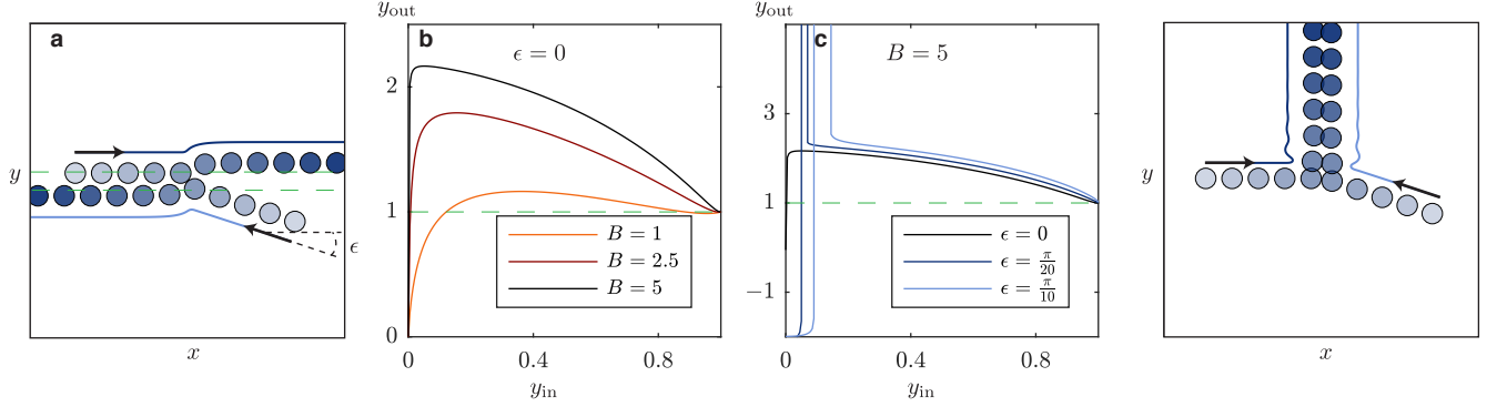
Figure 1.11 | Persistent transverse scattering. (a) Typical scattering trajectory for two particles targeting opposite directions ( B = 5 , \epsilon = \frac{\pi}{10} and y_{in} = 0.75 ). The initial and final vertical positions y_{in} and y_{out} are defined in the main text, Fig. 3a. \epsilon is the incoming deviation of the left mover. (b) Final vertical position y_{out} as a function of the initial vertical position y_{in} for a left and a right mover experiencing a frontal collision ( \epsilon = 0 ) at different values of the repulsion magnitude B . The transverse scattering is always different from the expected value for hard-core collisions (green line), and grows with the repulsion magnitude. (c) Final vertical position y_{out} as a function of the initial vertical position y_{in} at a high repulsion magnitude B = 5 for different impact angles \epsilon . At a sufficiently high impact angle, the particles can stick to each other and travel upwards or downwards, as pictured in (d). (d) Two particles travelling upwards together ( B = 5 , \epsilon = \frac{\pi}{10} and y_{in} = 0.125 )
