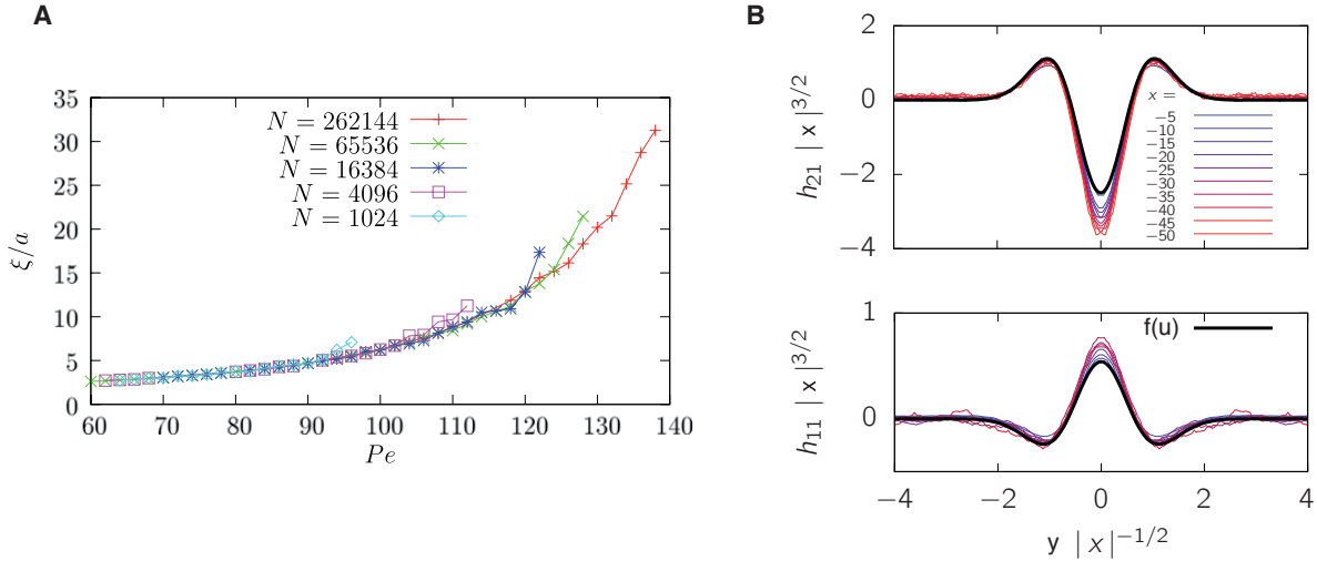
Figure 1.2 | Two key results emerge from the literature on passive systems. (A) Lane size \xi increases continuously with the driving force (the external drive is by definition proportional to the Peclet number Pe ). Adapted from [34]. (B) The density correlation function g(x, y) decays algebraically in the forcing direction, as x^{-3/2} in two dimensions. Here h(x, y) = [g(x, y) - 1] is numerically shown to rescale as x^{3/2}h(x, y) = f(yx^{-1/2}) , with f(u) a generic function, proving the long-range correlation [g(x, y) - 1] \propto x^{-3/2} . h_{11} and h_{21} respectively denote the correlations between particles travelling in the same and in opposite directions. Adapted from [76].
