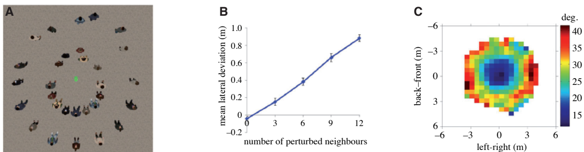
Figure 3 | Swarming experimental results (all adapted from [78]). (A) Participants (green dot) are immersed in two circles of virtual pedestrians. (B) The mean lateral deviation of participants increases linearly with the number of perturbed neighbors. (C) Spatial distribution of the mean absolute orientation difference between the central participant and the other participants in the human swarm.
