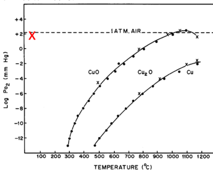
Figure I-12: Cu-O common pressure temperature phase diagram. X: standard conditions (from [18])
