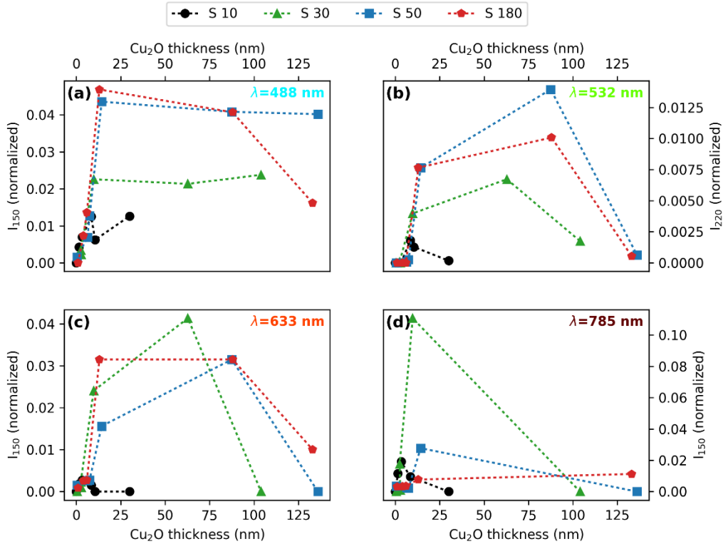
Figure IV-12: Raman peak intensity of \text{Cu}_2\text{O} as a function of \text{Cu}_2\text{O} thickness for excitation at 488 nm (a), 532 nm (b), 633 nm (c) and 785 nm (d)
