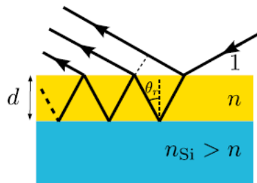
Figure I-38: Multiple refraction on a duplex system
