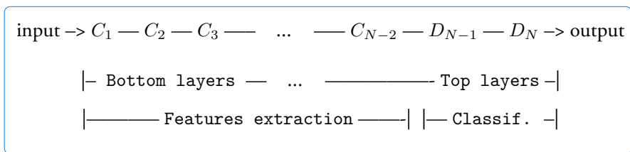
Figure 35 Schematic view of a CNN, with N_L layers including the convolutional layers C_i , with 1 \leq i \leq N_L - 2 (features extraction) and the dense layers D_{N_L-1} and D_{N_L} (classification).
