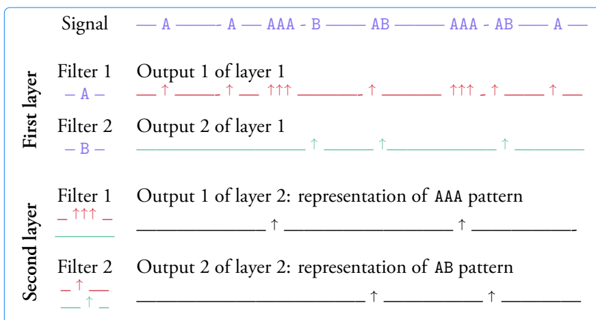
Figure 36 Schematic illustration of the effect of a CNN on a 1D signal.
