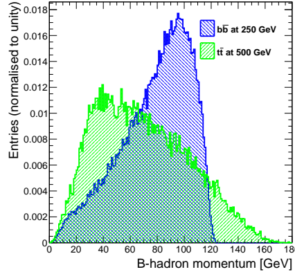
Figure 9.1: Generated b -hadron momentum by PYTHIA for b\bar{b} and t\bar{t} pair production processes signal processes.
