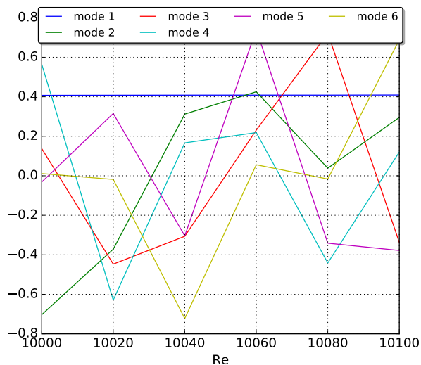
(a) First 6 Reynolds modes for Re \in [10000, 10100]
