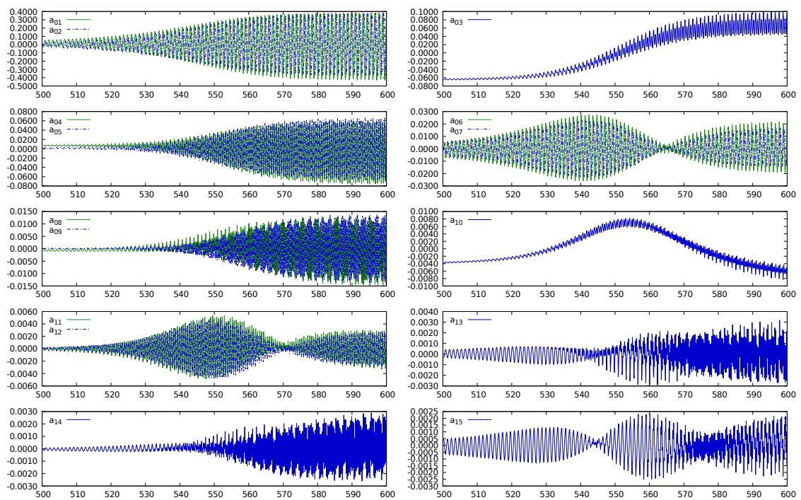
Fig. 8(b): Amplitude of POD modes and its FFT for Re = 10700 obtained for the (257 \times 257) grid for the point Q_2 in Fig. 2.
