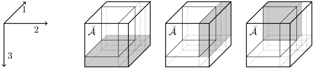
Figure 2.12: A visual of the truncated HOSVD, it shows that the approximation \check{\mathbf{A}} is defined simultaneously for each direction through least square approximation. Figure from [VVM12].
