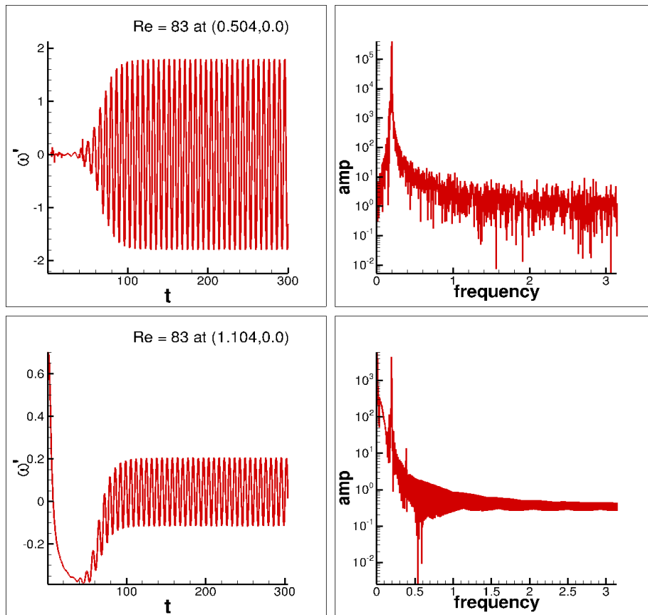
Figure 6.1: DNS time series and their associated DFT's are shown for (a) the flow inside a LDC and (b) the external flow past a cylinder, at indicated points in the flow. In (b), left frames are time series at different wake points and right frames are the associated spectra.
