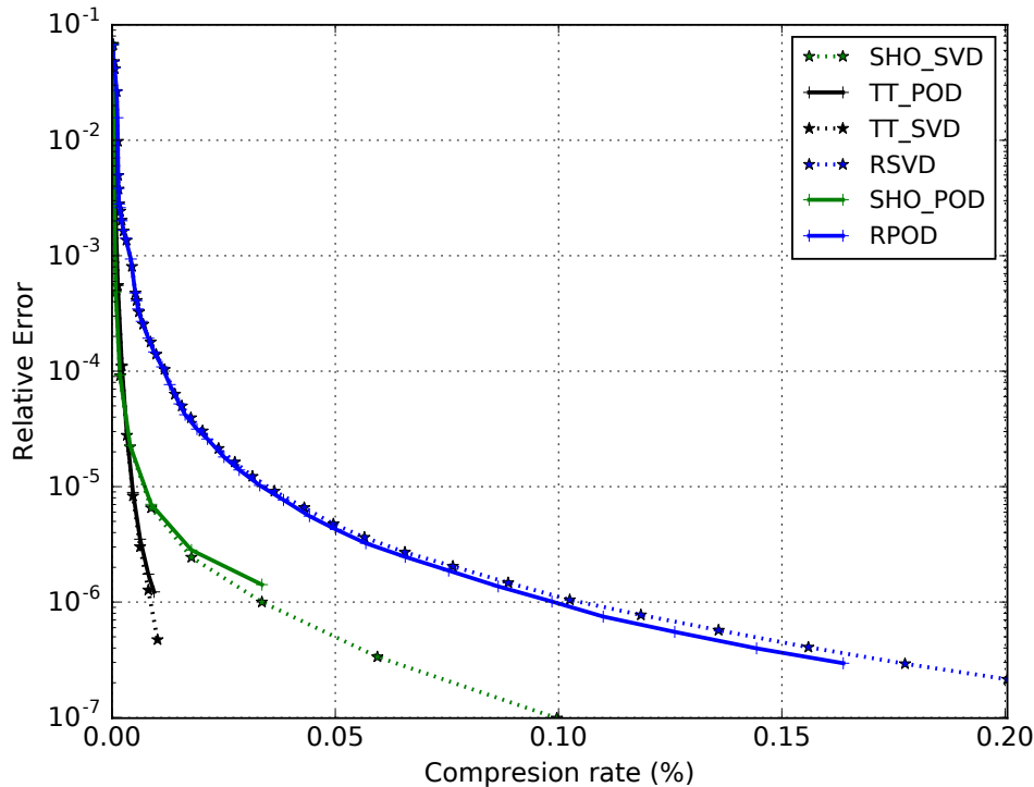
Figure 4.4: Decomposition of f_s on a 40^5 grid with L^2 and l^2 scalar products, decomposition error in their relative norm
