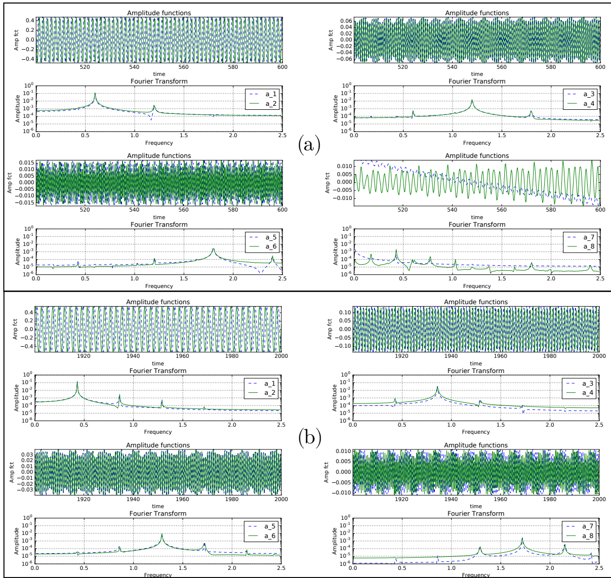
Figure 5.18: Amplitude of POD modes and its DFT for Re = 9800 using (257 \times 257) grid (a) before [t = 500 to 600] and (b) after [t = 1900 to 2000] the secondary instability, for the case of Fig. 5.17
