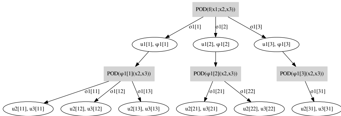
Figure 3.2: Example of a Recursive POD graph of f(x_1, x_2, x_3)
