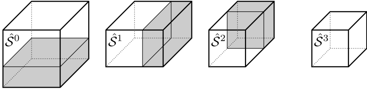
Figure 2.13: A visual of the sequentially truncated HOSVD with the same axis as figure 2.12. Here each approximated tensor \hat{\mathbf{S}}^i is performed on one dimension then a new tensor \hat{\mathbf{S}}^{i+1} is processed on the next direction. Processing order is (3,2,1). Figure from [VVM12].
