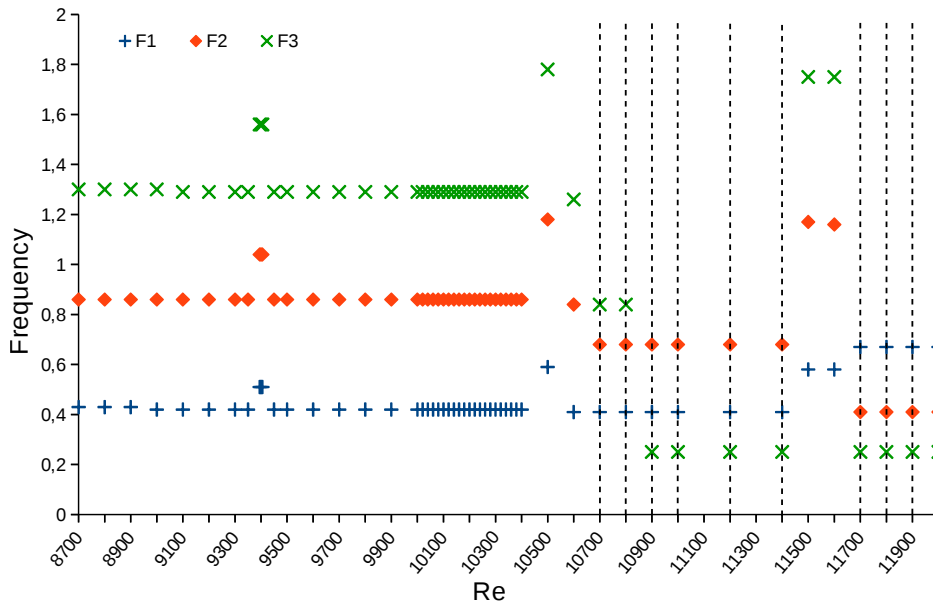
Figure 6.8: Frequency variation for Re = [8700, 12000] for the first three leading frequencies of the vorticity time series at point (0.95, 0.95) obtained for the last 50 periods. The dotted lines indicate the presence of multiple dominating peaks in the spectrum.
