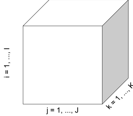
Figure 2.1: A third order tensor with \mathcal{T} \in \mathbb{R}^{I \times J \times K} .
