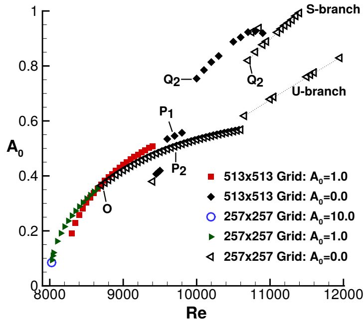
Figure 5.8: Variation of the equilibrium amplitude ( A_e ) with Reynolds number ( Re ) for the two grids, with ( 257 \times 257 ) and ( 513 \times 513 ) points. Note the points ( P_1 , P_2 ) and ( Q_1 , Q_2 ) have similar dynamics, as shown later. Additional points O and S represent the onset of unsteadiness ( Re = 8670 ) and secondary instability ( Re = 9800 ) of the flow field computed using ( 257 \times 257 ) grid points.
