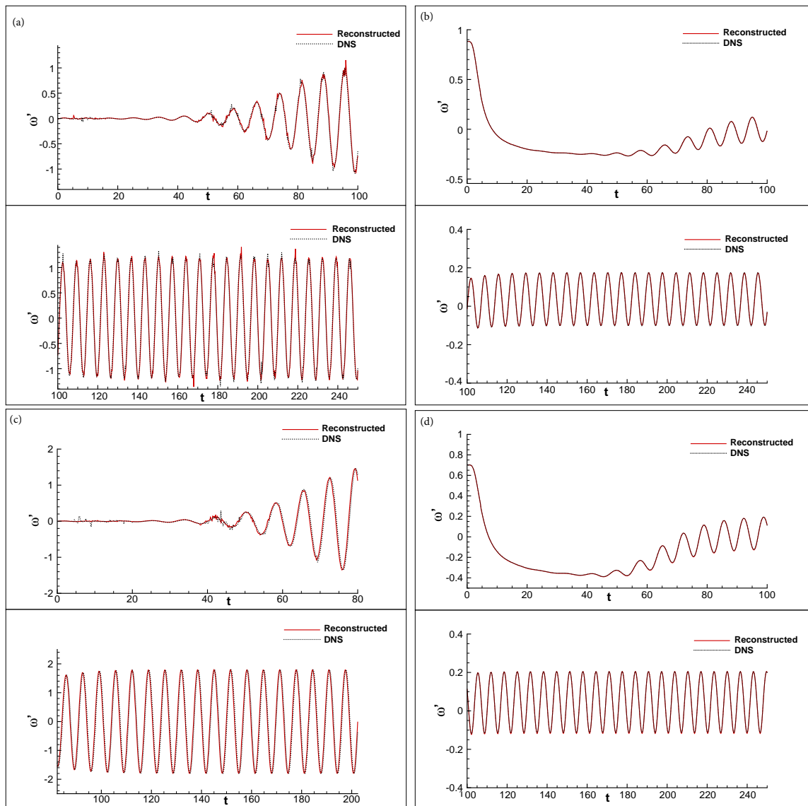
Figure 6.12: Reconstructed disturbance vorticity with time-scaling interpolation for (a) Re = 70 using Re = 68, 72, and 76 at (0.504, 0.0) , (b) at (1.104, 0.0) and (c) Re = 83 using Re = 78, 80, 86 and 90 at (0.504, 0.0) and (d) at (1.104, 0.0) . Within each subfigure, the top frame is for comparison at early times, while the bottom frame shows comparison at later times.
