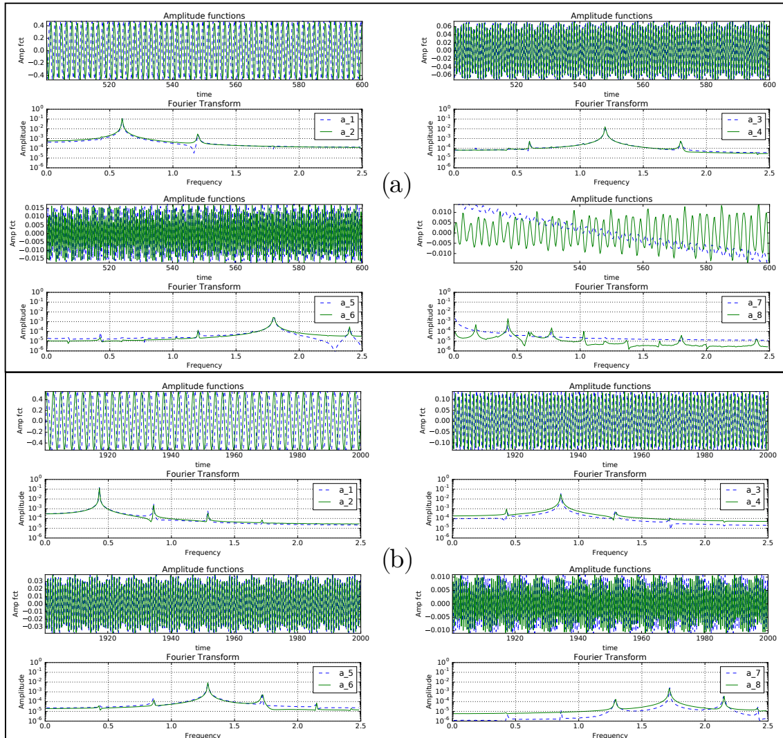
Fig. 10: Amplitude of POD modes and its DFT for Re = 9800 using (257 \times 257) grid (a) before [t = 500 \text{ to } 600] and (b) after [t = 1900 \text{ to } 2000] the secondary instability, for the case of Fig. 9.
