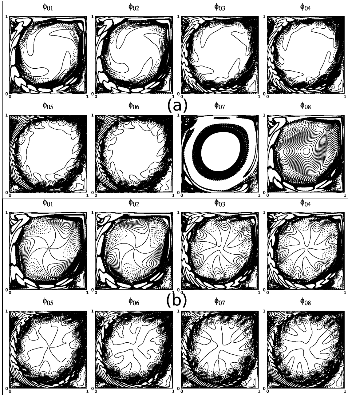
Fig. 9: Eigenfunctions of POD modes for Re = 9800 obtained with (257 \times 257) grid during (a) t = 500 to 600 before and during (b) t = 1900 to 2000 after the secondary instability.
