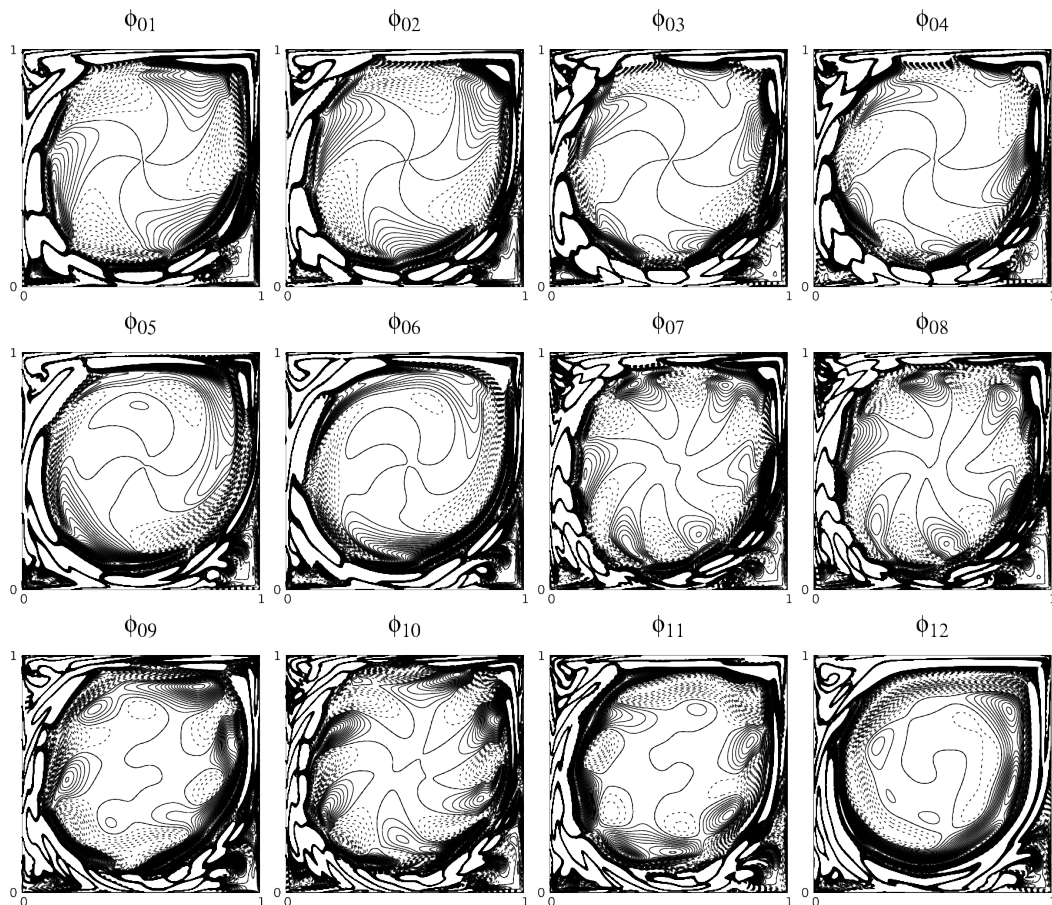
Figure 5.12: Eigenfunctions of POD modes at points Q_1 ( \text{Re}=10000 ) and Q_2 ( \text{Re}=10700 ). (\varphi_m)_m isolines are plotted in the [-0.5, 0.5] range with 0.01 spacing. Solid lines are positive values, while dashed lines are negative value contour.
