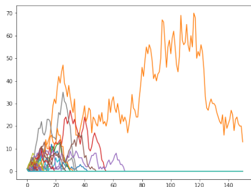
FIGURE 3.11 – Three-type process in fixed environment
