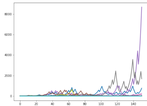
FIGURE 3.8 – Single-type process in random environment
