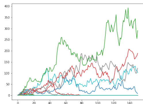
FIGURE 3.12 – Three-type process in random environment
