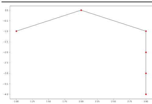
FIGURE 3.1 – Single-type process in fixed environment
