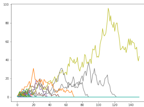
FIGURE 3.7 – Single-type process in fixed environment
