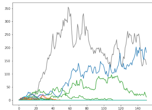
FIGURE 3.10 – Two-type process in random environment
