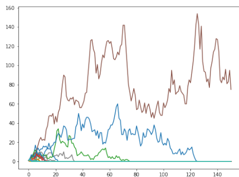
FIGURE 3.9 – Two-type process in fixed environment
