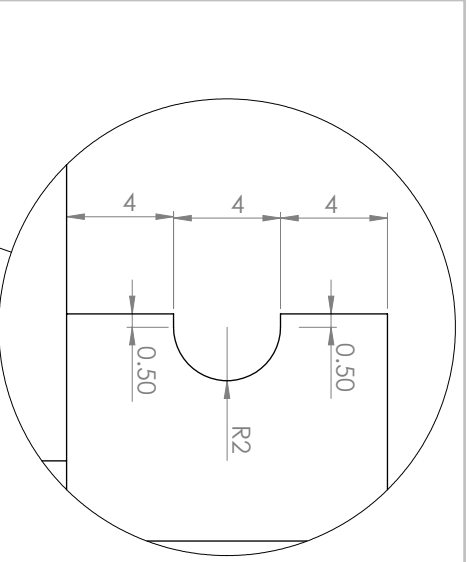
DETAIL F SCALE 5 : 1
