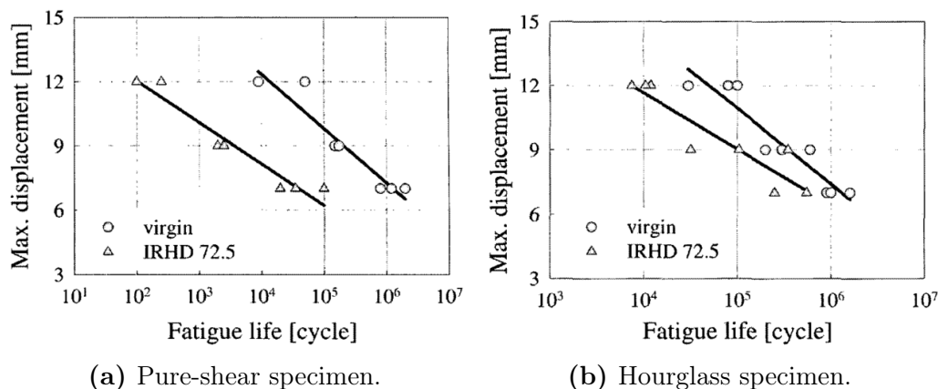
Figure 5.1-9 – Fatigue life of virgin and pre-aged (90 °C for about 192 h) natural rubber specimens (Choi et al. 2005).
