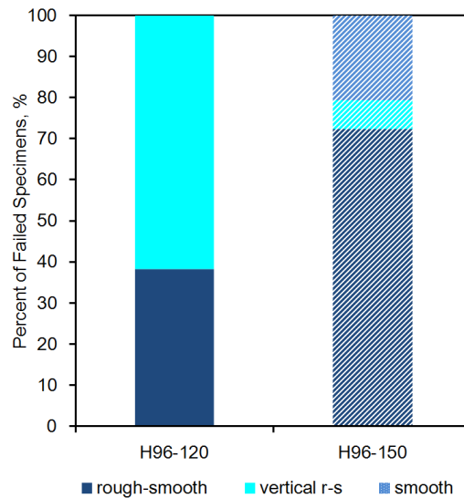
Figure 5.3-11 – Microscopic observations of fracture surfaces categories in broken specimens tested at 150 °C; hatched fill indicates partial sampling.
