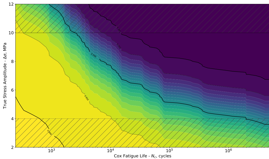
Figure 4.3-8 – Probabilistic Wöhler curve of A44H96 120°C estimated by Cox model. Hatched regions indicate extrapolated data.
