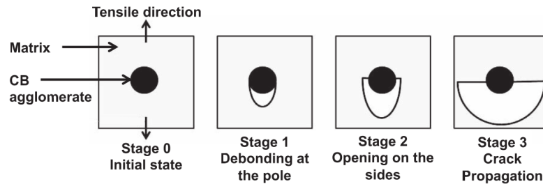
Figure 4.1-5 – Schematic representation of fatigue crack initiation mechanism around a CB agglomerate (Huneau et al. 2016).
