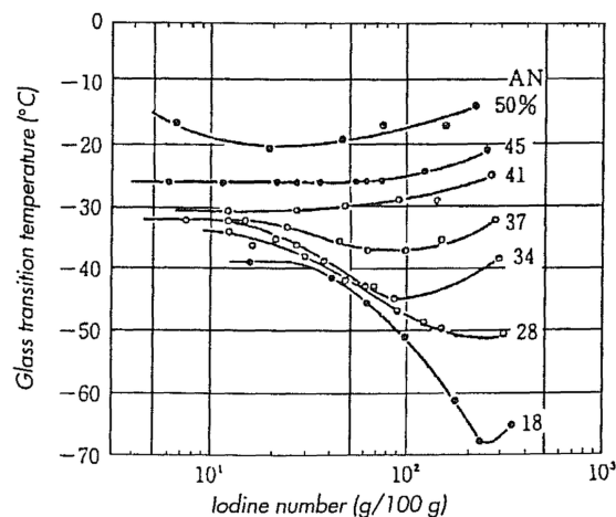
Figure 2.1-5 – Glass transition temperature with respect to iodine number (inverse of percent hydrogenation) and ACN content (Sawada 1993).
