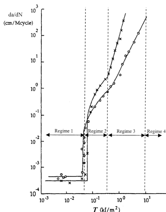
Figure 4.1-3 – Four regimes in fatigue crack propagation response of NR (×) and SBR (○); original figure from Lake and Lindley (1965) and modified by Mars and Fatemi (2002).
