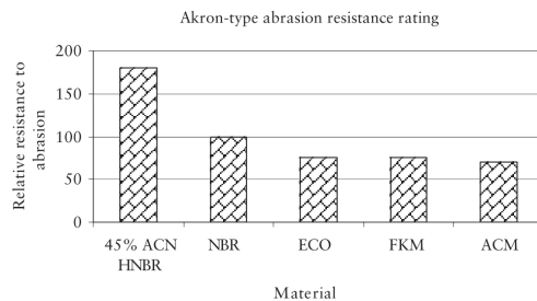
Figure 2.1-2 – Comparison of abrasion resistance of various elastomers with NBR as a reference (Keller 2012).
