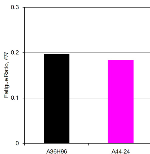
Figure 4.4-3 – Fatigue ratio of composite HNBR blend A44-24.
