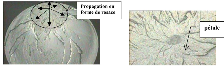
Figure 4.1-13 – Fracture surface of HNBR with N550 type of CB; left - \times 25 magnification with arrows indicating the direction of propagation of the cracks; right) \times 175 magnification of initiation and propagation regions with “petal” shaped cracks (Gauchet 2007).
