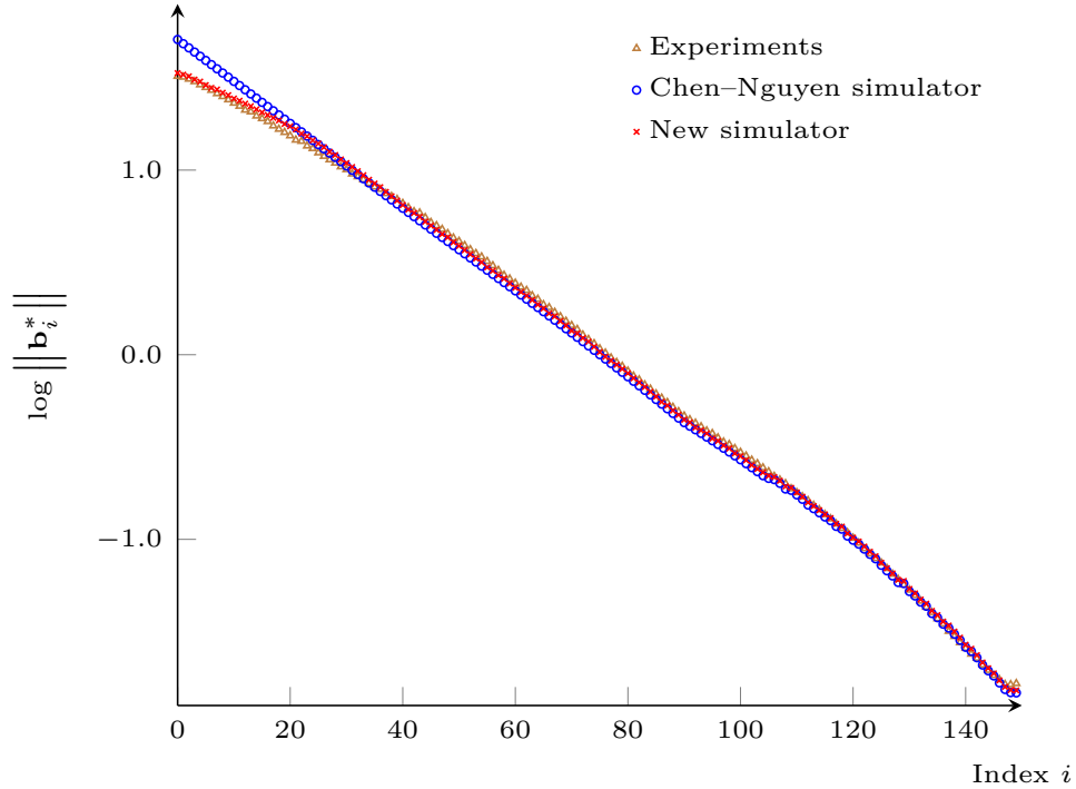
Fig. 5.21: Gram-Schmidt log-norms for \text{BKZ}_{60} at tour 20,000.
