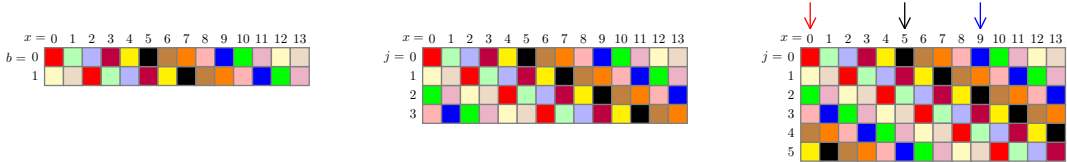
Fig. 4.1: An illustration of one-dimensional U-EDCP with number of possibilities 2, 4 and 6, and modulus 14.
