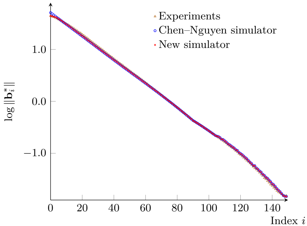
Fig. 5.19: Gram-Schmidt log-norms for BKZ_{60} at tour 50.
