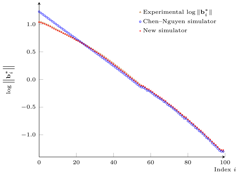
Fig. 5.17: Gram-Schmidt log-norms for BKZ_{45} at tour 2,000.
