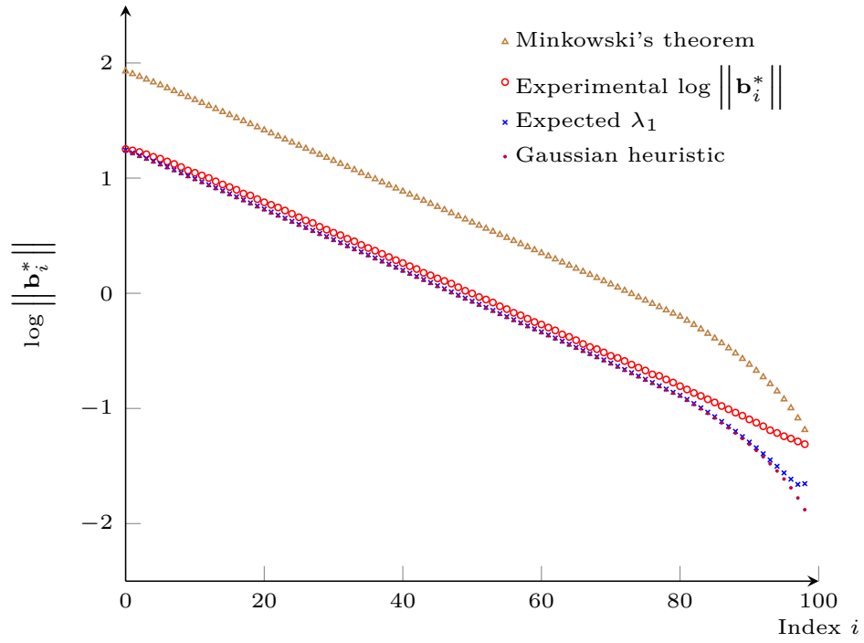
Fig. 5.6: Output of BKZ 20 .
