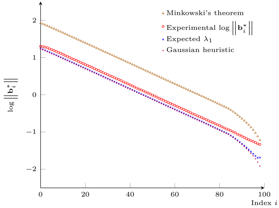
Fig. 5.5: Output of BKZ 16 .
