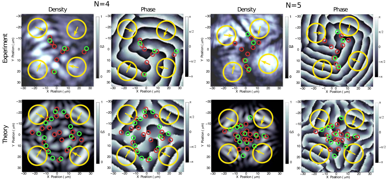
FIG. 2. Experimental (top) and theoretical (bottom) density and phase maps for \theta = 3.5^\circ , \varphi = 21^\circ [ L = 4.0(5) ], and \varphi = 26^\circ [ L = 4.9(6) ] in the low density regime. An interference pattern is visible together with phase singularities of both signs. Since the injected angular momentum is not zero, the number of (+) singularities (red circles) is different from the number of (-) singularities (green circles).
