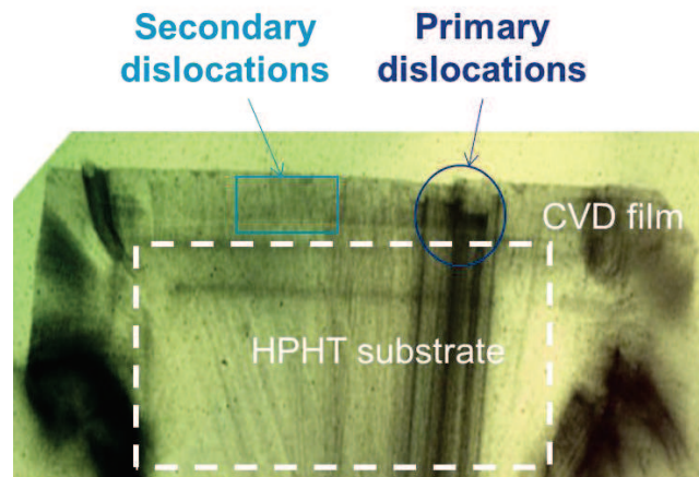
XRT image, Courtesy M. Kasu, Saga University
