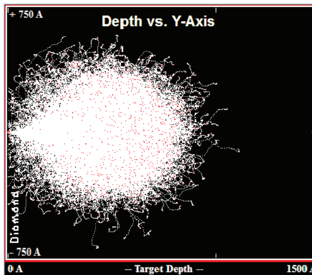
Figure IV.10. SRIM simulations for a model of 10^4 helium ions fired up into a diamond target with energy of 10 keV showing the ion path
