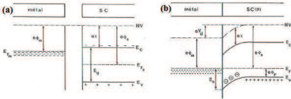
Figure I.20 Metal-semiconductor junction with \Phi_m < \Phi_s (a) before and (b) after the contact at the thermodynamic equilibrium [105].
