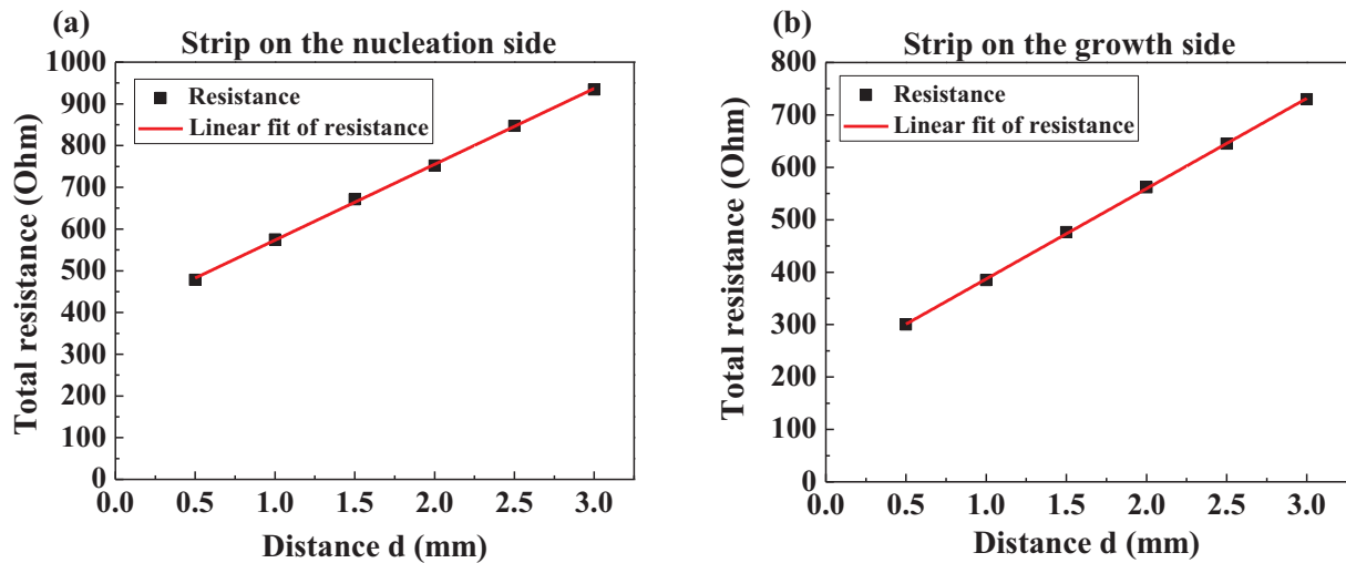
Figure III.14 Plots of the total resistance R_T against the distance d between the probes extrapolated from the I-V curves shown in Figure III.13 for the corresponding strips ((a) on the nucleation side and (b) on the growth one).
