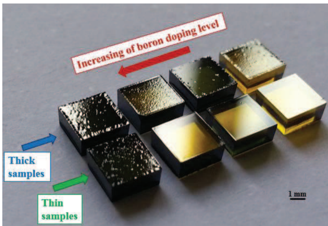
Figure IV.1. Picture of the set of diamond samples as-grown. In the first column on the left two samples with the same boron doping of 12000 ppm (B/C)_{\text{gas}} but different thickness (the thicker films on the top and the thinner ones on the bottom) are presented. Similarly, the second and third columns are arranged for the doping levels of 6000, 3000 ppm (B/C)_{\text{gas phase}} . Finally, in the fourth and last column the NID and intrinsic diamonds are placed on the top and bottom row, respectively.
