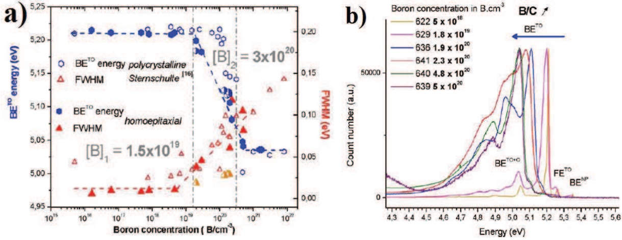
Figure IV.5. (a) Evolution of the BE TO peak energy (left axes) and FWHM (right axes) against the boron concentration for diamond samples with different boron doping level. Full, empty and mixed symbols indicate monocrystalline, polycrystalline or other samples, respectively [226]. (b) Cathodoluminescence spectra registered on CVD monocrystalline boron doped diamonds with different doping levels [226].
