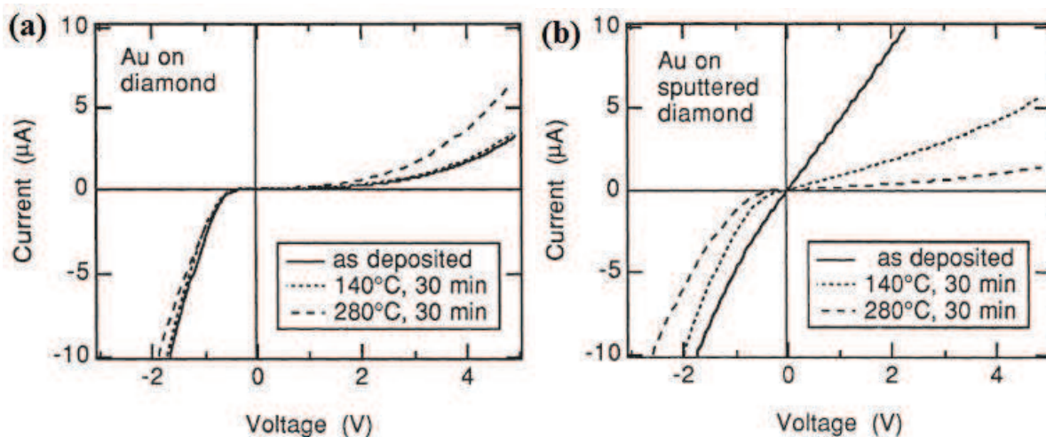
Figure I.22. I-V characteristics of Au contacts on (a) as-grown and (b) sputtered polycrystalline boron doped diamond surface [119].
