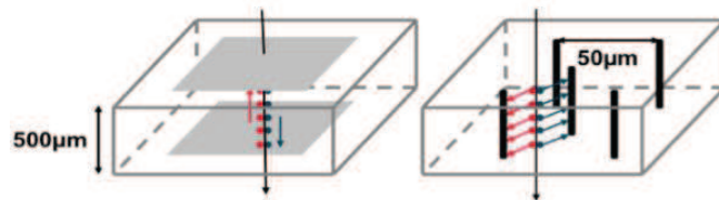
Figure I.31. Sketch of a planar (on the left) and 3D (on the right) electrode configuration for solid-state detectors. The drift distance of the carriers decrease by using a 3D electrode configuration [159].
