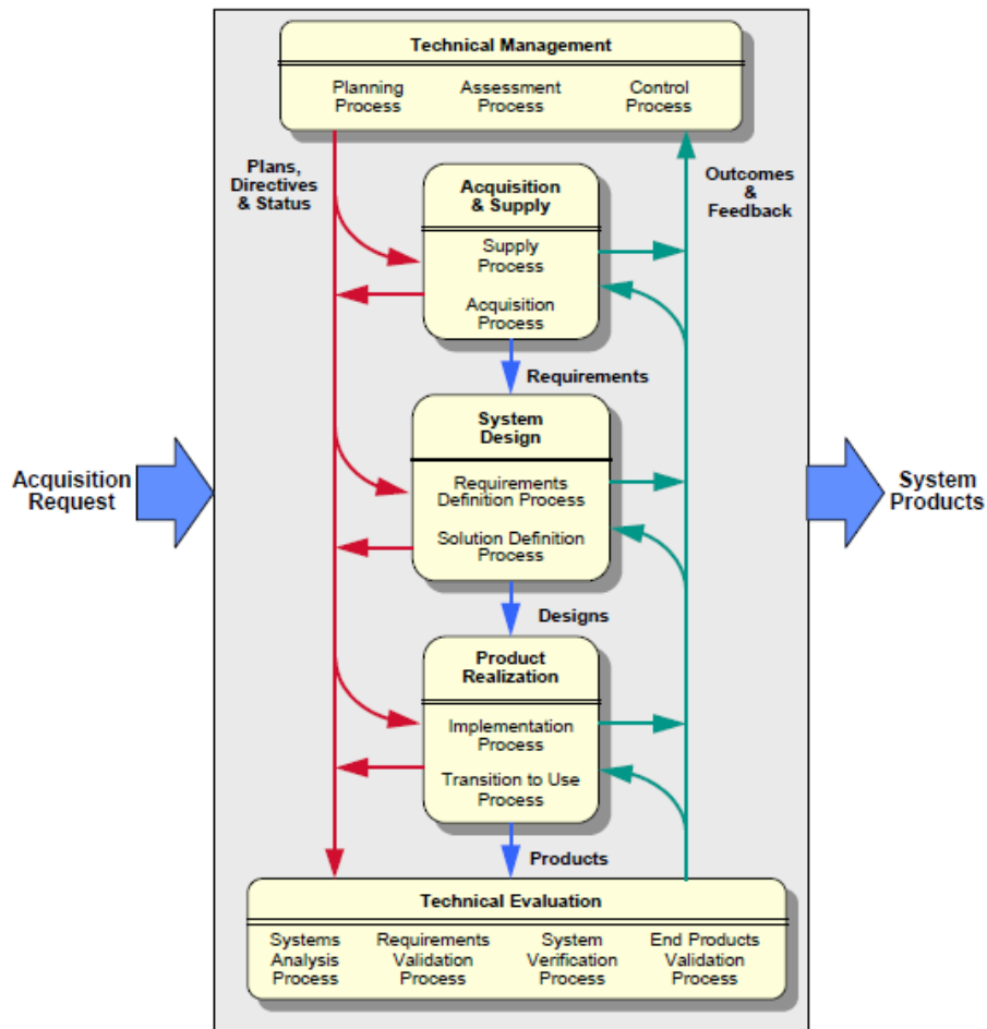
Figure 4a—Relationship of processes for engineering a system
