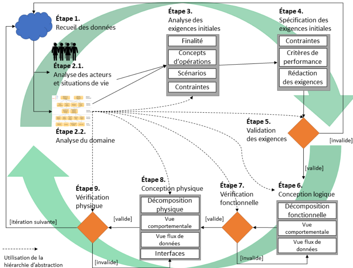
FIGURE 1.2 – Méthode IS+WDA
