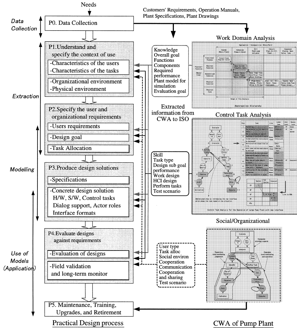
Figure 1. Relationship between CWA, ISO13407 design processes, and practical design processes.
