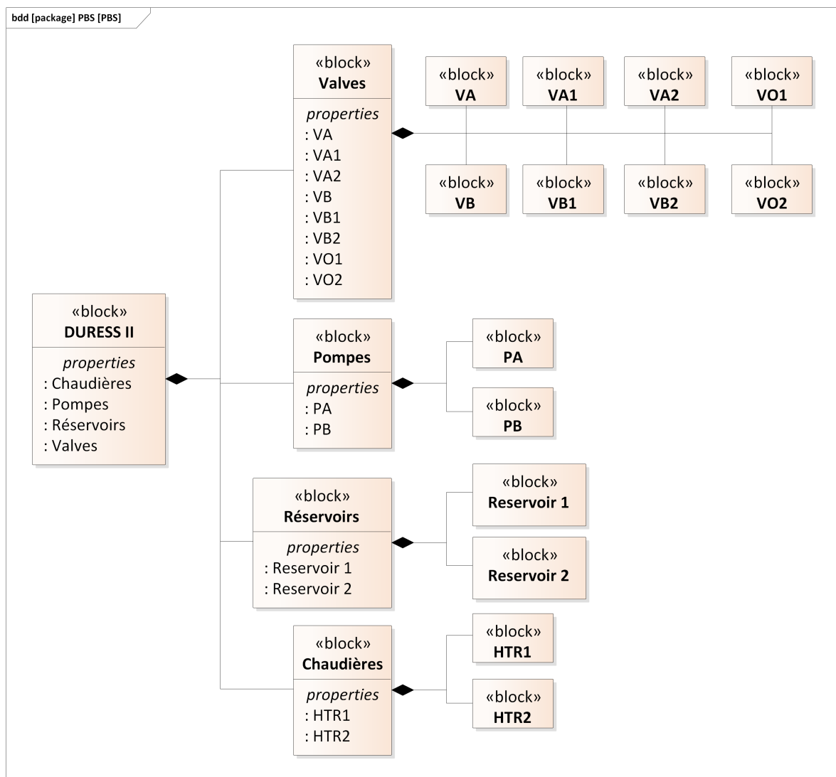
FIGURE 2.12 – Le PBS de DURESS II
