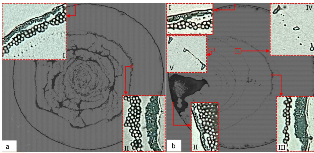
Figure 5.16 Dried deposits of bidispersed drops containing a mixture of 3.2 \mu\text{m} diameter particles (mass concentration of 0.0125 wt %) and 1 \mu\text{m} diameter particles (mass concentration of 0.0125 wt %) onto a heated substrate at temperature of 99 \text{ }^\circ\text{C} : (a) the rose-like pattern: (I) initial contact line, and (II) the second deposition line. (b) The typical stick-slip pattern: (I) initial contact line on the depinned side, (II) initial contact line on the pinned side, (III) the second deposition line, (IV) the third deposition line, and (V) the fourth deposition line. Insets show the zoomed-in regions highlighted in the solid rectangles. Scale bars, 600 \mu\text{m} .
