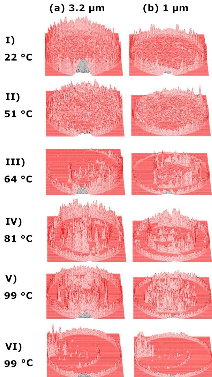
Figure A.4 Topography of the particle deposits at various temperatures: (a) Particle size of 3.2 \mu\text{m} , (b) Particle size of 1 \mu\text{m} .
