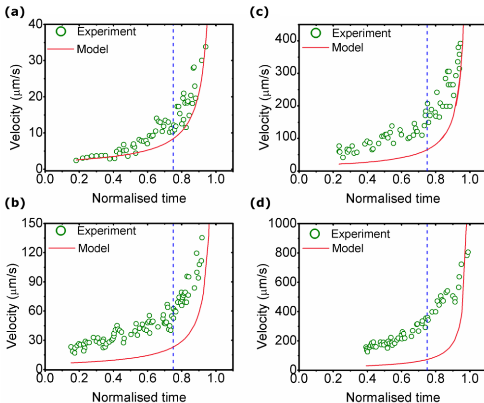
Figure 5.18 Particle velocity versus normalised time for drying bidispersed drops containing a mixture of 3.2 \mu\text{m} diameter particles (mass concentration of 0.0125 wt %) and 1 \mu\text{m} mean diameter particles (mass concentration of 0.0125 wt %) onto heated substrates at: (a) 22^\circ\text{C} , (b) 51^\circ\text{C} , (c) 64^\circ\text{C} , and (d) 81^\circ\text{C} . The dashed line indicates the start of the rush-hour behaviour.
