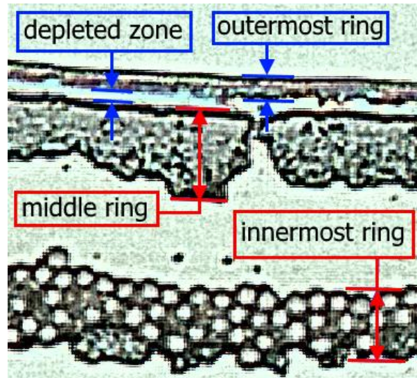
Figure 5.3 Zoomed-in picture ( 2\times ) of a completely dried water-based bidispersed drop containing a mixture of 3.2\ \mu\text{m} diameter particles (mass concentration of 0.0125 wt %) and 1\ \mu\text{m} mean diameter particles (mass concentration of 0.0125 wt %) onto a non-heated silicon substrate (at 22\ ^\circ\text{C} ). The complete evaporation of the thin liquid film leaves a depleted zone between the leading edge of the middle and outermost rings. The original micrograph is taken at magnification of 1000\times .
