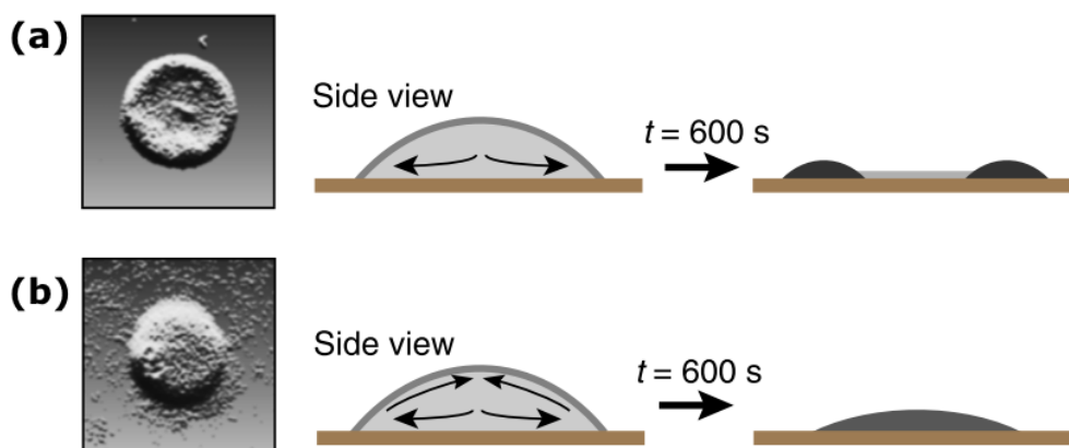
Figure 2.33 A coffee-ring pattern was formed without biosurfactants due to the coffee-ring effect. (b) A uniform pattern was formed with biosurfactants due to the strong Marangoni flow. Image taken from Ref. [68].
