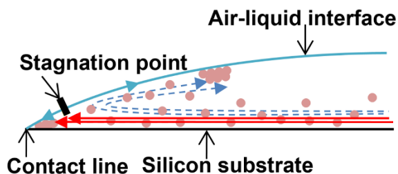
Figure 3.16. Schematic description of the flow pattern inside an evaporating water droplet containing CuO nanoparticles placed on a heated silicon substrate; the solid and dashed arrows indicate the outward capillary and thermally driven Marangoni flows, respectively. The black bar in the picture indicates a stagnation point where the direction change of the surface flow occurs.
