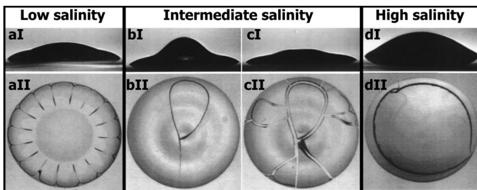
Figure 2.15 Influence of salt content on crack patterns from drying colloidal drops. (a) A regular radial crack pattern at low salinity. (b,c) A disordered crack pattern at intermediate salinity. (d) A circular crack pattern at high salinity. Side view of drops taken at: (aI) 15 min after deposition, (bI) 15 min after deposition, (cI) 20 min after deposition, and (dI) 15 min after deposition. Top view of drops taken at: (aII) 20 min after deposition, (bII) 20 min after deposition, (cII) 22 min after deposition, and (dII) 21 min after deposition. Image modified from Ref. [103].
