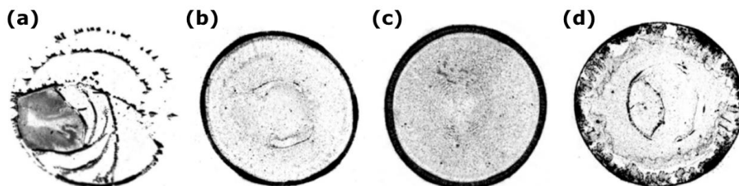
Figure 2.29 Influence of reduced environmental pressure on the pattern formation of a sessile \text{SiO}_2 nanofluid drop: (a) 750 mbar, (b) 500 mbar, (c) 250 mbar, and (d) 100 mbar. Image modified from Ref. [25].
