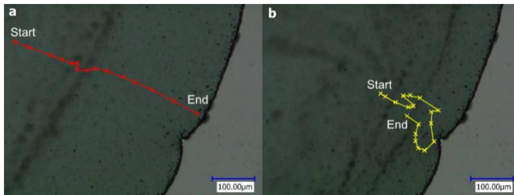
Figure 3.14. 500 \times still images of a water droplet containing 0.05 wt % CuO nanoparticles deposited onto a heated silicon substrate at 99 ^{\circ} C: (a) The line shows a tracer nanoparticle which moves towards the edge and deposit near the edge; the start and end points of the movement are at evaporation times of 0.08 and 0.68 s, respectively. (b) The line shows the movement direction of a specific nanoparticle cluster which circulates in the region very close to the edge; the start and final evaporation time of the movement are at 0.2 and 0.52 s, respectively. The optical micrographs are recorded at a temporal resolution of 60 fps and at 500 \times magnification. The scale bar is 100 \mu m.
