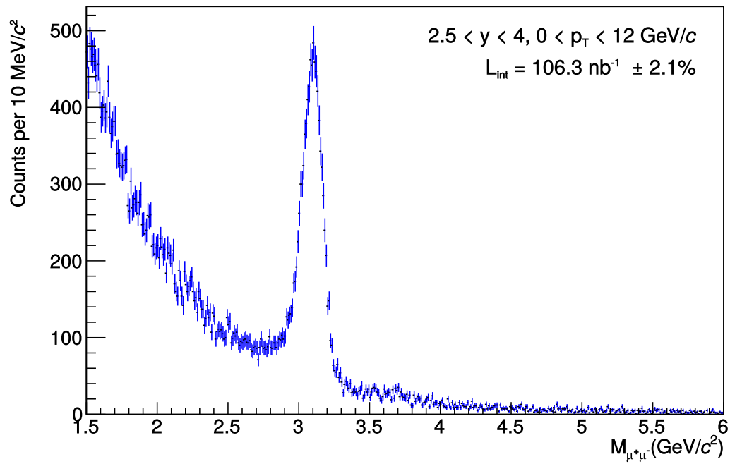
Figure 6.2: The dimuon invariant mass spectrum in pp collisions at \sqrt{s} = 5.02 TeV.
