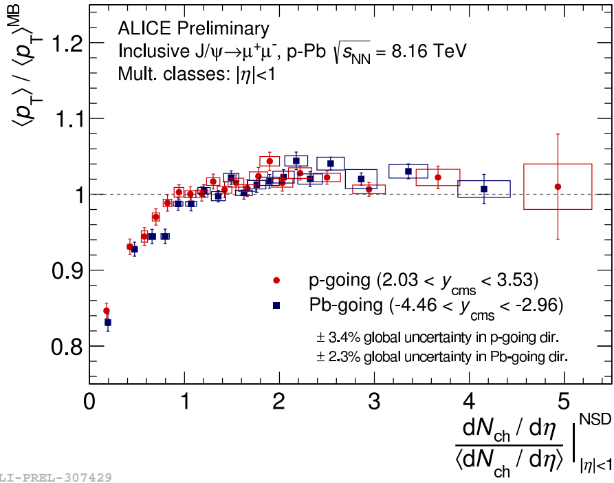
Figure 8.8: Multiplicity dependent \langle p_T \rangle^R results.
