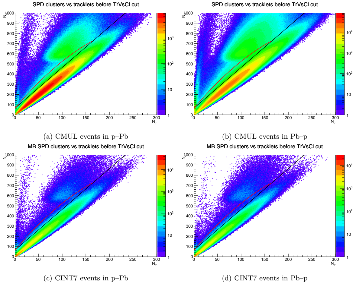
Figure 7.2: N_{CL} versus N_{tr} SPD pile-up cut. The black line represents Eq. (7.4) and red line the alternative polynomial form proposed in Eq. (7.2.1.2) for the intermediate tracklet range.
