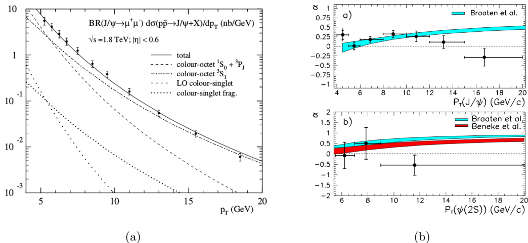
Figure 2.6: (a) p_T dependence of direct J/\psi production in p\bar{p} collisions at \sqrt{s} = 1.8 TeV at the Tevatron [45]. Visualised are colour singlet, colour octet and total contributions. Figure taken from [46]. (b) Polarisation of prompt J/\psi (top) and \psi(2S) (bottom) from 1.8 TeV p\bar{p} collisions at the Tevatron. The coloured bands show different NRQCD predictions [48, 49]. Figure taken from [47].
