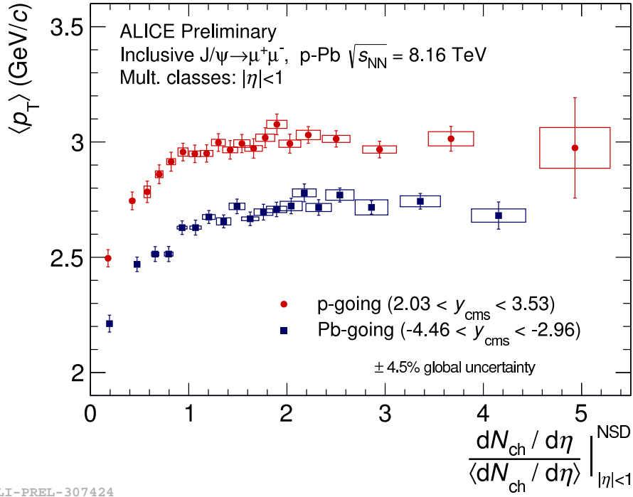
Figure 8.7: Multiplicity dependent \langle p_T \rangle results.
