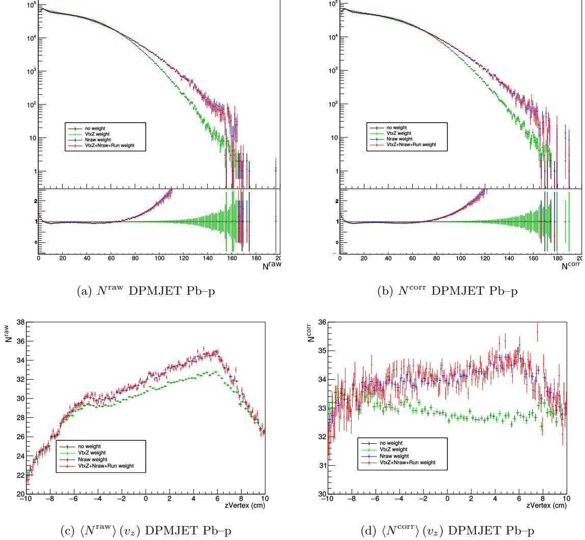
Figure 7.18: Effect of run, z -vertex and N^{\text{raw}} weights on tracklets distributions and profiles. Example shows DPMJET Pb-p. Note that black (no weight) points are hidden below the green ( z -vertex weight) ones. Top row shows the N^{\text{raw}} (left) and N^{\text{corr}} distributions, the respective bottom panels show the ratio of the weighted distributions with respect to the unweighted one. Bottom row shows the \langle N^{\text{raw}} \rangle (v_z) (left) and \langle N^{\text{corr}} \rangle (v_z) (right).
