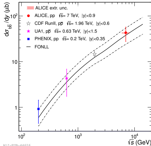
Figure 2.3: The energy dependence of the d\sigma_{b\bar{b}}/dy production cross section. Taken from [37].
