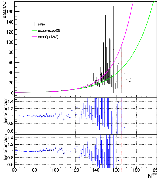
(c) EPOS p-Pb
