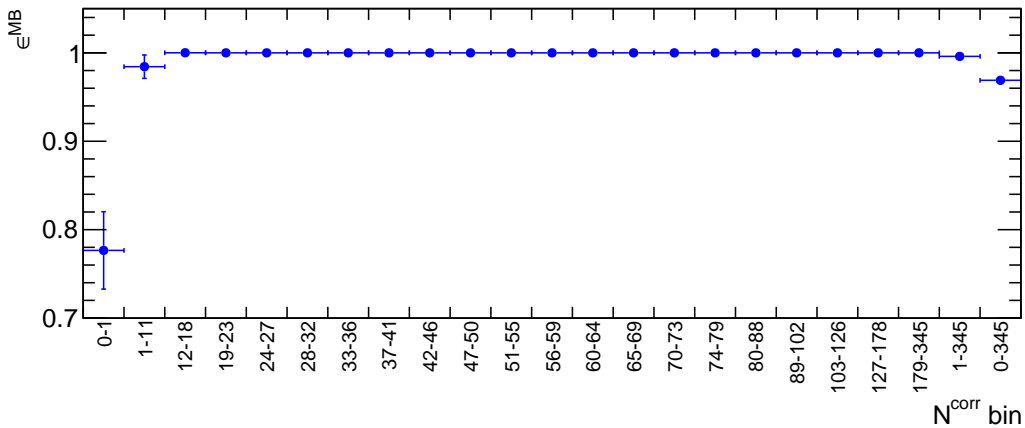
Figure 7.35: Multiplicity dependent vertex finding NSD event selection efficiency in Pb-p.
