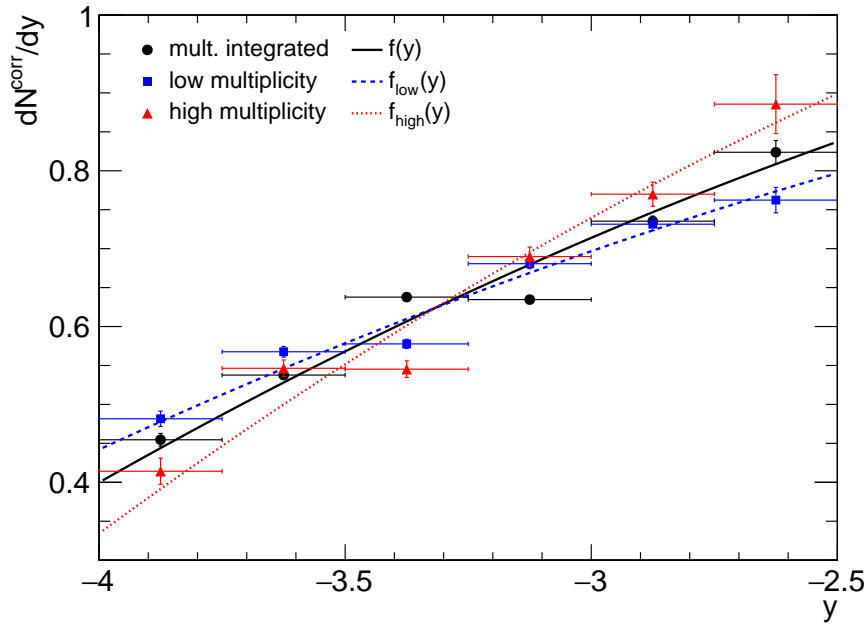
(b) y differential
