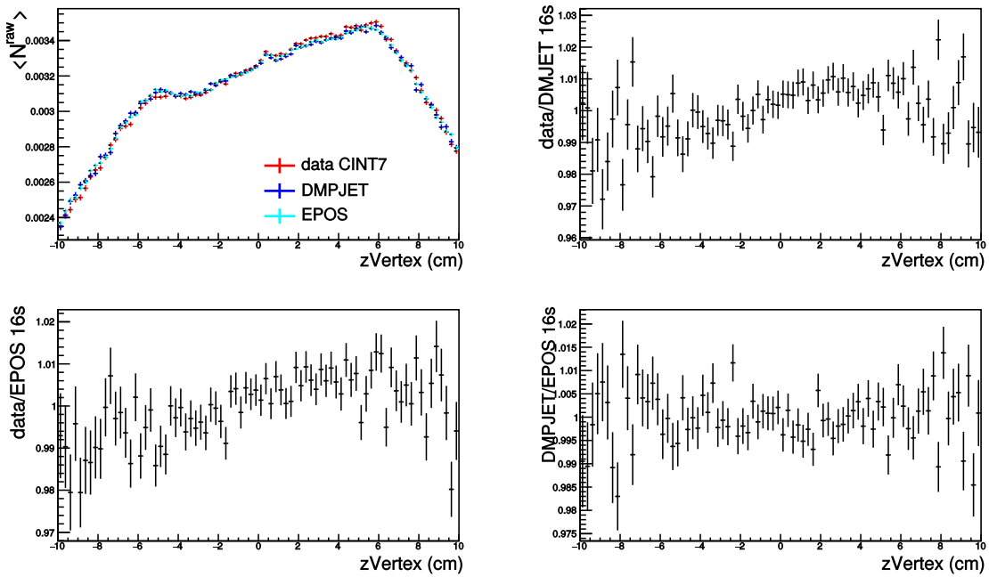
Figure 7.12: Same as Fig. 7.11 but for Pb-p period.
