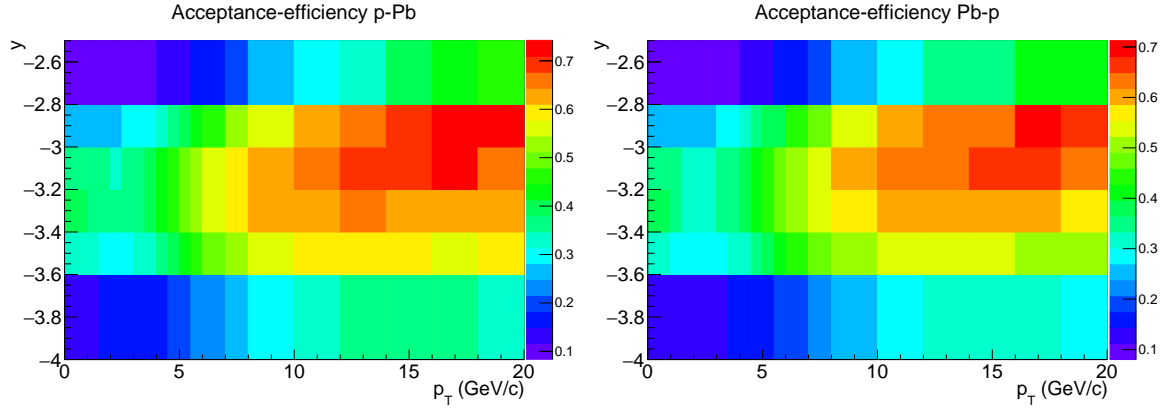
Figure 8.1: Double differential A\varepsilon(p_T, y) of the Muon Spectrometer in p-Pb and Pb-p at \sqrt{s_{\text{NN}}} = 8.16 TeV.
