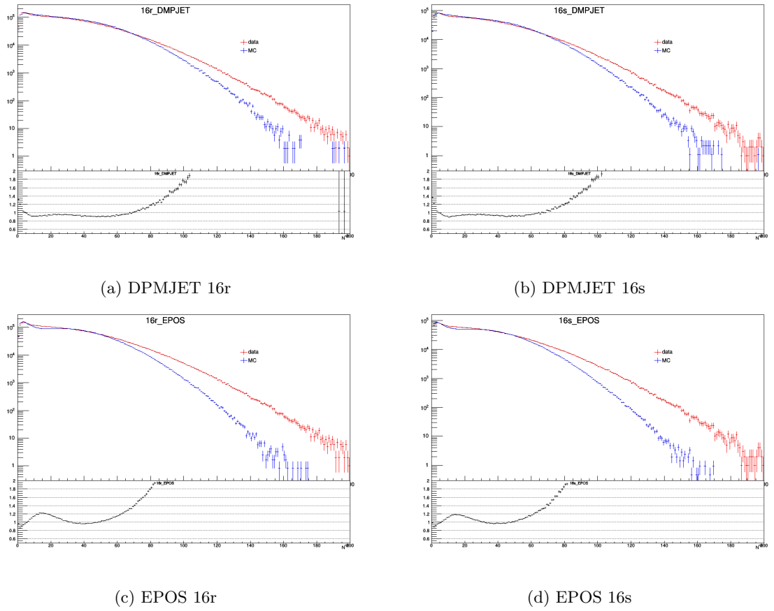
Figure D.4: Comparison of N^{\text{raw}} distribution between data and DPMJET or EPOS. Bottom panels show the ratio data/MC.
