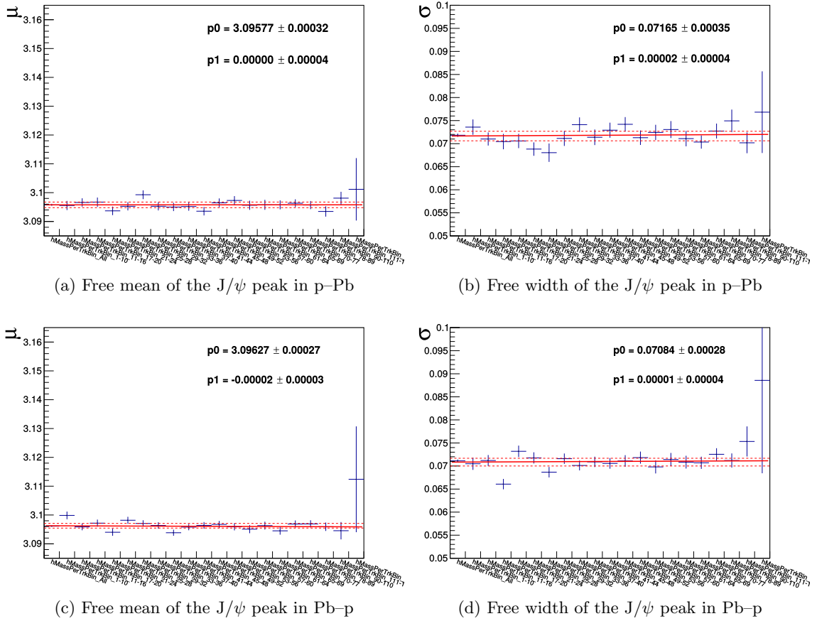
Figure 7.29: Values of free J/\psi mean and width in multiplicity bins.
