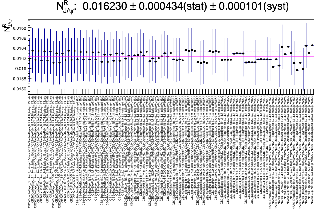
Figure 7.30: Relative N_{J/\psi} in the Pb–p period. The example show the one-but-last bin 127 < N^{\text{corr}} < 179 .
