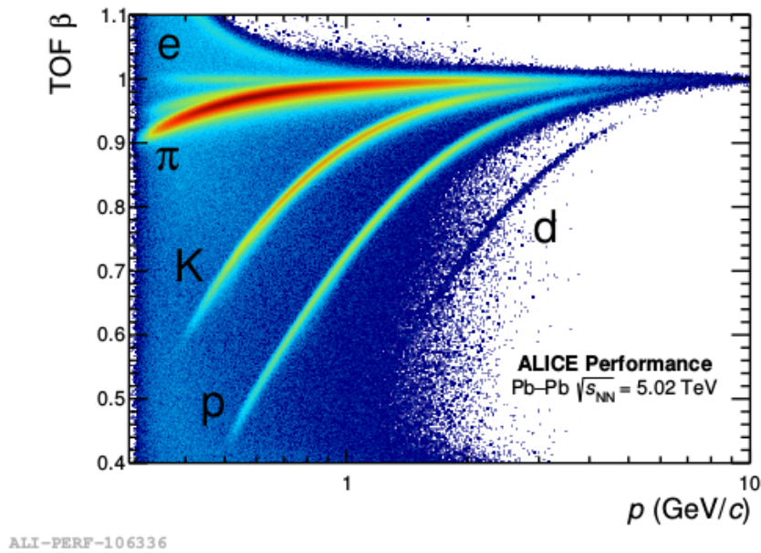
Figure 4.6: The TOF velocity \beta as a function of momentum in Pb–Pb collisions at \sqrt{s_{\text{NN}}} = 5.02\text{ TeV} . Taken from the ALICE Figure Repository [196].
