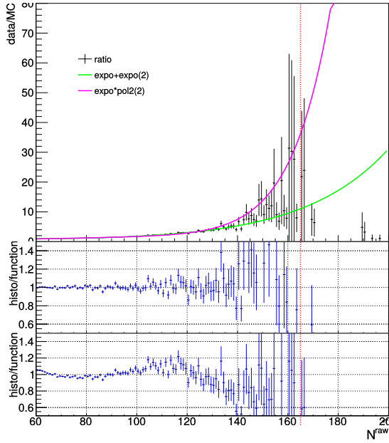
(a) DPMJET p-Pb
