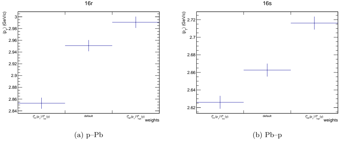
Figure 8.6: Spread of \langle p_T \rangle computed with different weight combination for the (a) p-Pb and (b) Pb-p data. Left is f_{low}^R(p_T) \cdot f_{low}^R(y) , centre is the default result, and on right is f_{high}^R(p_T) \cdot f_{high}^R(y) .
