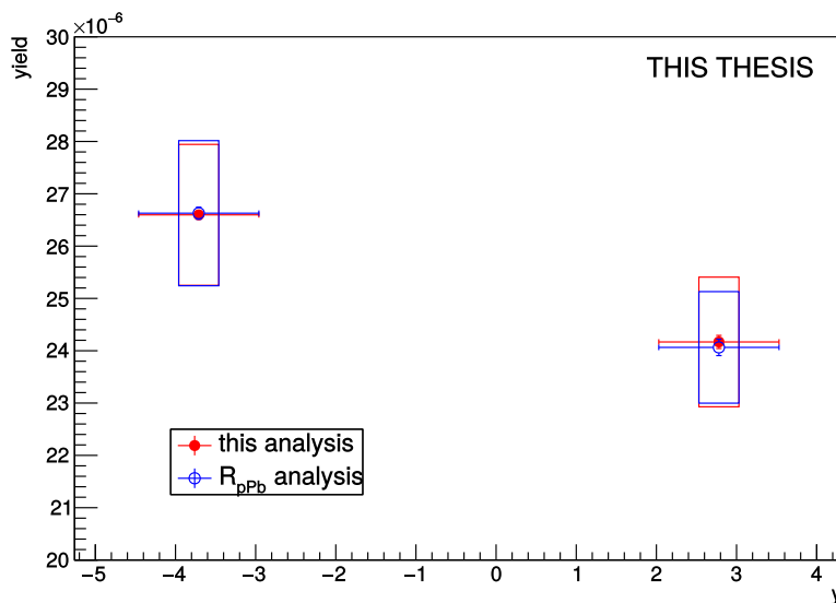
Figure 7.44: Multiplicity integrated invariant J/\psi yields in p-Pb and Pb-p at \sqrt{s_{\text{NN}}} = 8.16 TeV. Full discs show results of this multiplicity analysis, open circles denote results from R_{pPb} analysis [239].
