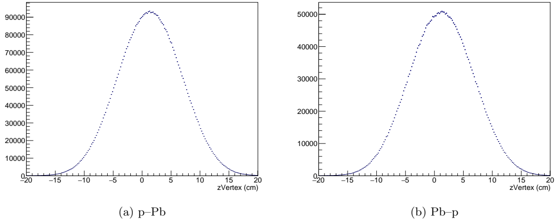
Figure 7.5: The z -coordinate of the SPD vertex in p-Pb and Pb-p. The maximum of the distribution is shifted in both period with respect to the nominal interaction point.
