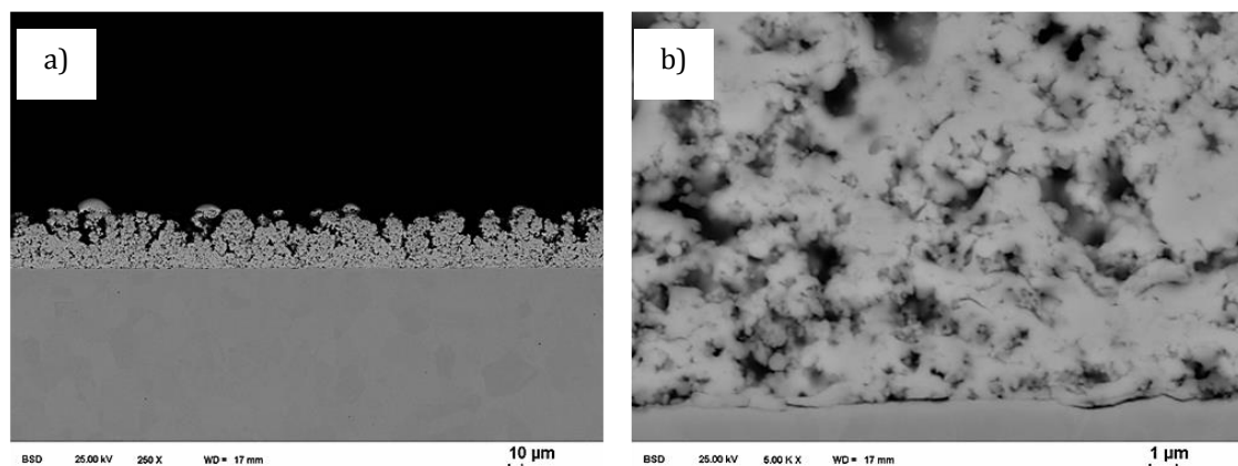
Fig. 4. SEM microstructure (backscattered electrons) of ST23 coatings under magnification of 2509 (a) and 50009 (b) 5). It was possible to observe that finer grains occurred near to the substrate. The top of the coatings consisted of a few very big grains which were very different comparing to the rest of the coating microstructure. These grains could have been formed by a few drop-lets of the suspension which leaked out from the injector and fell at the top of a hot sample at the end of the spray process. Three different pole figures {001}, {011} and {111} were composed to observe the main crystallite directions. The differences between these orientations were very small and it was not possible to distinguish any preferred directions of columns growth. The main volume grain size was near 600 nm - almost two times bigger than the initial powder particle size. However, the main number grain was of 300 nm and below, which was close to initial particle powder size.
