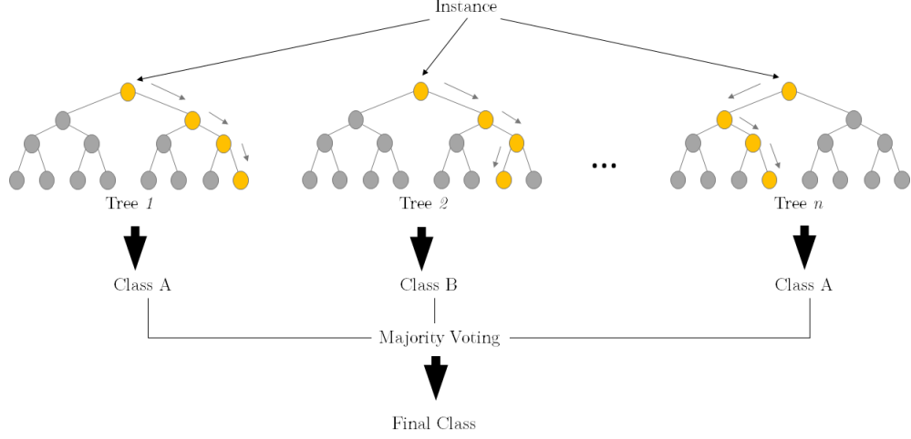
Figure 6.5: RF Classification
