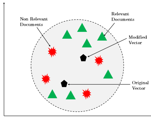
Figure 6.2: ROCCHIO Classification
