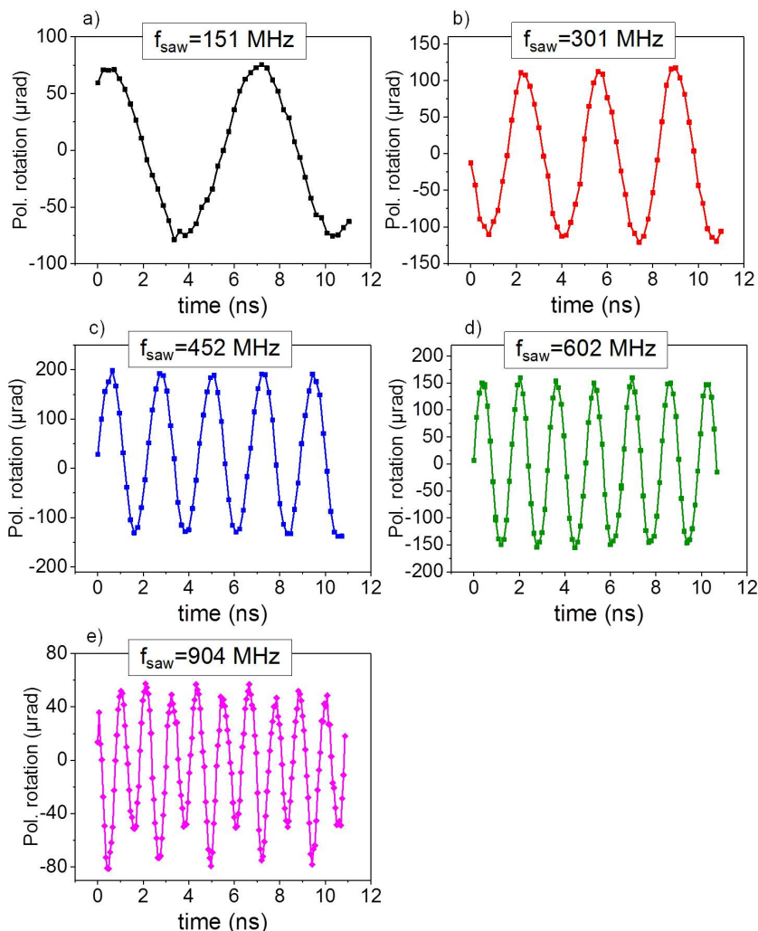
Figure 6.10.: Polarization rotation signal measured as a function of the optical delay for five SAW excitation frequencies (a) - (d). The signal was taken with a magnetic field \mu_0 H = 19.5 \text{ mT} applied along the hard axis at a temperature of T = 60 \text{ K} . (e) f_{\text{SAW}} = 904 \text{ MHz} . This frequency was measured at T = 90 \text{ K} and with \mu_0 H = 0.7 \text{ mT} . The second frequency in (e) is very possible due to the presence of 452 and 904 MHz in the excitation signal.
