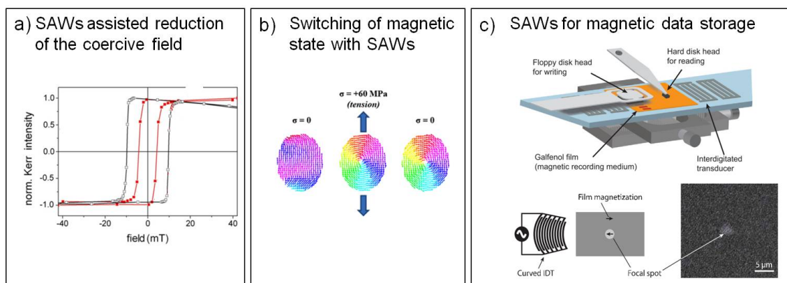
Figure 4.2.: a) Hysteresis cycles with and without SAW for GaMnAs [98]. b) Micromagnetic simulation of a nanomagnet state under the tensile dynamic strain [100]. c) Schematic of the device for magnetic data storage. Data will be recorded with the assistance of the SAW [99]
