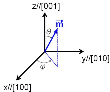
Figure 1.2.: Location of magnetization in polar coordinates system.
