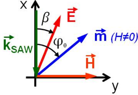
Figure 6.11.: Coordinate system for polarization rotation measurements.
