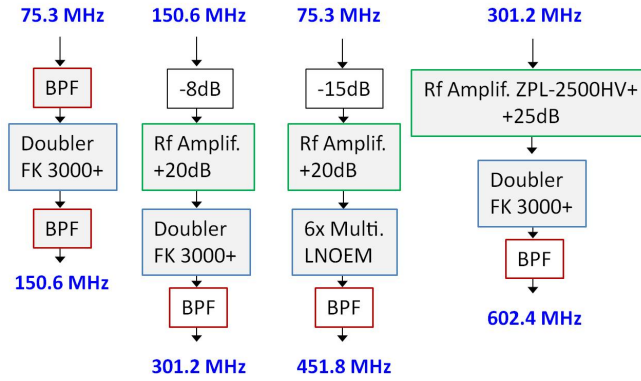
Figure 6.2.: RF connections for generation of harmonic frequencies of the laser repetition rate. RF amplifiers were used because the multipliers required a very specific RF input power. They may also introduced other harmonics, that is why a band-pass filter (BPF) was placed at the output.
