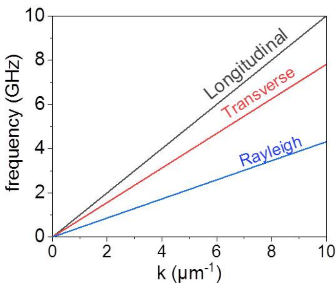
Figure 2.4.: The dispersion of longitudinal, transverse and Rayleigh waves for GaAs.
