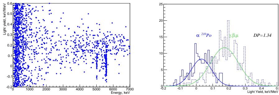
FIGURE 7.12: On the left:the scatter plot with 0 V bias applied on Neganov-Luke light detector. On the right:the LY histogram between two particle types with 0 V bias on the grids, the \alpha light amplitude (solid histogram) is slightly lower, than for \gamma/\beta (dashed histogram), discrimination power is 1.34\sigma .
