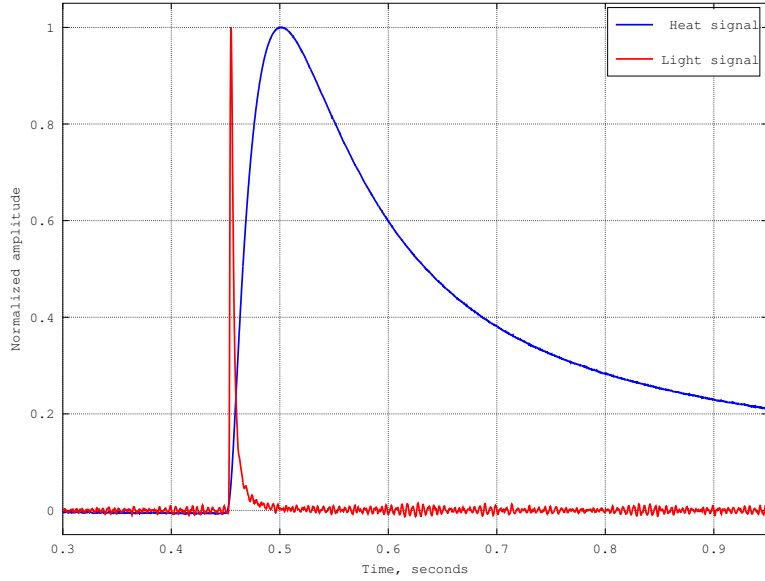
FIGURE 3.5: Typical signals from two bolometers in coincidence: in red is the signal from a light detector, in blue is the signal from crystal absorber.
