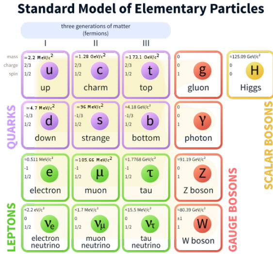
FIGURE 1.1: The schematic view of matter structure in Standard Model of elementary particles. The three generations of matter are shown in first three columns, gauge bosons in the fourth column, and the Higgs boson in the fifth. Figure taken from [24].
