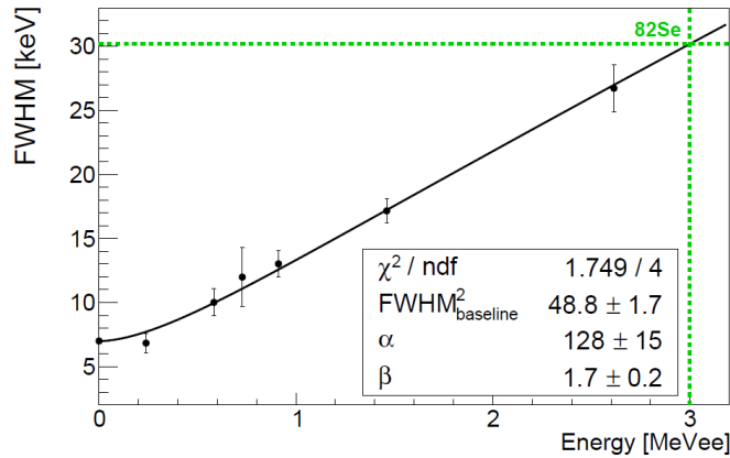
FIGURE 6.3: FWHM energy resolution as a function of the energy ( \text{Zn}^{82}\text{Se-1} ) for the most intense peaks produced by ^{228}\text{Th} and ^{40}\text{K} sources. The green dotted lines indicate the ^{82}\text{Se} Q-value.
