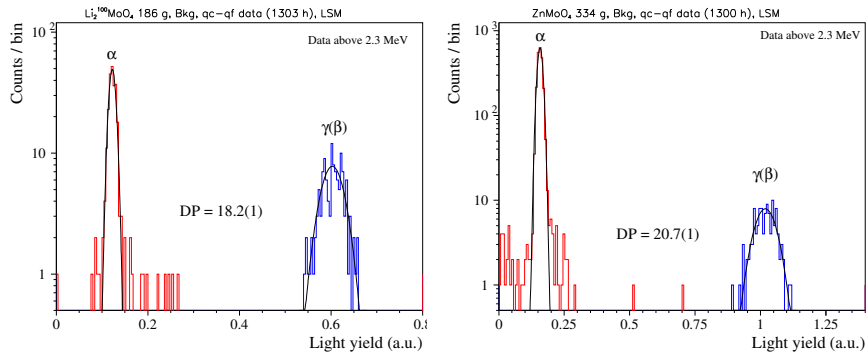
FIGURE 4.15: Q-plots of background measurements, collected over more than 1300 h for \text{Li}_2^{100}\text{MoO}_4 (left) and \text{ZnMoO}_4 (right).
