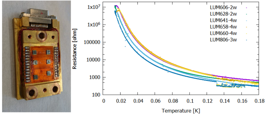
FIGURE 7.1: The holder for sensors test with 6 NTDs, attached using vacuum grease (left), and the R(T) characterization (right).
