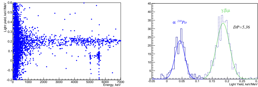
FIGURE 7.13: On the left:the scatter plot with 25 V bias applied on Neganov-Luke light detector. On the right:the discrimination between two particle types with 25 V bias on the grids, the \alpha (solid histogram) light amplitude(solid histogram) now can be separated from \gamma/\beta (dashed histogram), thanks to an increased sensitivity of the light read-out.
