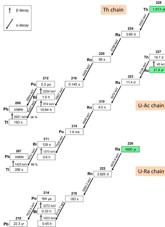
FIGURE 2.5: The three natural decay chains. Energies, half-lives and branching ratios are given.
