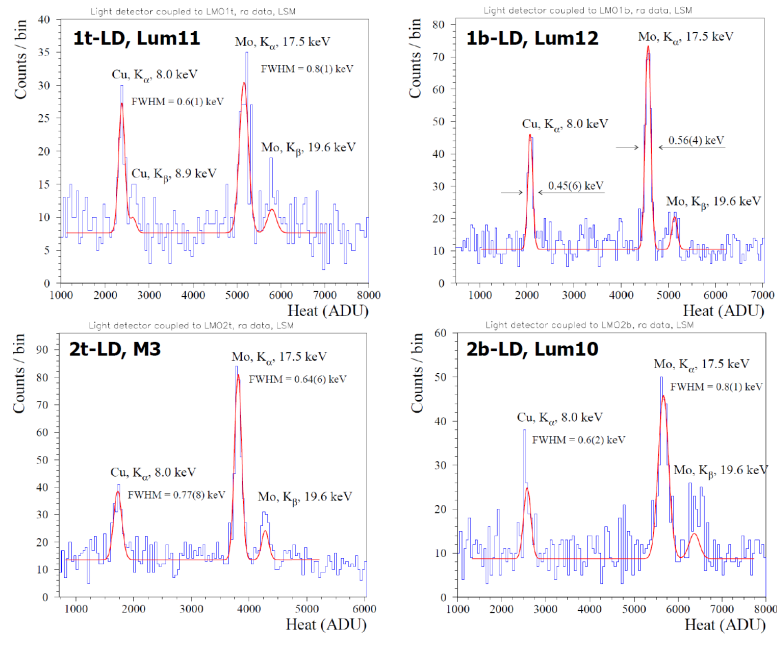
FIGURE 4.26: Spectrum of four light detectors, acquired during the ^{60}\text{Co} calibration at 17 mK.
