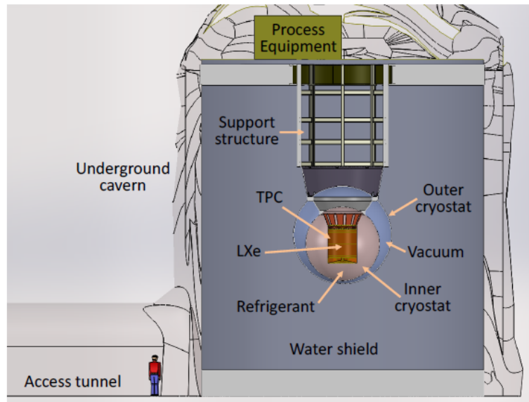
FIGURE 2.15: Engineering design rendering of the nEXO experiment concept
