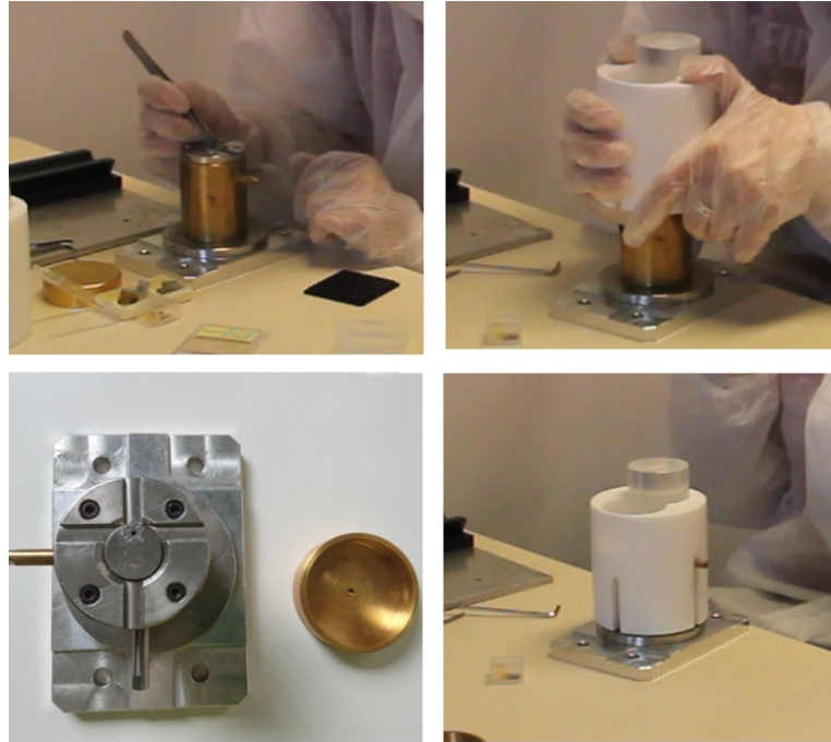
FIGURE 5.10: The tool for gluing (left bottom) together with the cap to provide 50 \mu\text{m} gap. On three other photos is shown the process of gluing: NTD placement (top left) and placing of the crystal (right).
