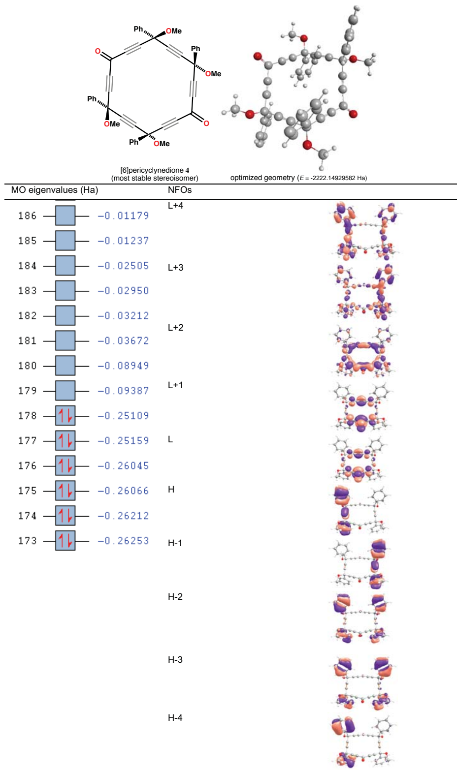
Figure S8. FMOs of the most stable stereoisomer of the carbo -[6]pericyclynedione 4 (B3PW91-6-31G(d,p) level).
