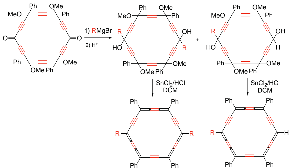
Scheme 1. The synthetic route based on a [6]pericyclonydione for preparation of dialkyl- and monoalkyl- carbo -benzenes by using \text{RMgBr} as a base.
