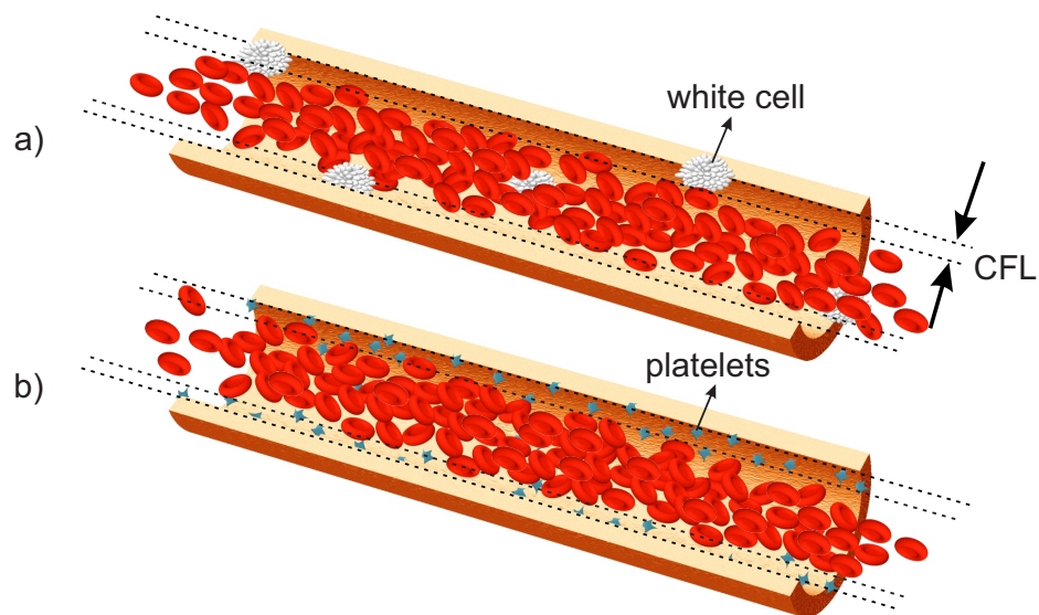
Fig. 11: Representation of the CFL and margination of a) white cells and b) platelets due to migration of red blood cells to the center of blood vessels.
