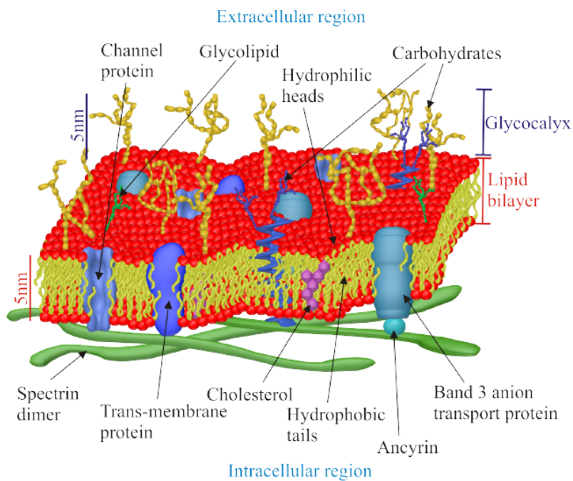
Fig. 5: Schematic drawing of RBC's lipid bilayer membrane, its components and the spectrin network/cytoskeleton attached to it intracellular face [1].
