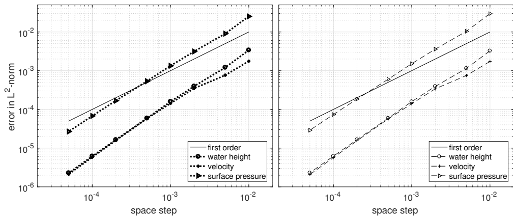
a) L^2 -errors with \lambda^2 = \delta_x
