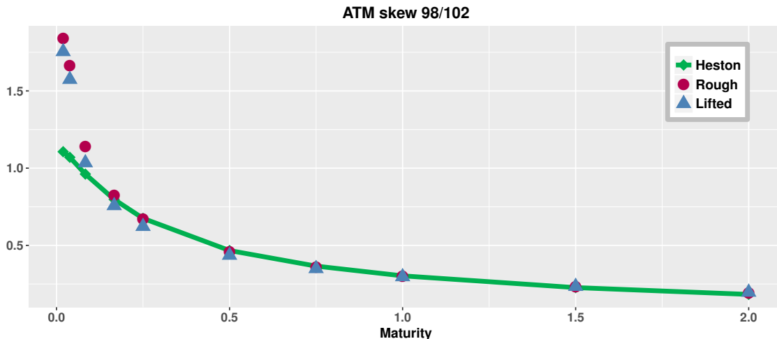
FIGURE 8.5: Term structure of the at-the-money skew of the rough Heston model \sigma_\infty(K, T; \Theta_0) of (8.3.6) (red circles), the calibrated lifted Heston model \sigma_{20}(K, T; r_{20} = 2.5, \Theta_0) of Table 8.4 (blue triangles) and the calibrated Heston model of Table 8.6 (green line).
