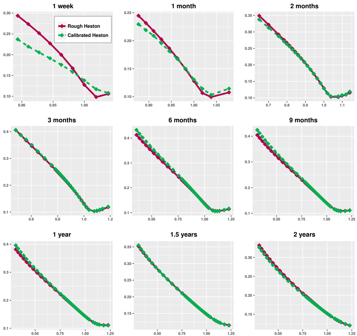
FIGURE 8.11: Implied volatility surface of the rough Heston model \sigma_\infty(K, T; \Theta_0) (red) and the calibrated Heston model of Table 8.6 (green) for maturities ranging from 1 week to 2 years (MSE = 2.06e-03).
