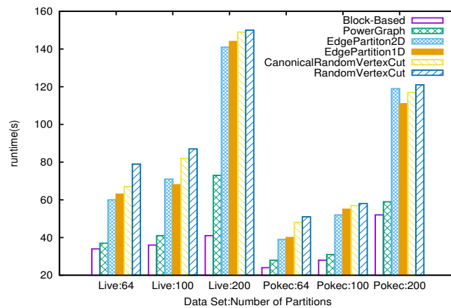
Fig. 3.8 Runtimes for Connected Components(CCs) computation with different partitionings for LiverJournal and Pocec
