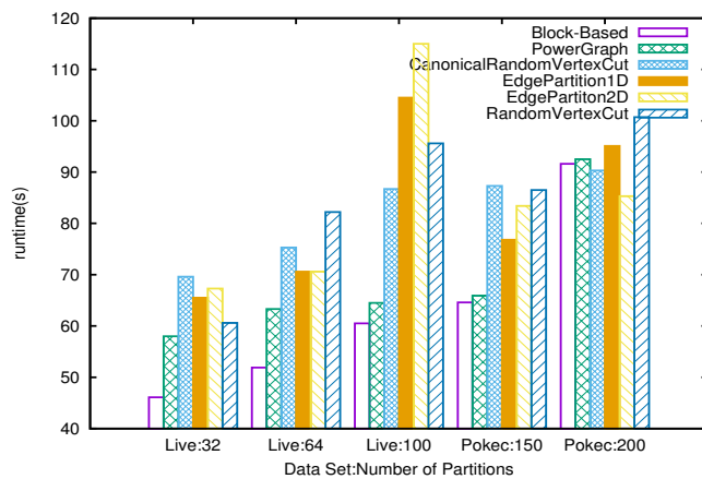
Fig. 3.10 Runtimes for Shortest Paths(SP) computation with different partitionings for LiveJournal and Pokec
