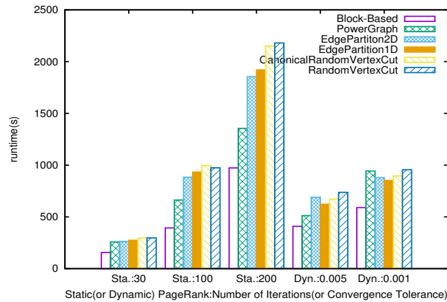
Fig. 3.7 Runtimes for static and dynamic PageRank for Pocec
