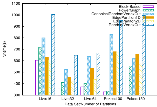
Fig. 3.9 Runtimes for Strongly Connected Components(SCC) computation with different partitionings for LiveJournal and Pokec
