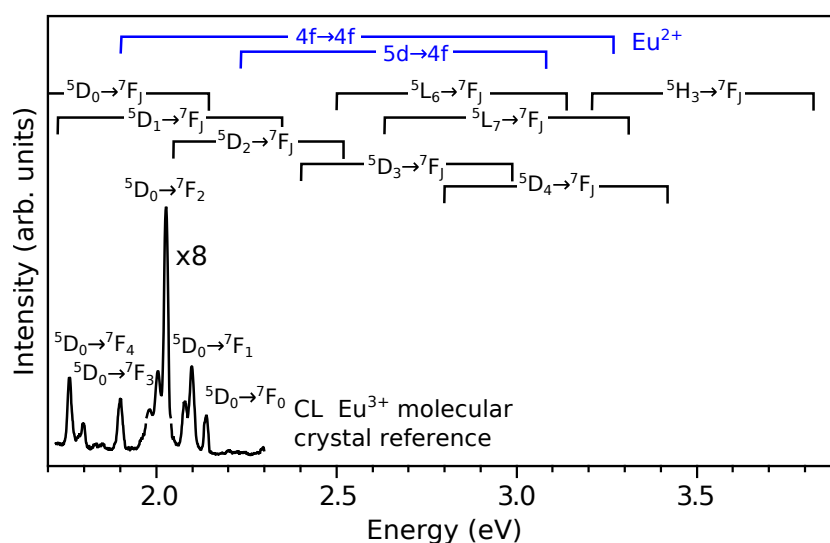
Figure 4.16: CL spectrum of Eu-complexes molecular crystal acquired in the STEM, with energy ranges of higher energy electron transitions in \text{Eu}^{3+} , from the calculated values reported in ref. [493], and most of them experimentally observed in complexes and doped crystals [493, 518, 519]. In blue, experimental ranges of \text{Eu}^{2+} sharp and broad transitions, from refs. [498–502, 504, 505] are also reported.
