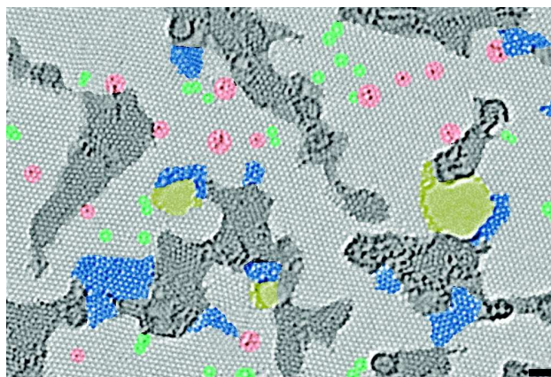
Figure 3.14: RGO obtained by hydrogen plasma treatment. Contaminated regions are shaded in dark gray, desordered regions in blue, individual ad-atoms or substitutions in red, isolated defects in green and holes in yellow. The scale bar is 1 nm [26].
