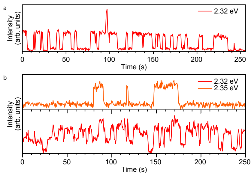
Figure 4.12: Emission from defects at 2.32 (red) and 2.35 (orange): intensity oscillation as a function of continuous illumination. Series of spectra acquired from areas about 30 nm (a) and 160 nm (b) wide.
