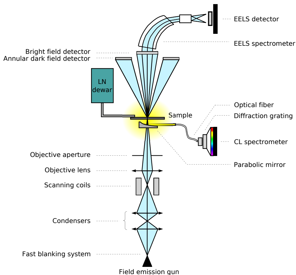
Figure 2.2: STEM microscope equipped with a liquid nitrogen system at the sample stage (LN dewar) and detection systems for EELS and CL spectroscopy. Collection and convergence angles are exaggerated for clarity. Real values are in the order of 10 mrad.
