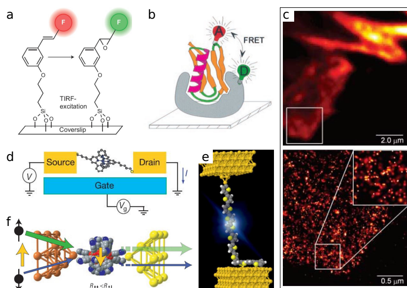
Figure 4.2: Some applications of single molecules. (a) Example of nanoreporter activity of a single molecule during a chemical reaction [329] and (b) of a pair of molecules (donor D and acceptor A , for investigation by FRET) during a biological process. (c) Comparison between (upper panel) an image obtained by total internal reflection fluorescence and (lower panel) PALM image corresponding to the area in the white square. (d-f) Schematics of single-molecule optoelectronic and spintronic devices: (d) a transistor [330], (e) a light emitting junction [331] and (f) a spin-valve favoring the flow of minority spin-down electrons [332].
