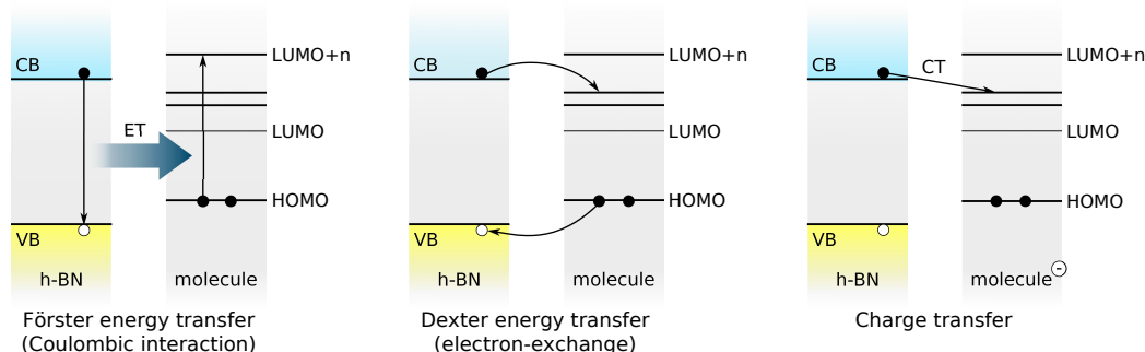
Figure 4.21: Possible mechanisms for the excitation transfer. For simplicity, excitonic and defect levels h-BN, vibrational levels associated to molecular electronic levels are not represented.
