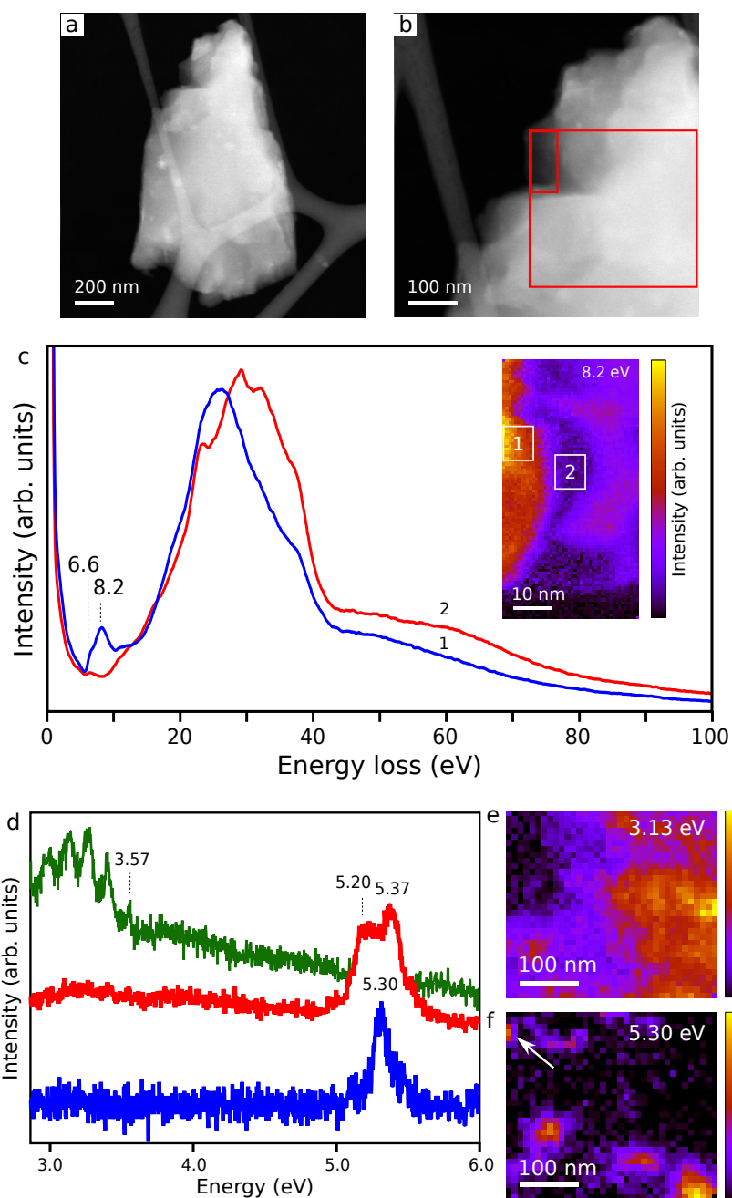
Figure 5.15: Thermally treated c -BN crystals. (a,b) HAADF images, where the regions investigated by hyperspectral imaging are indicated by the red rectangles. (c) Results from hyperspectral imaging: two spectra extracted from areas indicated by the white square in the intensity map. The map colour scale represents the intensity of the 8.2 eV feature. (d) Few CL spectra and (e-f) associated intensity maps.
