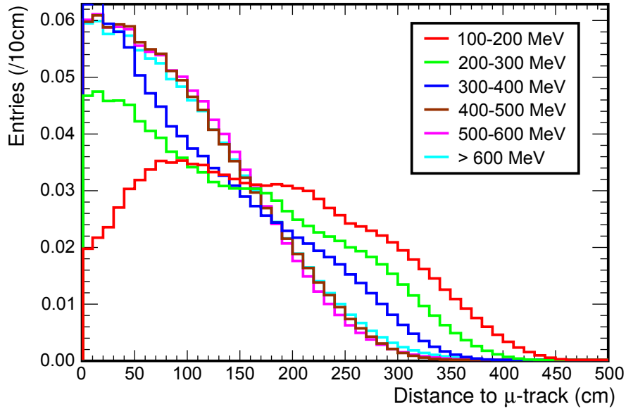
Figure 10.2 – Envelope functions for different FDI \mu energies (see labels), obtained from uncorrelated prompt - \mu pairs in the H analysis. Curves from [141].
