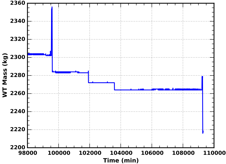
Figure 11.13 – Measured mass of the weighing tank during the filling of the chimney and the expansion tank. Partly compensating drifts can be observed whilst no liquid is being poured.
