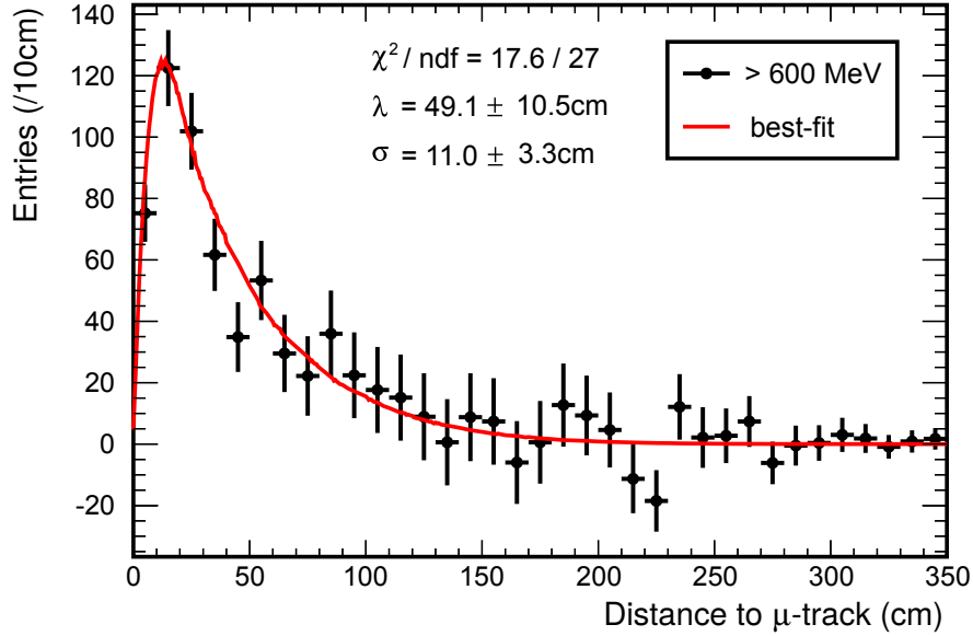
Figure 10.3 – Cosmogenic distance distribution for the FDI H \mu sample with the highest energy (black) and best matching prediction (red). Curves from [141].
