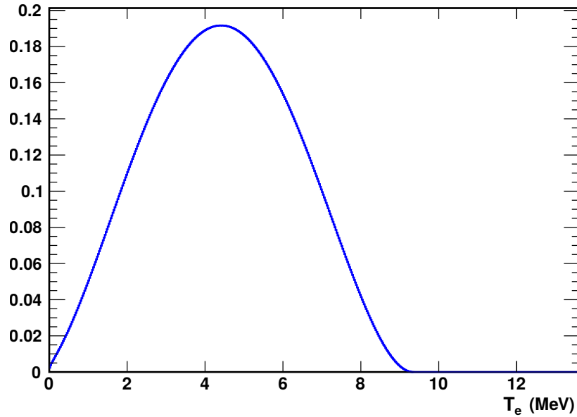
Figure 7.3 – Distribution of the kinetic energy of an electron in the \beta -decay of the {}^9\text{Li} ground state to the 2.78 MeV level in {}^9\text{Be} . The distribution was obtained by slicing the y-axis of the two-dimensional histogram presented in Figure 7.2 at Q_\beta = 9.342 MeV.
