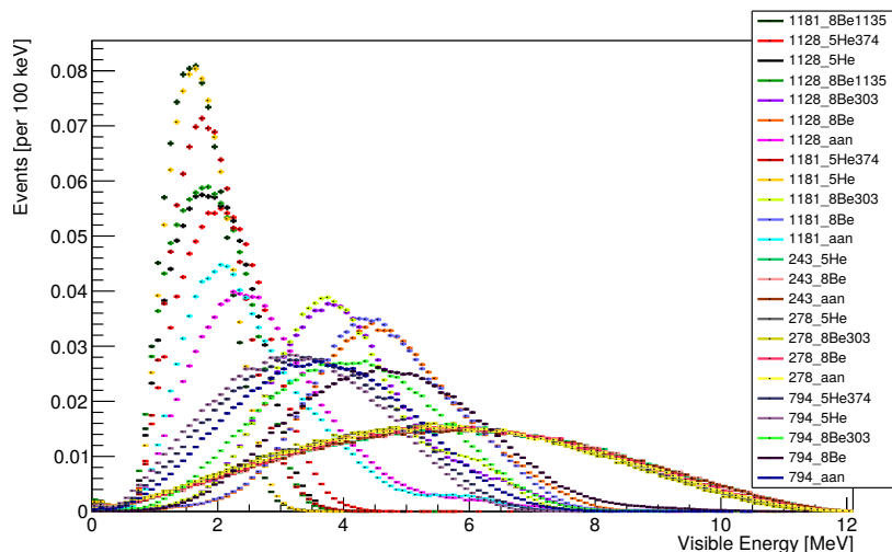
Figure 3 – Branches du {}^9\text{Li} .
