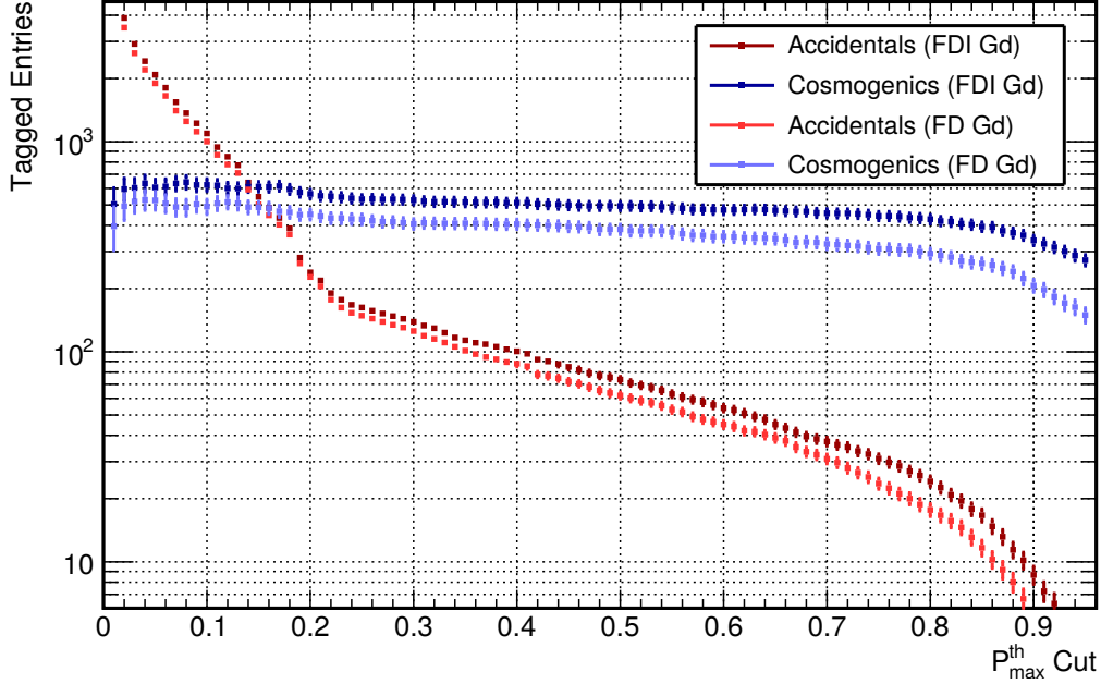
Figure 9.9 – Number of cosmogenics and accidentals tagged by the cosmogenic veto at FDI (dark colours) and FDII=FD (light colours), for the Neutrino Gd data set.
