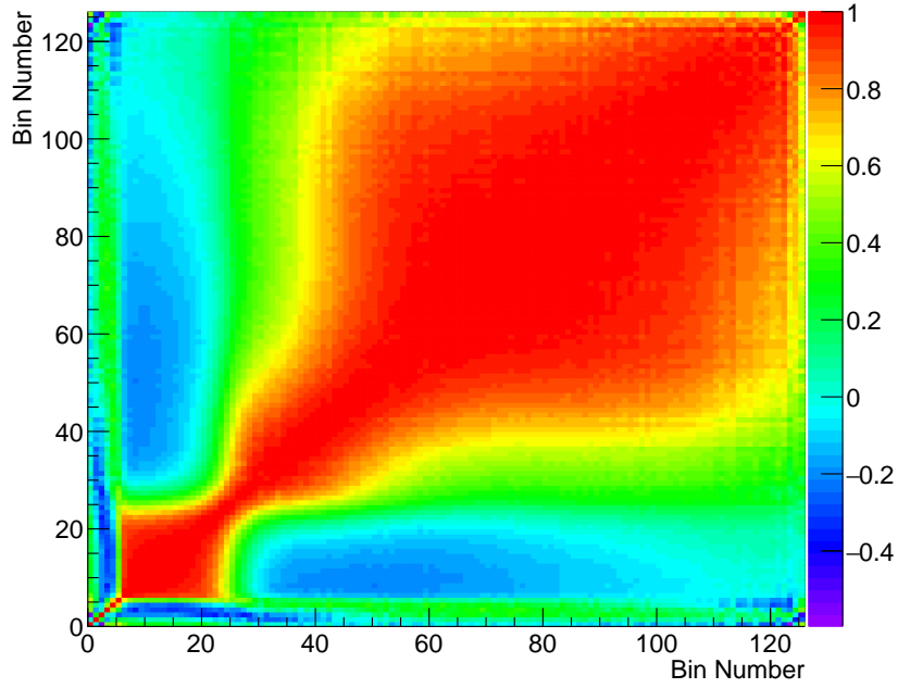
Figure 4 – Matrice de corrélations du spectre du {}^9\text{Li} .
