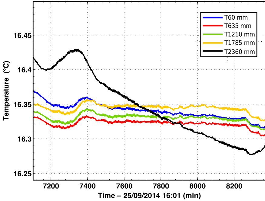
Figure 11.4 – Temperature evolution of the target sensors during the thermalisation stage. The labels of the sensors carry their position in the target along the upwards z -axis, whose origin is located at the bottom of the target. The sensor at z = 2360 mm behaves as if a little outside the liquid.
