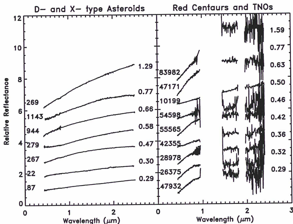
Figure 8.9: Comparison of D- and X-type asteroid spectra with Centaur and TNO spectra with the highest slopes. The object number is labeled on the left, and the overall visible and near-infrared slope is labeled on the right. In general, the TNOs have much steeper visible slopes, but flatten out in the near-infrared.
