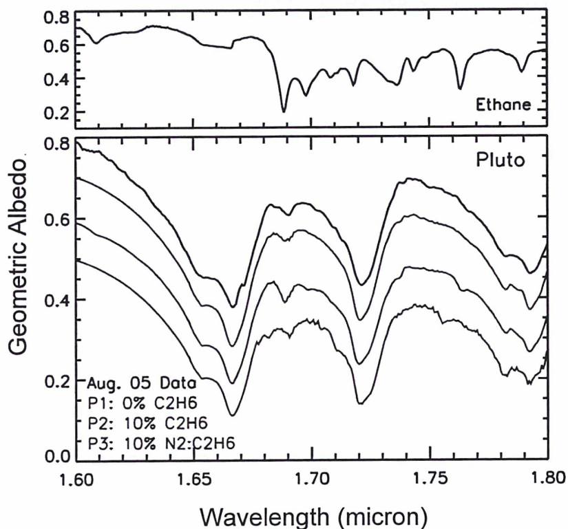
Figure 7.7: Pluto: Models (red) compared to the smoothed August, 2005 Pluto spectrum (black) as in Fig. 7.6 with an enlarged view from 1.6 - 1.8 \mu\text{m} . From top to bottom it shows the data from August, 2005, the model without ethane, with 10% pure ethane, and with 10% ethane diluted in nitrogen. We see here that ethane can be added to the model without increasing significantly the band near 1.69 \mu\text{m} if the amount of pure methane is reduced slightly. The band, however, is slightly shifted to shorter wavelengths than the data. The spectra are shifted by -0.1, 0.0, +0.1, and +0.2, for clarity. For comparison, at the top of this figure (and the next figure) we include a synthetic spectrum of 100% pure ethane created from optical constants from Quirico and Schmitt (1997b) with a grain size of 100 \mu\text{m} .
