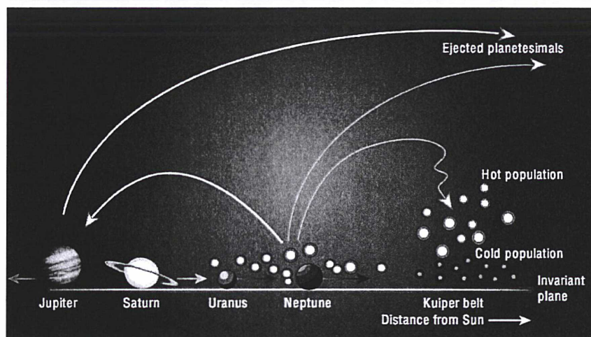
Figure 1.7: In the model by Gomes (2003b), as Jupiter moved inward and the three other giant planets moved outward, most small bodies in the region were ejected from the Solar System. Some bodies that were scattered by Neptune, however, were excited into orbits that are expected to now make up the “hot” population. (Source: Morbidelli and Levison, 2003)
