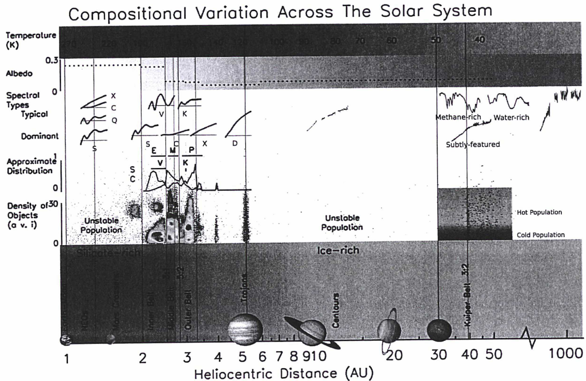
Figure 8.10: This cartoon summarizes and simplifies the distribution of material across the Solar System. The planets are pictured at the bottom and the location of different small body populations are labeled. The bottom panel shows the gradient from the predominantly “silicate-rich” material (brown) toward the predominantly “ice-rich” material (blue). The ice line is labeled at 2.7 AU, which is believed to be the approximate location past which water ice is stable, although this is a rough location and is debatable (Kennedy and Kenyon, 2008). The next panel shows the density of small bodies as a function of heliocentric distance plotted as semi-major axis versus inclination with color showing the density of bodies (red indicates highest density). In the classical Kuiper Belt region, the approximate hot and cold populations are indicated (cold population has i < 5^\circ ). The approximate distribution of taxonomic type is displayed for the inner Solar System in the next panel. The lines mark the distribution of certain taxonomic types according to their frequency among SDSS colors, we show the frequency of S and C-types, and the generally location of a few other types. The general locations of less prominent spectral types are also marked. Above that is a model spectrum of the dominant spectral type per region and then the typical spectral types per region which are present, but not the most frequent. The gray bar shows the average albedo. In the inner Solar System the albedo marked is the average for the dominant spectral type from the sample from DeMeo et al. (2009a). The Trojan albedo is from Fernández et al. (2003), and the Centaur and TNO albedos are averages from the data presented in Stansberry et al. (2008), however, only objects NOT dominated by water and other volatiles were included (Orcus, Quaoar, dwarf planets, etc. were excluded). The top panel displays the approximate effective temperature based on a black body calculation as a function of distance from the Sun with an assumed albedo of 0.1.
