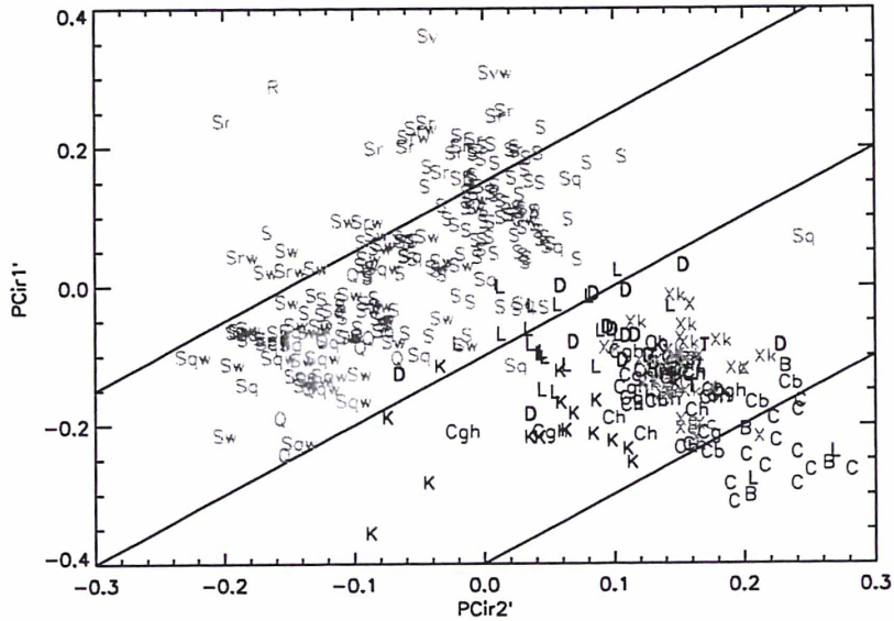
Figure 4.15: Plot of PCir1' v. PCir2'. Here we create four segments separated by the three lines to help determine to which class an object belongs. Without the visible information, we cannot determine definite class boundaries in many cases.
