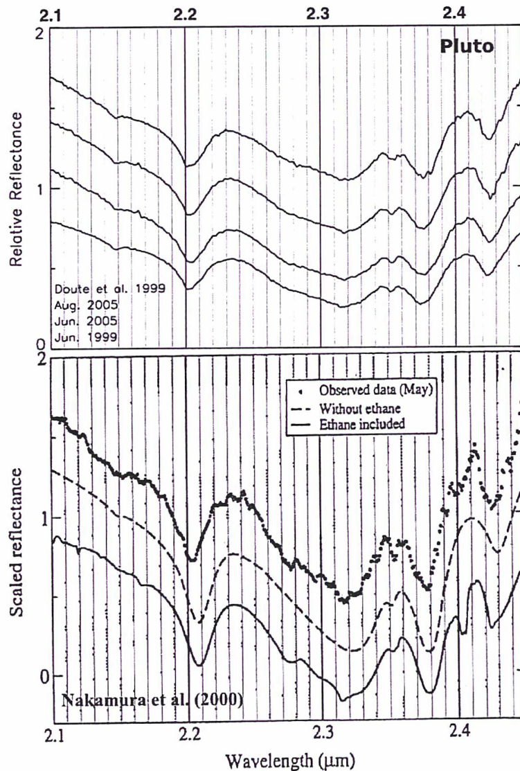
Figure 7.12: Pluto: Comparison of spectra of Pluto from Nakamura et al. (2000) taken on May 6, 1999 with Doute et al. (1999) and this work. The bottom half of the figure is taken from Nakamura et al. (2000), and shows, from top to bottom, the data, a model without ethane, and a model with pure ethane. The top half of the figure shows, from top to bottom, the spectrum from Doute et al. (1999), and our data (smoothed in this case) from August, 2005, June, 2005, and June, 1999. The feature at 2.4 \mu\text{m} is much more subtle in the spectra from this work compared to the Nakamura spectrum. The spectrum from June, 1999 was taken one month after the Nakamura spectrum at the same location on Pluto's surface.
