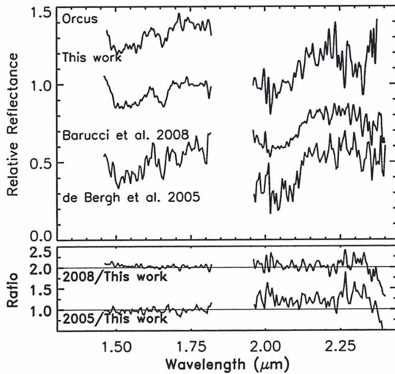
Figure 6.5: Top: The near-infrared spectra of Orcus from this and previous work. The data are from de Bergh et al. (2005), Barucci et al. (2008b), and this work from bottom to top. The spectra are normalized to 1 at 1.75 \mu\text{m} , a fairly flat region of the spectrum, and are shifted vertically by 0.4 for clarity. Bottom: The ratio of these previously published spectra to this work.
