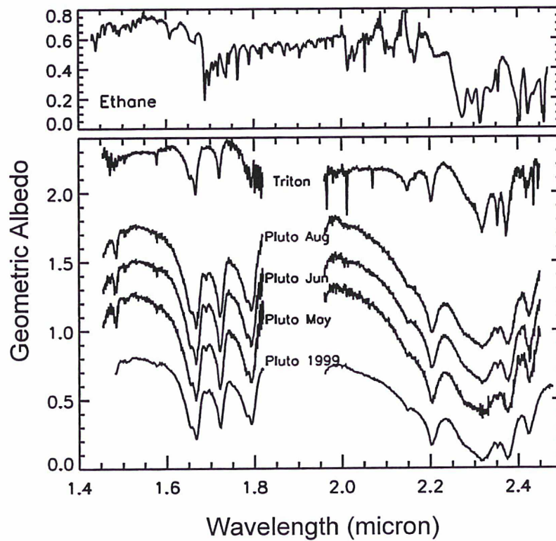
Figure 7.4: Spectra of Triton from Nov. 2008, and Pluto from Aug., Jun., and May, 2005 and Jun. 1999. The June, 1999 spectrum has overall flux differences from the 2005 spectra, likely due to the >10\% error in flux in that data. The spectra are shifted vertically by -0.2 , +0.25 , +0.5 , and +0.75 from bottom to top, and are normalized to unity at 1.55 microns. The top portion of the figure displays a synthetic spectrum of ethane to compare band locations with the data.
