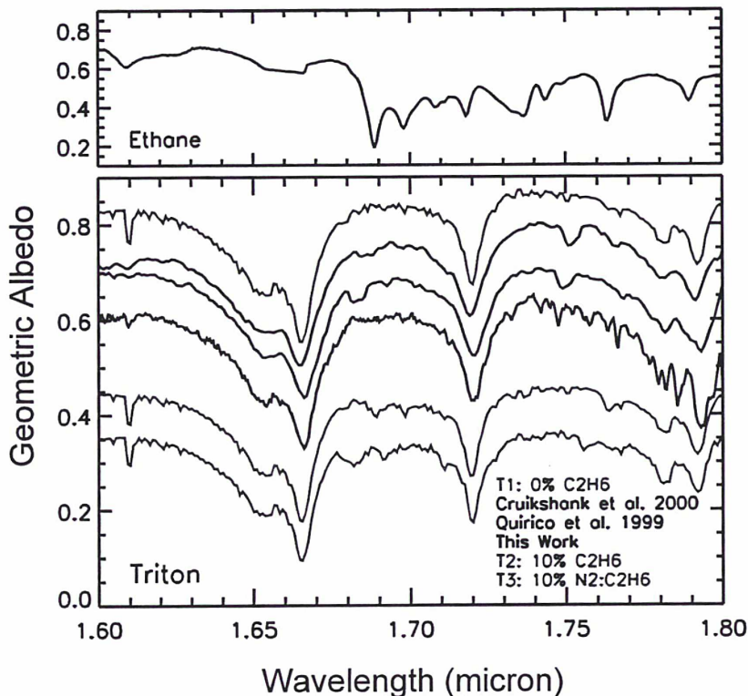
Figure 7.10: Triton: Models (red) compared to spectral data (black) of Triton. From top to bottom it shows the model without ethane, data from Cruikshank et al. (2000) (May, 1995), Quirico et al. (1999) (Sep., 1995), and this work (Nov., 2008), the model with 10% pure ethane, and the model with 10% diluted ethane in the 1.6-1.8- \mu\text{m} range. Interestingly, the features near 1.69 and 1.75 \mu\text{m} are not at the same position among the data. It is clear that these weak features do not match the models, however, laboratory data show that ethane bands can shift as much as 0.007 \mu\text{m} between the pure and diluted forms, which raises the possibility that other amounts of dilution could match the data. The spectra are shifted by -0.42, -0.32, -0.22, -0.12, -0.12, and 0.08 for clarity. For comparison, at the top of this figure (and the next figure) we include a synthetic spectrum of 100% pure ethane created from optical constants from Quirico and Schmitt (1997b) with a grain size of 100 \mu\text{m} .
