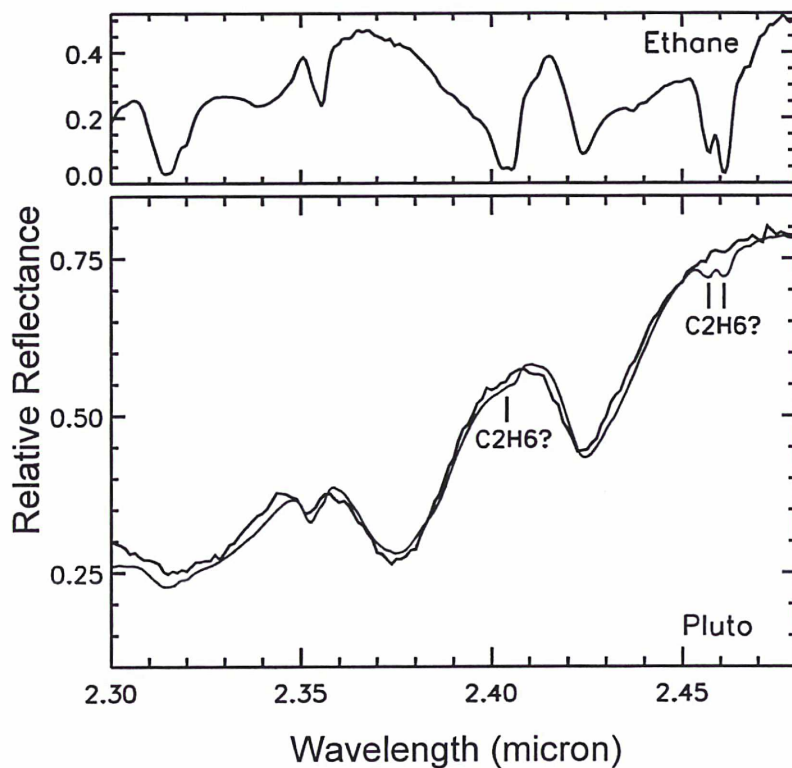
Figure 7.13: Pluto: Here we present the relative reflectance of the 1999 UKIRT spectrum plotted to longer wavelengths that were not measured by SINFONI. The data (black) is normalized to unity at 1.55 \mu\text{m} . A modified version of the model (red) of the August, 2005 spectrum including 10 % ethane is overlaid. Because of the flux issue with the 1999 data we scale and shift the model to generally match the methane bands. We thus cannot make any inferences about the albedo of the data versus the model, however, we can inspect the relative strengths of the ethane bands when 10 % is included in the model. A spectrum of pure ethane with 100 \mu\text{m} grains is included at the top of the figure as a reference. Two faint features (at 2.457 and 2.461 \mu\text{m} ) in the data are located at the same position of two strong features of ethane.
