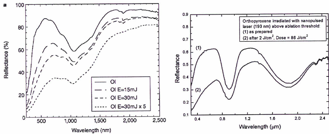
Figure 1.12: Laboratory experiments simulating space weathering through nanophase pulses. Left: Olivine before and after specified irradiation doses by Sasaki et al. (2001). After irradiation the reflectance in the visible regime is significantly decreased causing an apparent reddening of the spectrum and decrease in absorption. Right: Orthopyroxene before and after irradiation by Brunetto et al. (2006b). As for olivine the reflectance at shorter wavelengths is decreased at shorter wavelengths although the effect is not as pronounced for pyroxene as for olivine.
