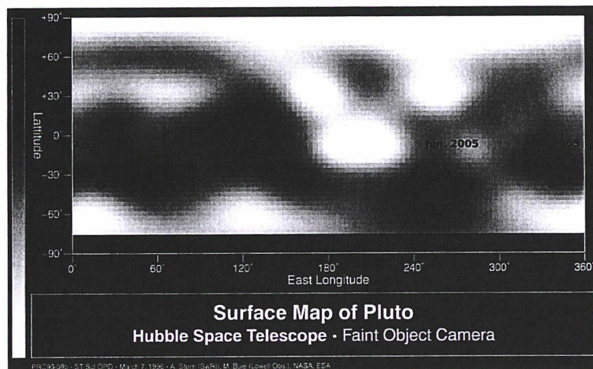
Figure 7.3: The dark circles mark the central longitude and latitude on Pluto’s surface for each observation. The figure is shown in a similar format to that in Olkin et al. (2007), with the albedo map from Stern et al. (1997). The rotational north pole is +90 degrees latitude, and longitudes are plotted as 360 minus the IAU definition values reported elsewhere in this article. The longitudes plotted here are 21, 80, 267, and 340 degrees, from left to right.
