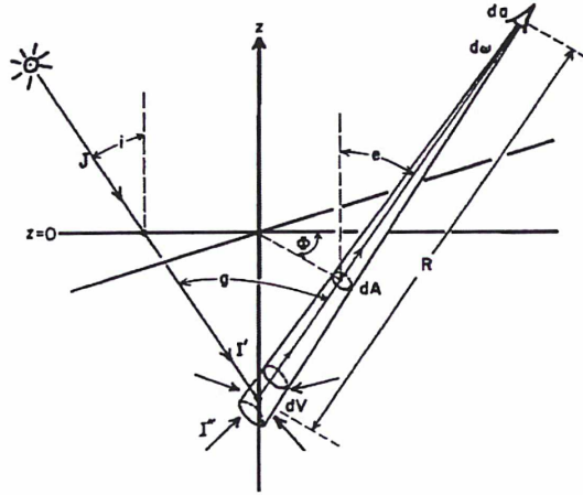
Figure 3.4: This is a diagram of Hapke geometry from Hapke (1981). The incident light J makes an angle i with the z -axis, and the reflected light makes an angle e with the z -axis. The detector has an area da and receives light within the solid angle d\omega .
