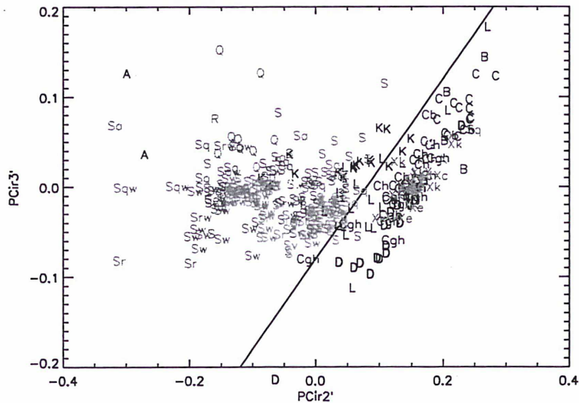
Figure 4.14: Plot of PCir2' v. PCir3'. Here “featured” versus “subtly featured” objects are separated by the line.
