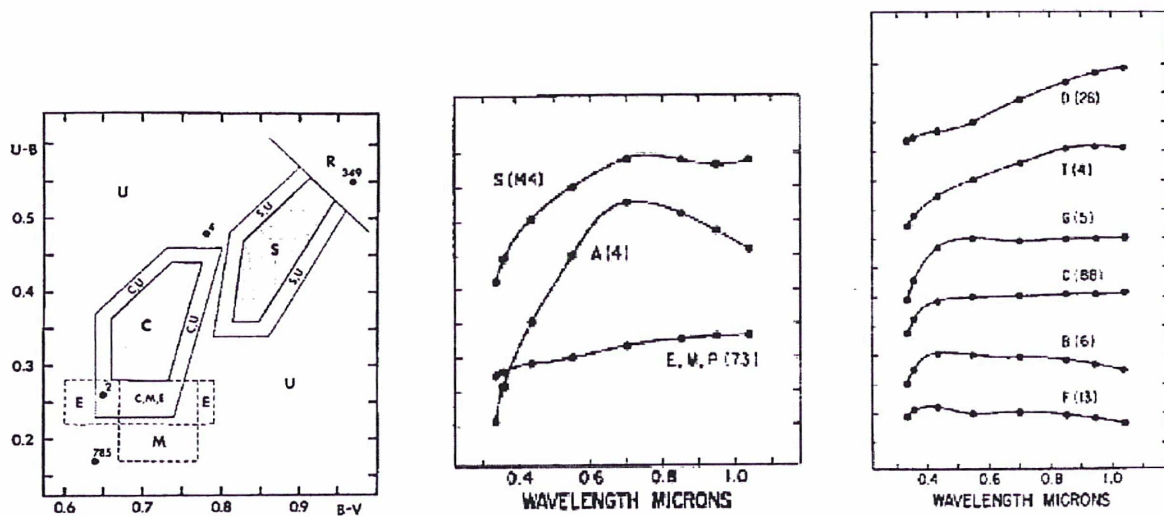
Figure 4.1: Left: Separation of classes in Bowell Taxonomy using U-B and B-V colors Bowell et al. (1978). Middle and Right: Example spectra for each class in the Tholen taxonomy (Zellner et al., 1985; Tholen, 1984)
