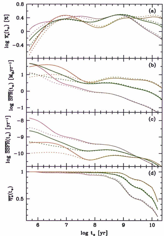
Figure 12. Comparison between mean SFHs for the SF hq sample modelled with only one stellar extinction (dotted lines) and with differential extinction (solid lines). For clarity, only Z_{\text{neb}} bins B, D and F are drawn, and colour-coding is the same as in Fig. 2. Each panel shows a different representation of SFHs: (a) smoothed population vector, \bar{x}_*(t_*) , (b) \text{SFR}(t_*) , (c) \text{SSFR}(t_*) and (d) \bar{t}_*(t_*) .
