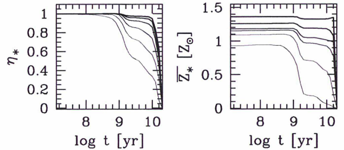
Figure 1. Histories of our parent sample in stellar mass bins. Thicker lines are used for more massive bins. Panels show the median curve for time evolution of stellar mass evolution (left; see equation 1) and metallicity evolution (right).
