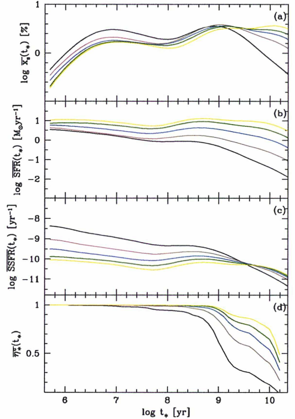
Figure 10. As Fig. 8, but binning SF galaxies by their stellar surface densities, with five 0.5 dex wide bins centred at \log \Sigma_\star = 7.25, 7.75, 8.25, 8.75 and 9.25 M_\odot \text{ kpc}^{-2} , containing 1477, 12 554, 37 177, 27 742, 3046 galaxies, respectively.
