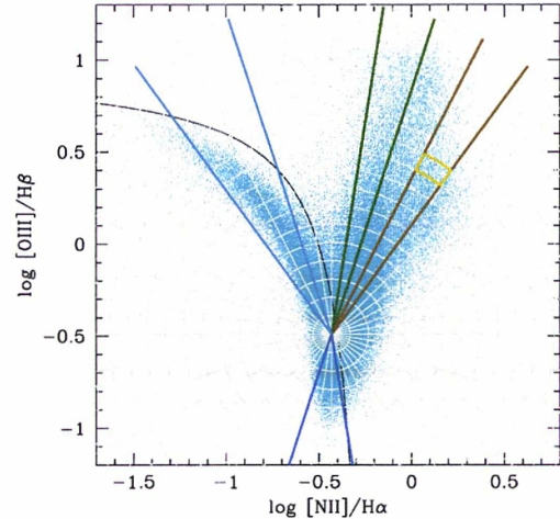
Figure 1. The chopped seagull and the definition of the SF branches (light blue and dark blue), Seyfert branch (green) and LINER branch (red). The data points represent all the galaxies defined in Section 2.1 that have S/N > 3 in the four lines involved in the plot (131 287 objects). The black curve is the upper envelope of pure SF galaxies according to Stasińska et al. (2006).
