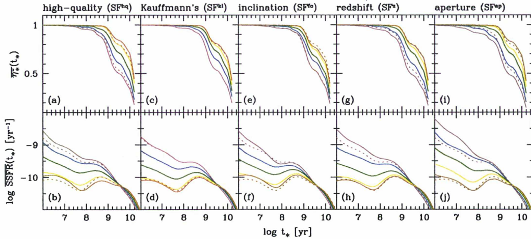
Figure 11. Average mass assembly histories ( \eta_*^c , top panels) and specific SFR (SSFR, bottom) histories for Z_{\text{neb}} bins B to F, colour-coded as in Fig. 2. Solid lines show the curves for different sample definitions. For comparison, the dotted lines in all panels show the curves for bins B (lower curves; magenta) and F (upper curves; red) of the full SF sample.
